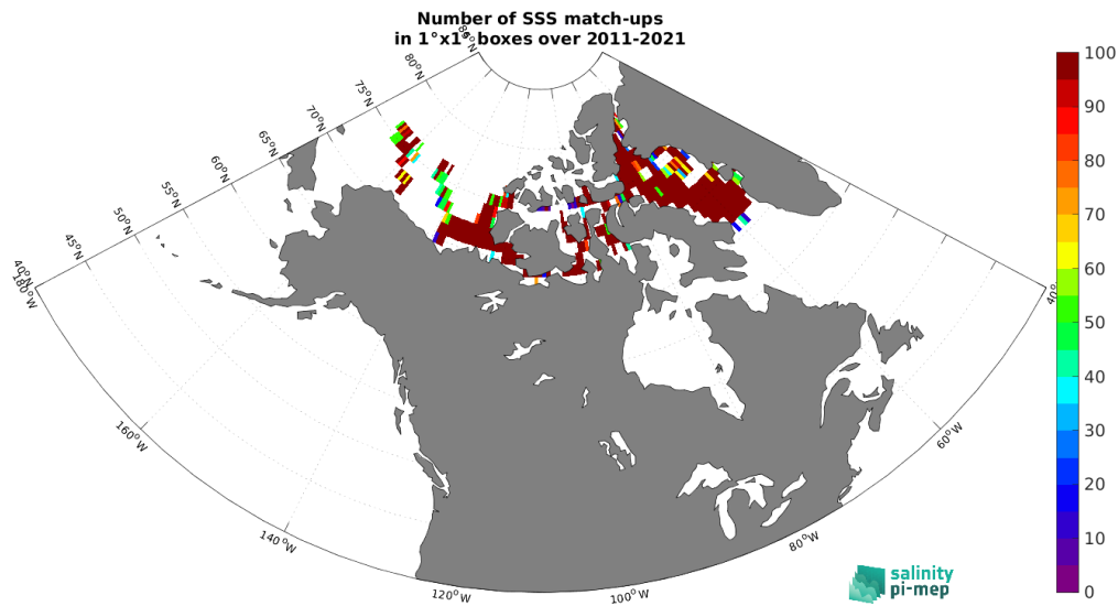
Figure 5: Number of SSS match-ups between TSG (Amundsen) SSS and the SMOS SSS L3 Arctic v4 - 9 Days (BEC) SSS product for the Arctic Ocean Pi-MEP region over 1^\circ \times 1^\circ boxes and for the full satellite product period.
