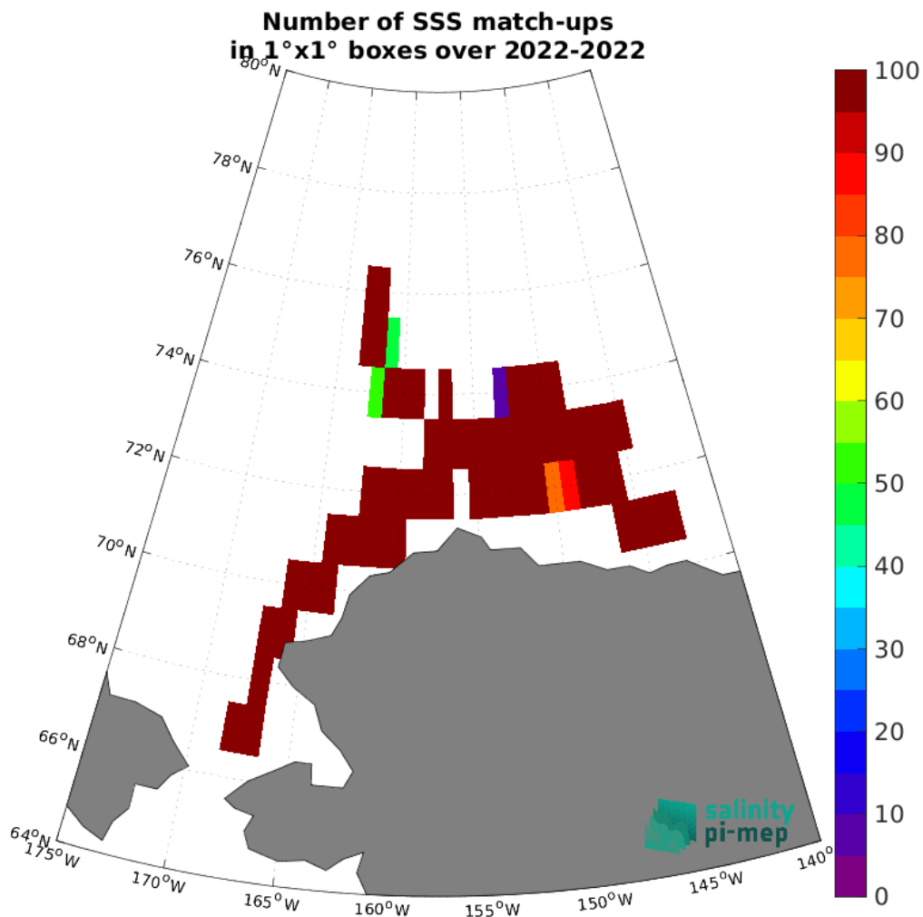
Figure 5: Number of SSS match-ups between SASSIE SSS and the SMOS SSS L3 Arctic v4 - 9 Days (BEC) SSS product for the Arctic Ocean Pi-MEP region over 1^\circ \times 1^\circ boxes and for the full satellite product period.
