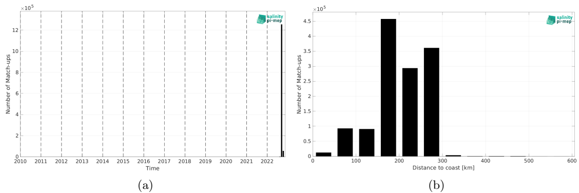
Figure 2: Number of match-ups between SASSIE and SMOS SSS L3 Arctic v4 - 9 Days (BEC) SSS as a function of time (a) and as function of the distance to coast (b) over the Arctic Ocean Pi-MEP region and for the full satellite product period.
