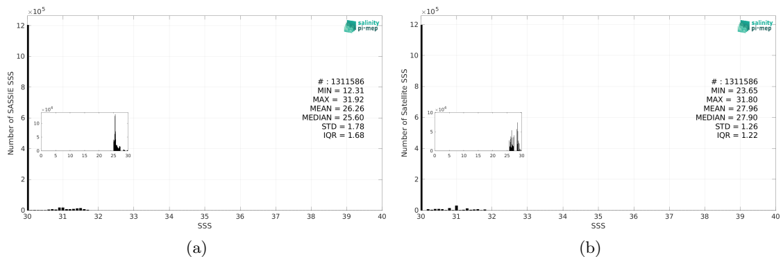
Figure 3: Histograms of SSS from SASSIE (a) and SMOS SSS L3 Arctic v4 - 9 Days (BEC) (b) considering all match-up pairs per bins of 0.1 over the Arctic Ocean Pi-MEP region and for the full satellite product period.
