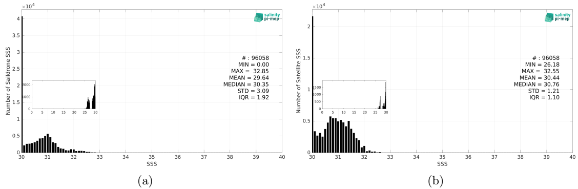
Figure 3: Histograms of SSS from Sairdrone (a) and SMOS SSS L3 Arctic v4 - 9 Days (BEC) (b) considering all match-up pairs per bins of 0.1 over the Arctic Ocean Pi-MEP region and for the full satellite product period.
