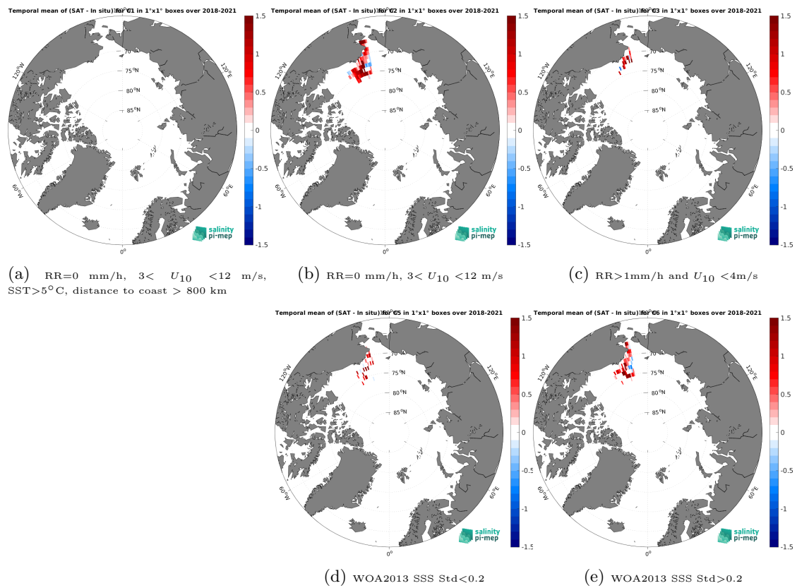
Figure 14: Temporal mean gridded over spatial boxes of size 1^\circ \times 1^\circ of \Delta SSS (SMOS SSS L3 Arctic v4 - 9 Days (BEC) - Saildrone) for 5 different subdatasets corresponding to:RR=0 mm/h, 3 < U_{10} < 12 m/s, SST>5°C, distance to coast > 800 km (a), RR=0 mm/h, 3 < U_{10} < 12 m/s (b), RR>1mm/h and U_{10} < 4 m/s (c), WOA2013 SSS Std<0.2 (d), WOA2013 SSS Std>0.2 (e).
