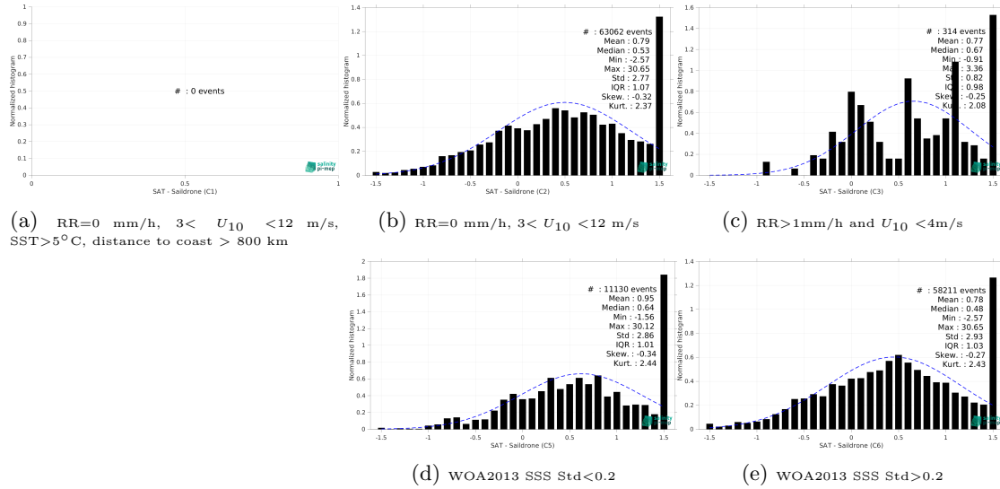
Figure 15: Normalized histogram of \Delta SSS (SMOS SSS L3 Arctic v4 - 9 Days (BEC) - Saildrone) for 5 different subdatasets corresponding to: RR=0 mm/h, 3 < U_{10} < 12 m/s, SST > 5°C, distance to coast > 800 km (a), RR=0 mm/h, 3 < U_{10} < 12 m/s (b), RR > 1mm/h and U_{10} < 4 m/s (c), WOA2013 SSS Std < 0.2 (d), WOA2013 SSS Std > 0.2 (e).
