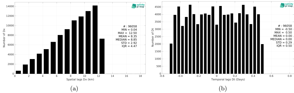
Figure 6: Histograms of the spatial (a) and temporal (b) lags between the location/time of the Sairdronne measurement and the date of the corresponding SMOS SSS L3 Arctic v4 - 9 Days (BEC) SSS pixel.
