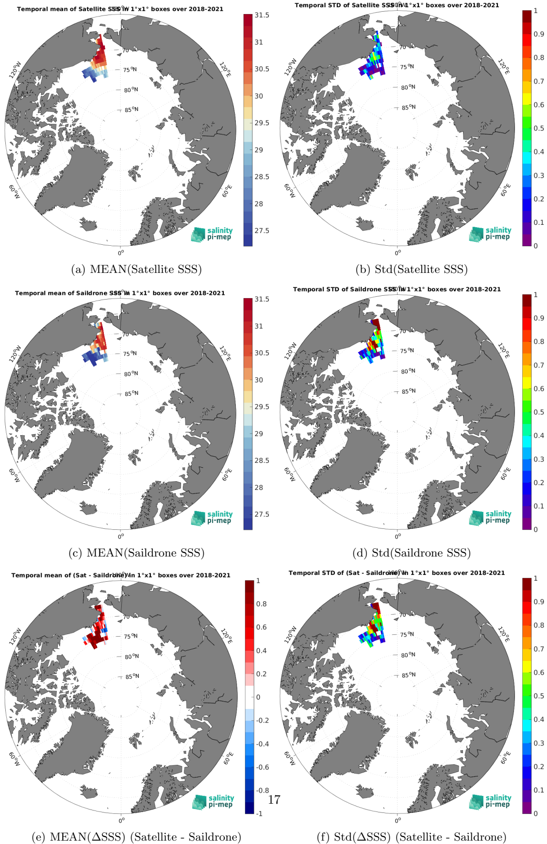
Figure 7: Temporal mean (left) and Std (right) of SSS from SMOS SSS L3 Arctic v4 - 9 Days (BEC) (top), Saildrone (middle), and of \Delta SSS (Satellite - Saildrone). Only match-up pairs are used to generate these maps.
