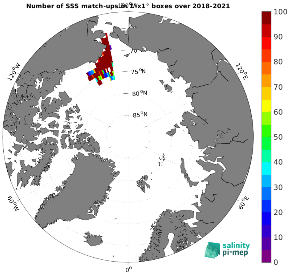
Figure 5: Number of SSS match-ups between Saildrone SSS and the SMOS SSS L3 Arctic v4 - 9 Days (BEC) SSS product for the Arctic Ocean Pi-MEP region over 1^\circ \times 1^\circ boxes and for the full satellite product period.
