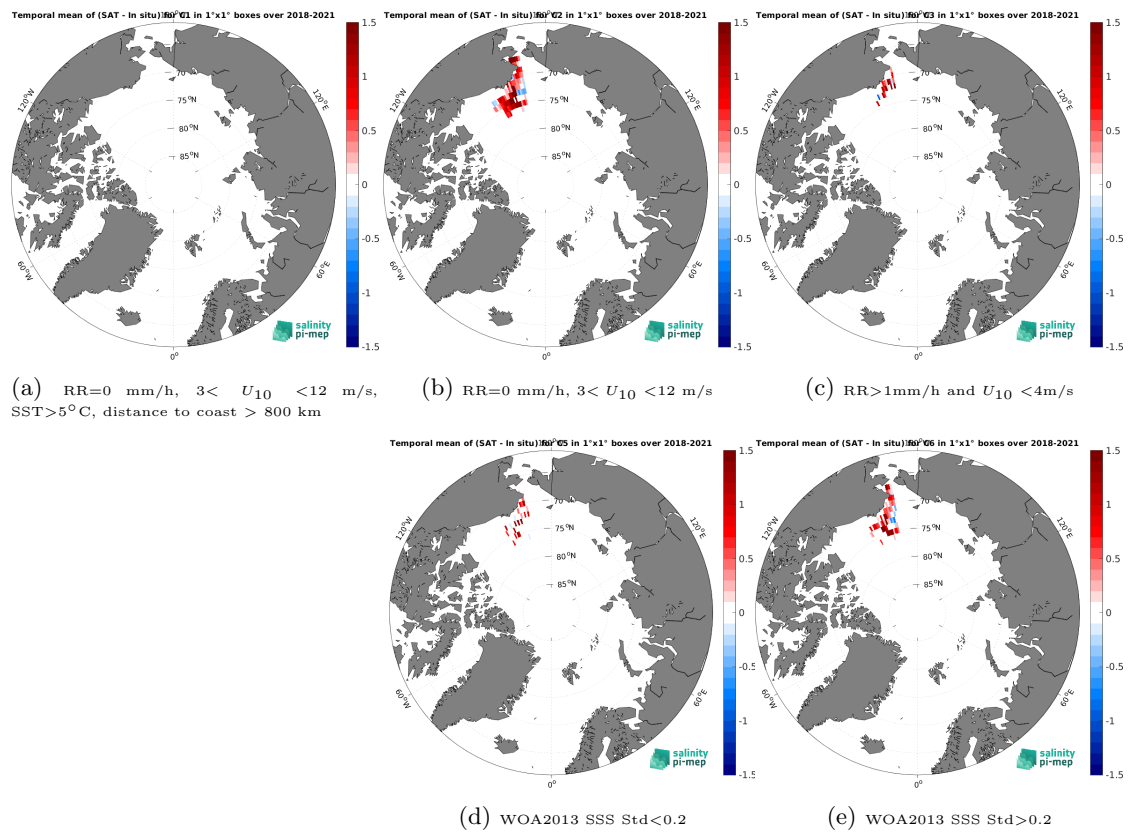
Figure 14: Temporal mean gridded over spatial boxes of size 1^\circ \times 1^\circ of \Delta\text{SSS} (SMOS SSS L3 Arctic v4 - 9 Days (BEC) - Saildrone) for 5 different subdatasets corresponding to:RR=0 mm/h, 3 < U_{10} < 12 m/s, SST>5°C, distance to coast > 800 km (a), RR=0 mm/h, 3 < U_{10} < 12 m/s (b), RR>1mm/h and U_{10} < 4 m/s (c), WOA2013 SSS Std<0.2 (d), WOA2013 SSS Std>0.2 (e).
