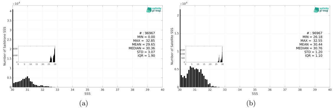
Figure 3: Histograms of SSS from Saildrone (a) and SMOS SSS L3 Arctic v4 - 9 Days (BEC) (b) considering all match-up pairs per bins of 0.1 over the Arctic Ocean Pi-MEP region and for the full satellite product period.
