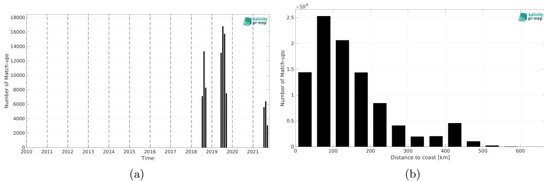
Figure 2: Number of match-ups between Saildrone and SMOS SSS L3 Arctic v4 - 9 Days (BEC) SSS as a function of time (a) and as function of the distance to coast (b) over the Arctic Ocean Pi-MEP region and for the full satellite product period.
