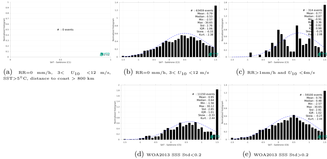
Figure 15: Normalized histogram of \Delta SSS (SMOS SSS L3 Arctic v4 - 9 Days (BEC) - Sairdronne) for 5 different subdatasets corresponding to: RR=0 mm/h, 3 < U_{10} < 12 m/s, SST > 5°C, distance to coast > 800 km (a), RR=0 mm/h, 3 < U_{10} < 12 m/s (b), RR > 1mm/h and U_{10} < 4 m/s (c), WOA2013 SSS Std < 0.2 (d), WOA2013 SSS Std > 0.2 (e).
