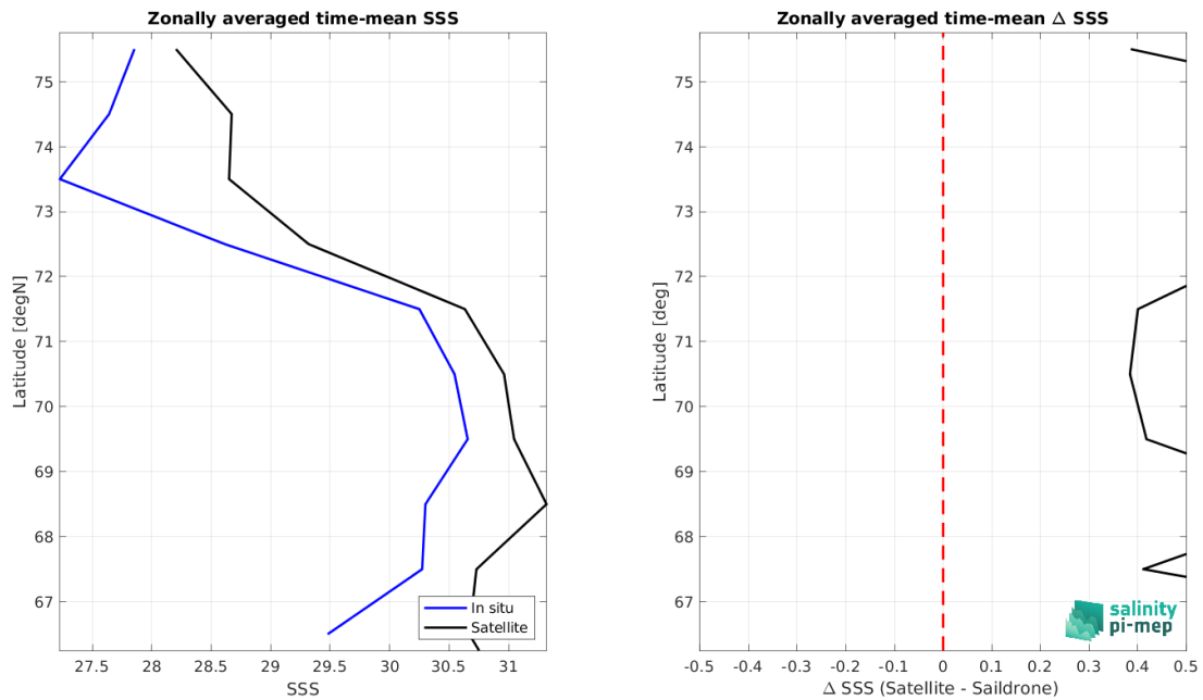
Figure 9: Left panel: Zonal mean SSS from SMOS SSS L3 Arctic v4 - 9 Days (BEC) satellite product (black) and from Saildrone (blue). Right panel: Zonal mean of \Delta SSS (Satellite - Saildrone) for all the collected Pi-MEP match-up pairs estimated over the full satellite product period.
