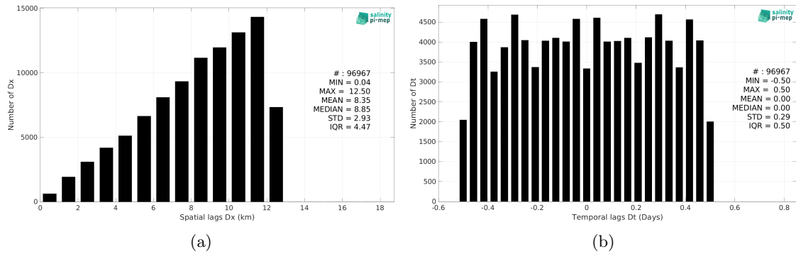
Figure 6: Histograms of the spatial (a) and temporal (b) lags between the location/time of the Saildrone measurement and the date of the corresponding SMOS SSS L3 Arctic v4 - 9 Days (BEC) SSS pixel.
