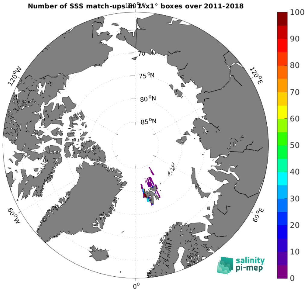
Figure 5: Number of SSS match-ups between Marine mammals SSS and the SMOS SSS L3 Arctic v4 - 9 Days (BEC) SSS product for the Arctic Ocean Pi-MEP region over 1^\circ \times 1^\circ boxes and for the full satellite product period.
