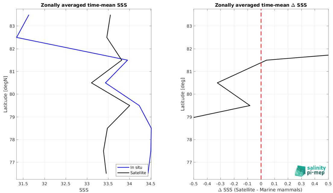
Figure 9: Left panel: Zonal mean SSS from SMOS SSS L3 Arctic v4 - 9 Days (BEC) satellite product (black) and from Marine mammals (blue). Right panel: Zonal mean of \Delta SSS (Satellite - Marine mammals) for all the collected Pi-MEP match-up pairs estimated over the full satellite product period.
