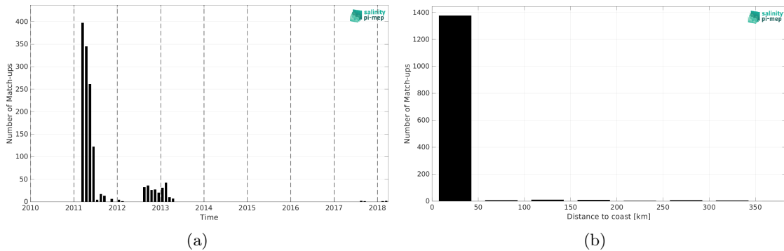
Figure 2: Number of match-ups between Marine mammals and SMOS SSS L3 Arctic v4 - 9 Days (BEC) SSS as a function of time (a) and as function of the distance to coast (b) over the Arctic Ocean Pi-MEP region and for the full satellite product period.
