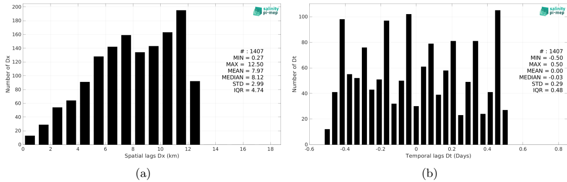
Figure 6: Histograms of the spatial (a) and temporal (b) lags between the location/time of the Marine mammals measurement and the date of the corresponding SMOS SSS L3 Arctic v4 - 9 Days (BEC) SSS pixel.
