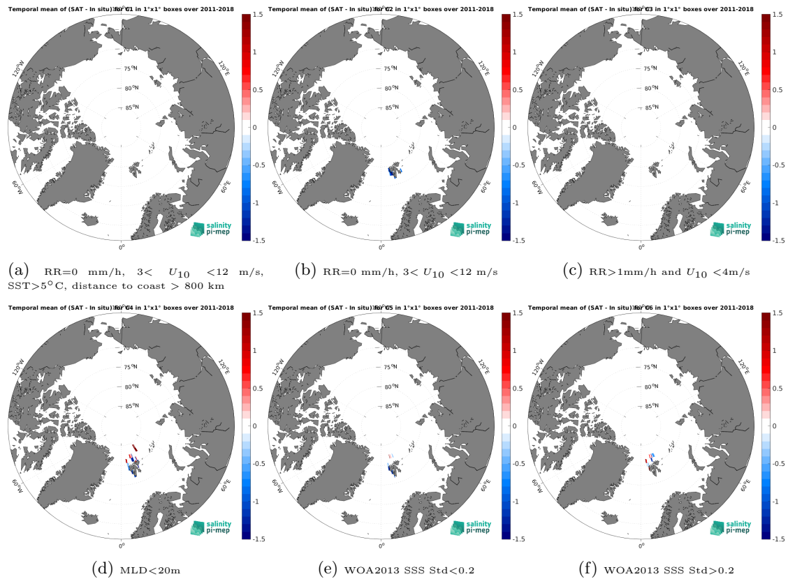
Figure 14: Temporal mean gridded over spatial boxes of size 1^\circ \times 1^\circ of \Delta SSS (SMOS SSS L3 Arctic v4 - 9 Days (BEC) - Marine mammals) for 6 different subdatasets corresponding to:RR=0 mm/h, 3 < U_{10} < 12 m/s, SST >5^\circ C, distance to coast > 800 km (a), RR=0 mm/h, 3 < U_{10} < 12 m/s (b), RR >1 mm/h and U_{10} < 4 m/s (c),MLD <20 m (d),WOA2013 SSS Std <0.2 (e),WOA2013 SSS Std >0.2 (f).
