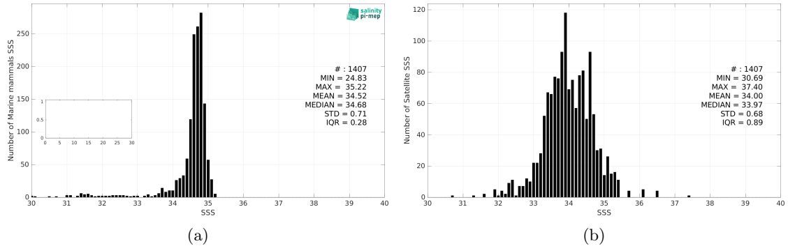
Figure 3: Histograms of SSS from Marine mammals (a) and SMOS SSS L3 Arctic v4 - 9 Days (BEC) (b) considering all match-up pairs per bins of 0.1 over the Arctic Ocean Pi-MEP region and for the full satellite product period.
