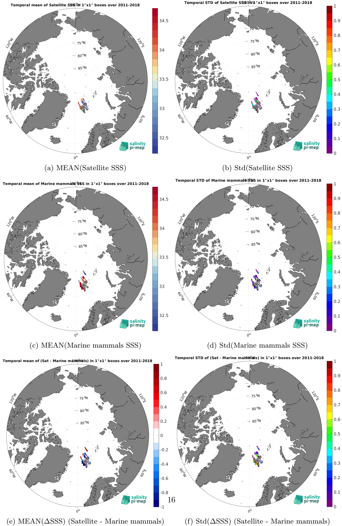
Figure 7: Temporal mean (left) and Std (right) of SSS from SMOS SSS L3 Arctic v4 - 9 Days (BEC) (top), Marine mammals (middle), and of \Delta SSS (Satellite - Marine mammals). Only match-up pairs are used to generate these maps.
