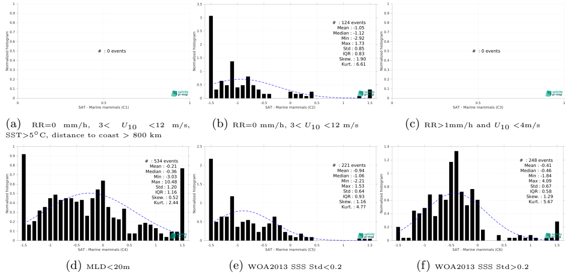
Figure 15: Normalized histogram of \Delta SSS (SMOS SSS L3 Arctic v4 - 9 Days (BEC) - Marine mammals) for 6 different subdatasets corresponding to: RR=0 mm/h, 3 < U_{10} < 12 m/s, SST>5°C, distance to coast > 800 km (a), RR=0 mm/h, 3 < U_{10} < 12 m/s (b), RR>1mm/h and U_{10} < 4 m/s (c), MLD<20m (d), WOA2013 SSS Std<0.2 (e), WOA2013 SSS Std>0.2 (f).
