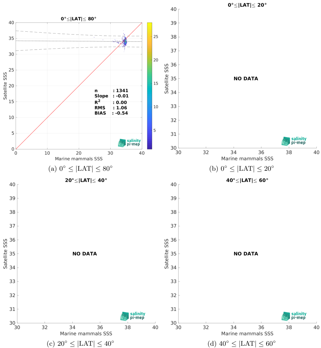
Figure 10: Contour maps of the concentration of SMOS SSS L3 Arctic v4 - 9 Days (BEC) SSS (y-axis) versus Marine mammals SSS (x-axis) at match-up pairs for different latitude bands. For each plot, the red line shows x=y . The black thin and dashed lines indicate a linear fit through the data cloud and the \pm 95\% confidence levels, respectively. The number match-up pairs n , the slope and R^2 coefficient of the linear fit, the root mean square (RMS) and the mean bias between satellite and in situ data are indicated for each latitude band in each plots.
