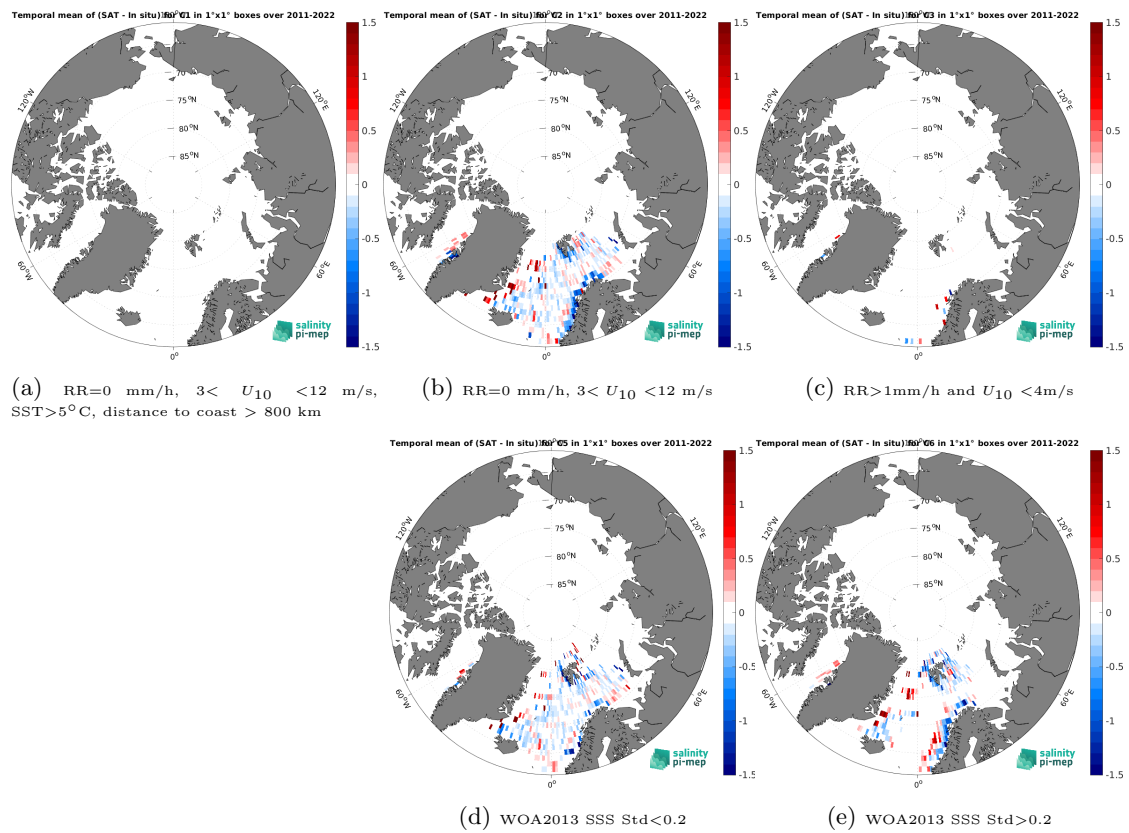
Figure 14: Temporal mean gridded over spatial boxes of size 1^\circ \times 1^\circ of \Delta\text{SSS} (SMOS SSS L3 Arctic v4 - 9 Days (BEC) - ICES) for 5 different subdatasets corresponding to:RR=0 mm/h, 3 < U_{10} < 12 m/s, SST>5°C, distance to coast > 800 km (a), RR=0 mm/h, 3 < U_{10} < 12 m/s (b), RR>1mm/h and U_{10} < 4 m/s (c), WOA2013 SSS Std<0.2 (d), WOA2013 SSS Std>0.2 (e).
