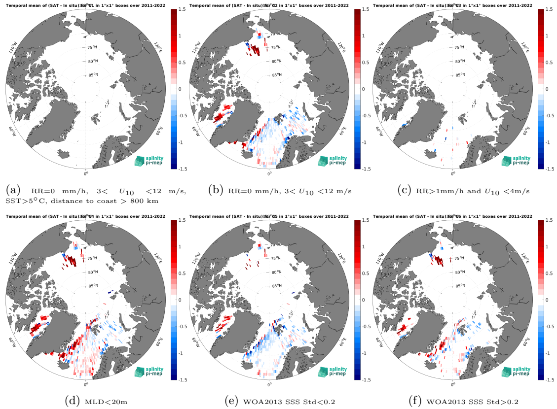
Figure 14: Temporal mean gridded over spatial boxes of size 1^\circ \times 1^\circ of \Delta SSS (SMOS SSS L3 Arctic v4 - 9 Days (BEC) - Argo) for 6 different subdatasets corresponding to:RR=0 mm/h, 3 < U_{10} < 12 m/s, SST>5°C, distance to coast > 800 km (a), RR=0 mm/h, 3 < U_{10} < 12 m/s (b), RR>1mm/h and U_{10} < 4 m/s (c),MLD<20m (d),WOA2013 SSS Std<0.2 (e),WOA2013 SSS Std>0.2 (f).
