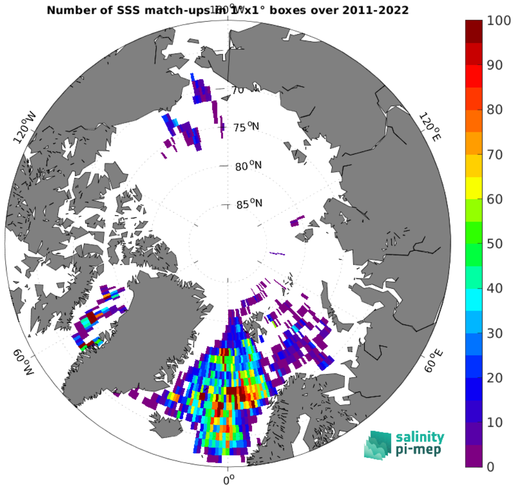
Figure 5: Number of SSS match-ups between Argo SSS and the SMOS SSS L3 Arctic v4 - 9 Days (BEC) SSS product for the Arctic Ocean Pi-MEP region over 1^\circ \times 1^\circ boxes and for the full satellite product period.
