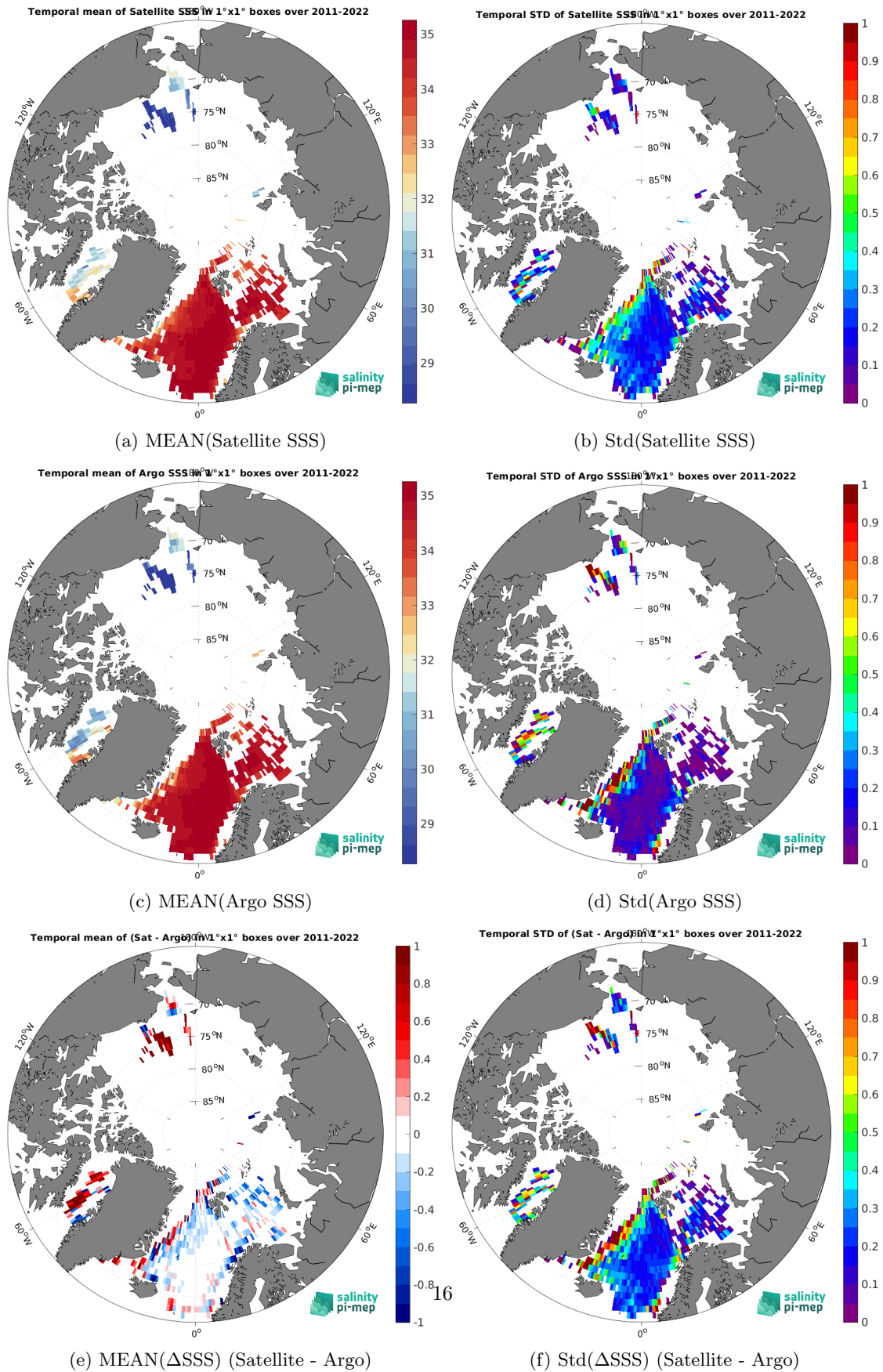
Figure 7: Temporal mean (left) and Std (right) of SSS from SMOS SSS L3 Arctic v4 - 9 Days (BEC) (top), Argo (middle), and of \Delta SSS (Satellite - Argo). Only match-up pairs are used to generate these maps.
