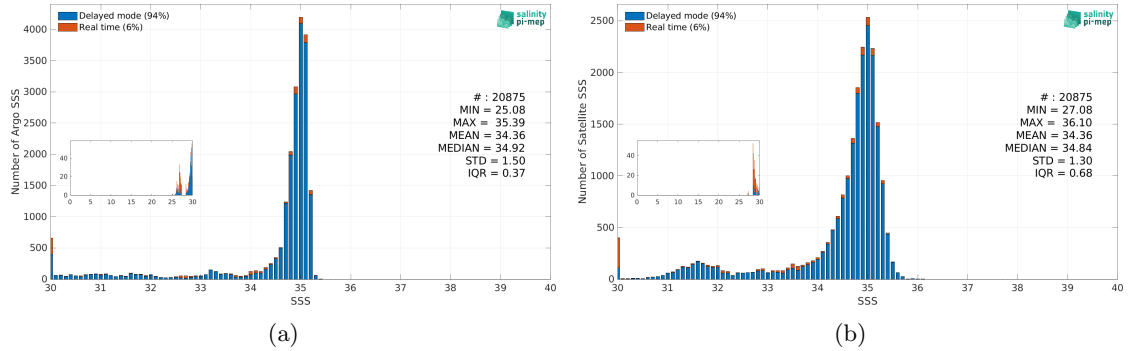
Figure 3: Histograms of SSS from Argo (a) and SMOS SSS L3 Arctic v4 - 9 Days (BEC) (b) considering all match-up pairs per bins of 0.1 over the Arctic Ocean Pi-MEP region and for the full satellite product period.
