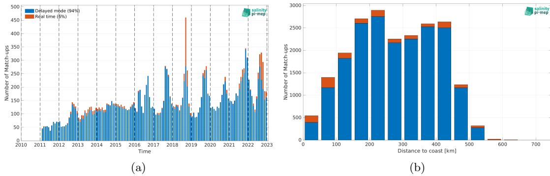
Figure 2: Number of match-ups between Argo and SMOS SSS L3 Arctic v4 - 9 Days (BEC) SSS as a function of time (a) and as function of the distance to coast (b) over the Arctic Ocean Pi-MEP region and for the full satellite product period.
