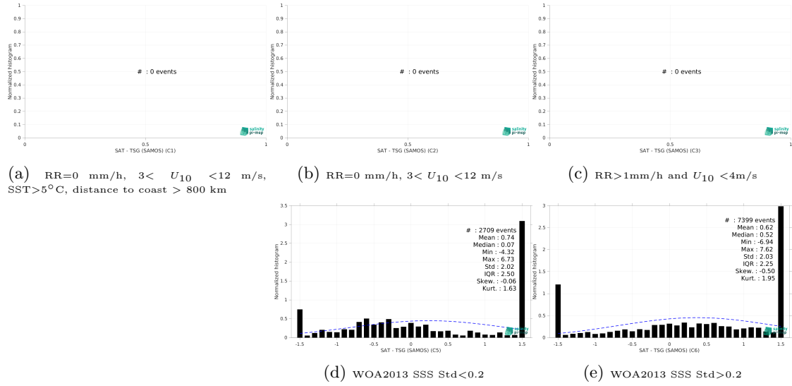
Figure 13: Normalized histogram of \Delta SSS (SMOS SSS L3 Arctic v3.1 - 9 Days (BEC) - TSG (SAMOS)) for 5 different subdatasets corresponding to: RR=0 mm/h, 3 < U_{10} < 12 m/s, SST>5°C, distance to coast > 800 km (a), RR=0 mm/h, 3 < U_{10} < 12 m/s (b), RR>1mm/h and U_{10} < 4 m/s (c), WOA2013 SSS Std<0.2 (d), WOA2013 SSS Std>0.2 (e).
