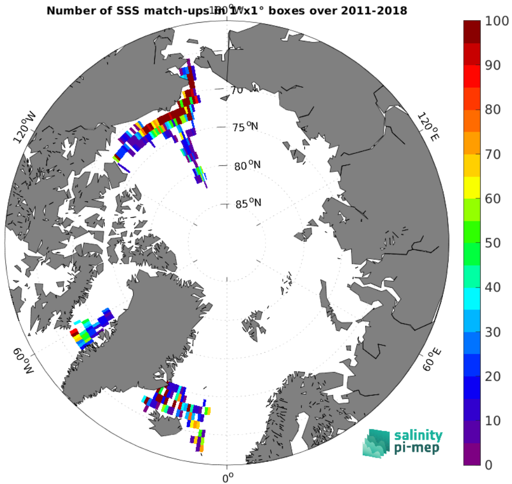
Figure 4: Number of SSS match-ups between TSG (SAMOS) SSS and the SMOS SSS L3 Arctic v3.1 - 9 Days (BEC) SSS product for the Arctic Ocean Pi-MEP region over 1^\circ \times 1^\circ boxes and for the full satellite product period.
