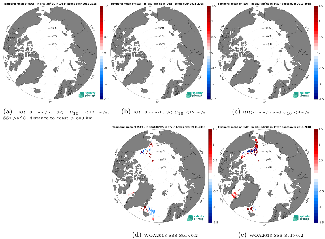
Figure 12: Temporal mean gridded over spatial boxes of size 1^{\circ}\times 1^{\circ} of \Delta\text{SSS} (SMOS SSS L3 Arctic v3.1 - 9 Days (BEC) - TSG (SAMOS)) for 5 different subdatasets corresponding to:RR=0 mm/h, 3 < U_{10} < 12 m/s, SST >5^{\circ}\text{C} , distance to coast > 800 km (a), RR=0 mm/h, 3 < U_{10} < 12 m/s (b), RR >1 mm/h and U_{10} < 4 m/s (c), WOA2013 SSS Std <0.2 (d), WOA2013 SSS Std >0.2 (e).
