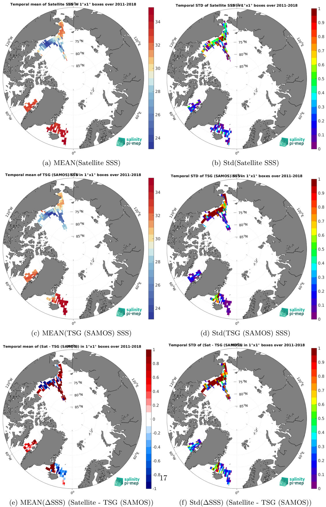
Figure 6: Temporal mean (left) and Std (right) of SSS from SMOS SSS L3 Arctic v3.1 - 9 Days (BEC) (top), TSG (SAMOS) (middle), and of \Delta SSS (Satellite - TSG (SAMOS)). Only match-up pairs are used to generate these maps.
