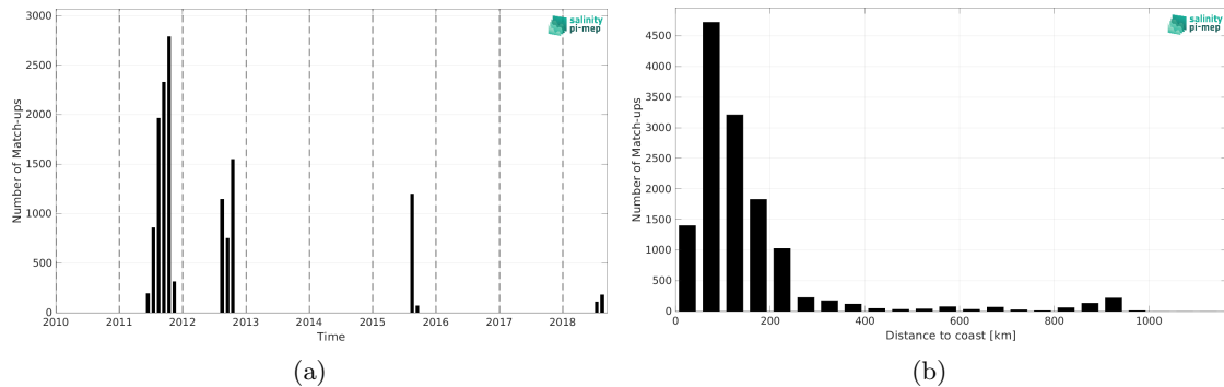
Figure 1: Number of match-ups between TSG (SAMOS) and SMOS SSS L3 Arctic v3.1 - 9 Days (BEC) SSS as a function of time (a) and as function of the distance to coast (b) over the Arctic Ocean Pi-MEP region and for the full satellite product period.
