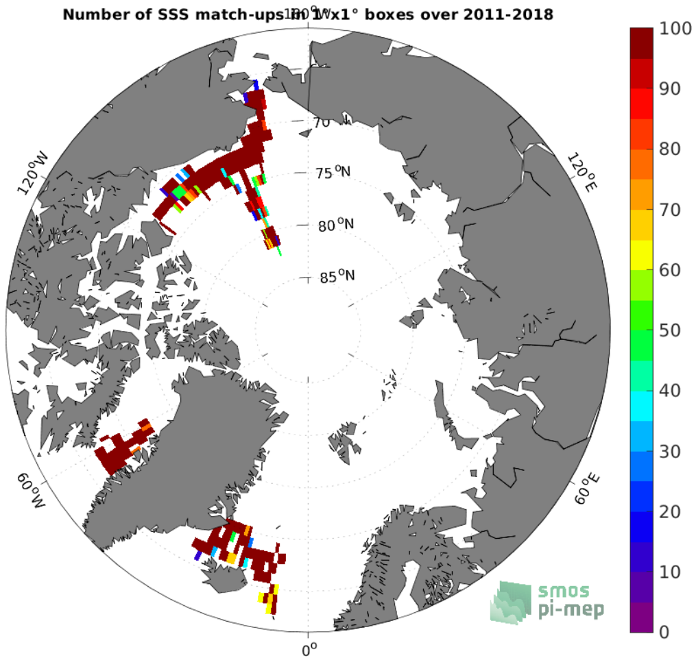
Figure 4: Number of SSS match-ups between TSG (SAMOS) SSS and the SMOS SSS L3 Arctic v3.1 - 9 Days (BEC) SSS product for the Arctic Ocean Pi-MEP region over 1^{\circ} \times 1^{\circ} boxes and for the full satellite product period.
