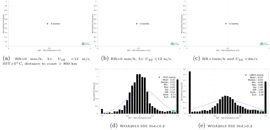
Figure 13: Normalized histogram of \Delta SSS (SMOS SSS L3 Arctic v3.1 - 9 Days (BEC) - TSG (Polarstern)) for 5 different subdatasets corresponding to: RR=0 mm/h, 3 < U_{10} < 12 m/s, SST>5°C, distance to coast > 800 km (a), RR=0 mm/h, 3 < U_{10} < 12 m/s (b), RR>1mm/h and U_{10} < 4 m/s (c), WOA2013 SSS Std<0.2 (d), WOA2013 SSS Std>0.2 (e).
