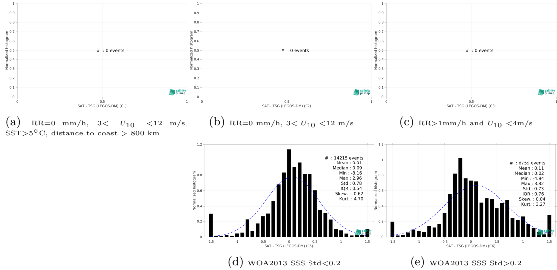
Figure 13: Normalized histogram of \Delta SSS (SMOS SSS L3 Arctic v3.1 - 9 Days (BEC) - TSG (LEGOS-DM)) for 5 different subdatasets corresponding to: RR=0 mm/h, 3 < U_{10} < 12 m/s, SST >5^{\circ}\text{C} , distance to coast > 800 km (a), RR=0 mm/h, 3 < U_{10} < 12 m/s (b), RR >1 mm/h and U_{10} < 4 m/s (c), WOA2013 SSS Std <0.2 (d), WOA2013 SSS Std >0.2 (e).
