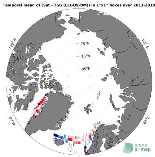
(e) MEAN( \Delta SSS) (Satellite - TSG (LEGOS-DM))
