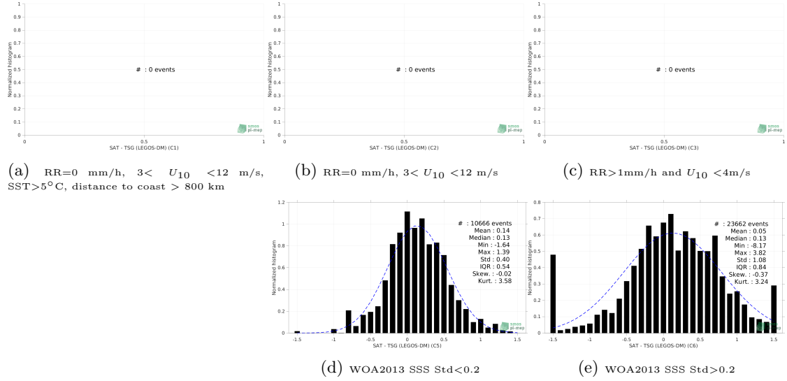
Figure 13: Normalized histogram of \Delta SSS (SMOS SSS L3 Arctic v3.1 - 9 Days (BEC) - TSG (LEGOS-DM)) for 5 different subdatasets corresponding to: RR=0 mm/h, 3 < U_{10} < 12 m/s, SST > 5°C, distance to coast > 800 km (a), RR=0 mm/h, 3 < U_{10} < 12 m/s (b), RR > 1mm/h and U_{10} < 4 m/s (c), WOA2013 SSS Std < 0.2 (d), WOA2013 SSS Std > 0.2 (e).
