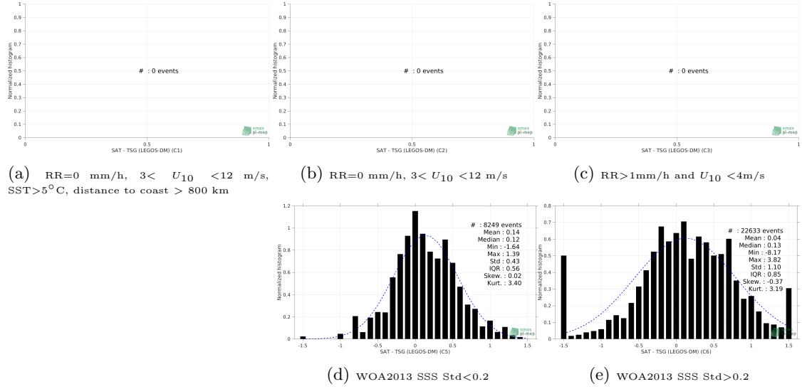
Figure 13: Normalized histogram of \Delta SSS (SMOS SSS L3 Arctic v3.1 - 9 Days (BEC) - TSG (LEGOS-DM)) for 5 different subdatasets corresponding to: RR=0 mm/h, 3 < U_{10} < 12 m/s, SST>5°C, distance to coast > 800 km (a), RR=0 mm/h, 3 < U_{10} < 12 m/s (b), RR>1mm/h and U_{10} < 4 m/s (c), WOA2013 SSS Std<0.2 (d), WOA2013 SSS Std>0.2 (e).
