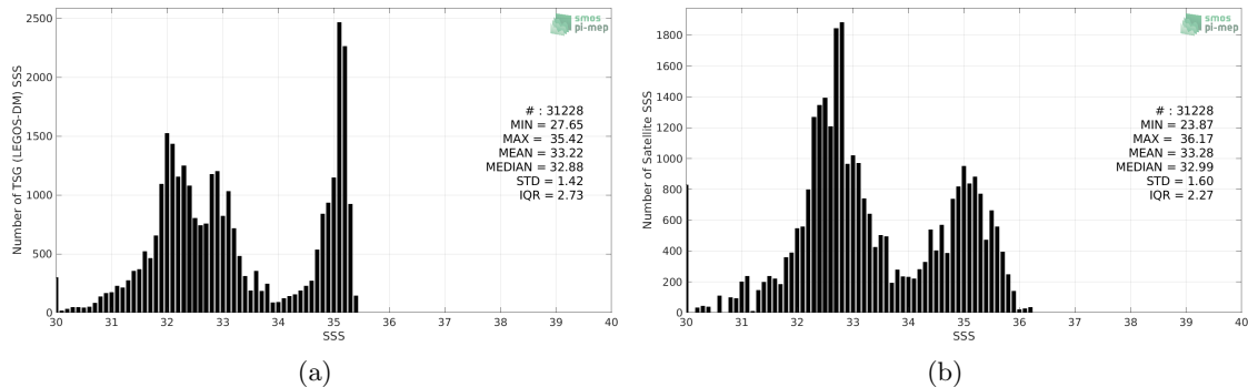
Figure 2: Histograms of SSS from TSG (LEGOS-DM) (a) and SMOS SSS L3 Arctic v3.1 - 9 Days (BEC) (b) considering all match-up pairs per bins of 0.1 over the Arctic Ocean Pi-MEP region and for the full satellite product period.
