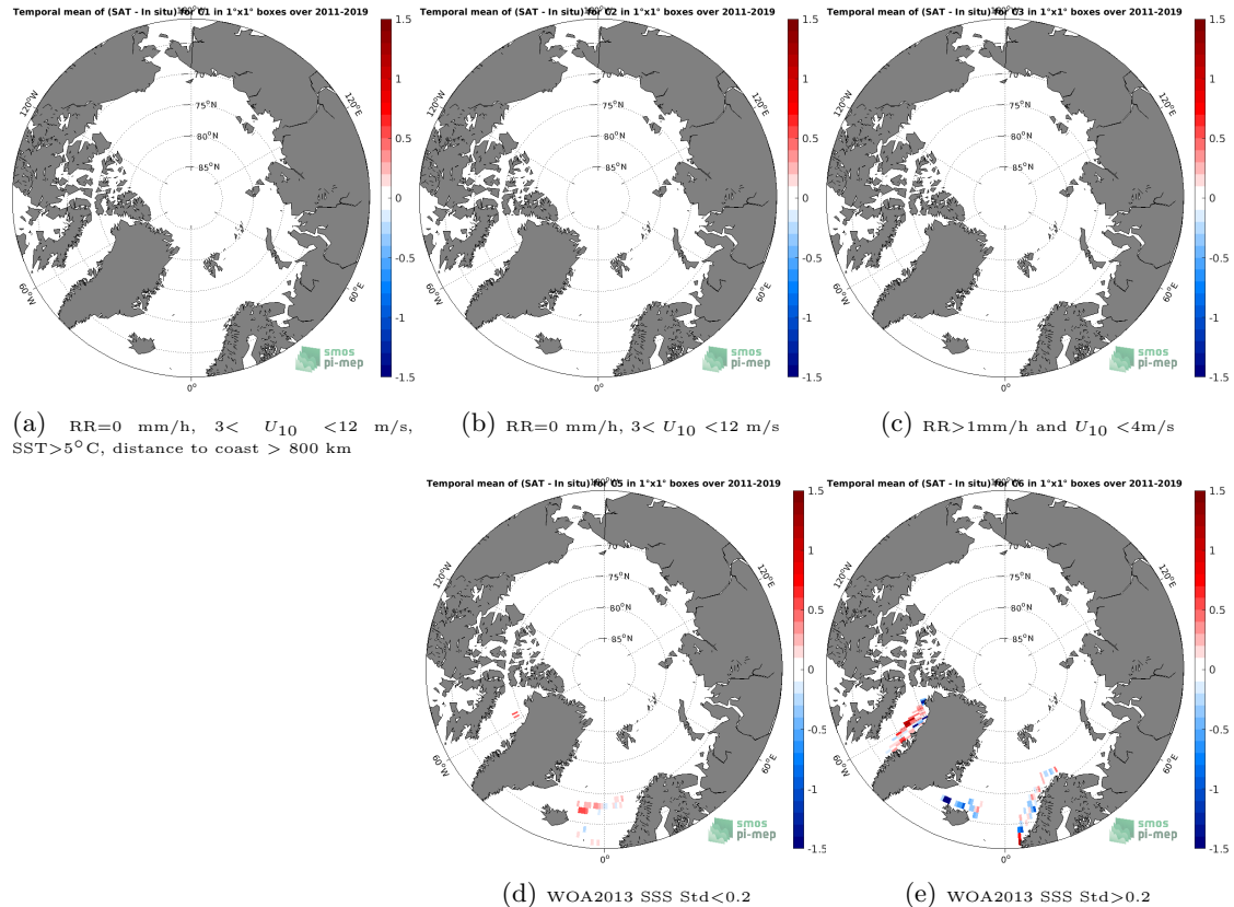
Figure 12: Temporal mean gridded over spatial boxes of size 1^{\circ}\times 1^{\circ} of \Delta\text{SSS} (SMOS SSS L3 Arctic v3.1 - 9 Days (BEC) - TSG (LEGOS-DM)) for 5 different subdatasets corresponding to: RR=0 mm/h, 3 < U_{10} < 12 m/s, SST > 5^{\circ}\text{C} , distance to coast > 800 km (a), RR=0 mm/h, 3 < U_{10} < 12 m/s (b), RR > 1 mm/h and U_{10} < 4 m/s (c), WOA2013 SSS Std < 0.2 (d), WOA2013 SSS Std > 0.2 (e).
