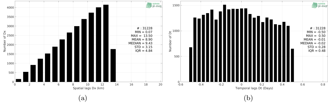
Figure 5: Histograms of the spatial (a) and temporal (b) lags between the location/time of the TSG (LEGOS-DM) measurement and the date of the corresponding SMOS SSS L3 Arctic v3.1 - 9 Days (BEC) SSS pixel.
