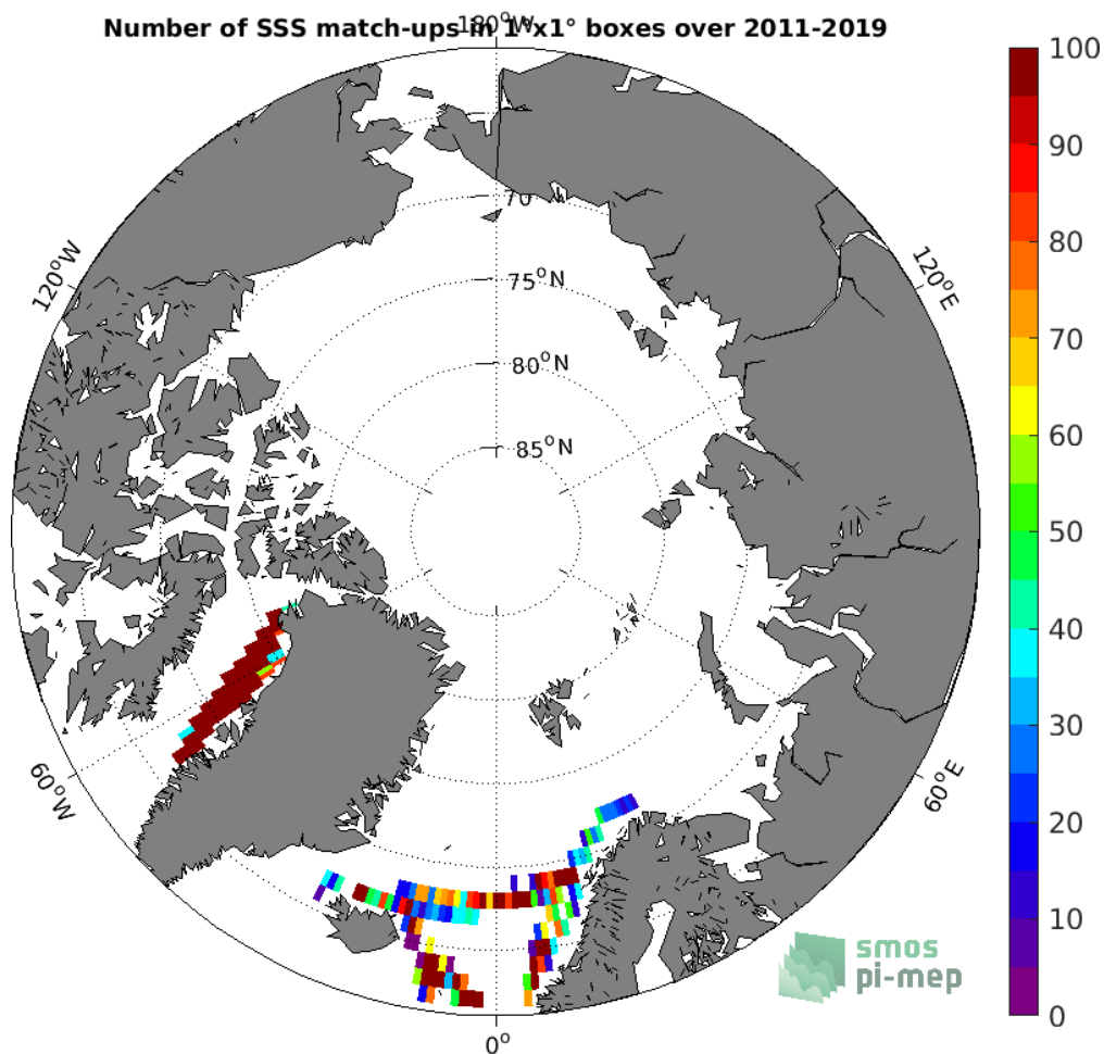
Figure 4: Number of SSS match-ups between TSG (LEGOS-DM) SSS and the SMOS SSS L3 Arctic v3.1 - 9 Days (BEC) SSS product for the Arctic Ocean Pi-MEP region over 1^\circ \times 1^\circ boxes and for the full satellite product period.
