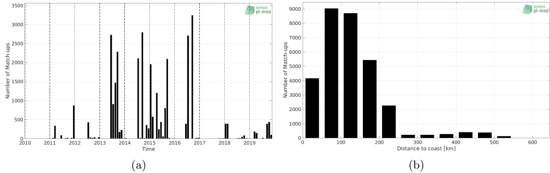
Figure 1: Number of match-ups between TSG (LEGOS-DM) and SMOS SSS L3 Arctic v3.1 - 9 Days (BEC) SSS as a function of time (a) and as function of the distance to coast (b) over the Arctic Ocean Pi-MEP region and for the full satellite product period.
