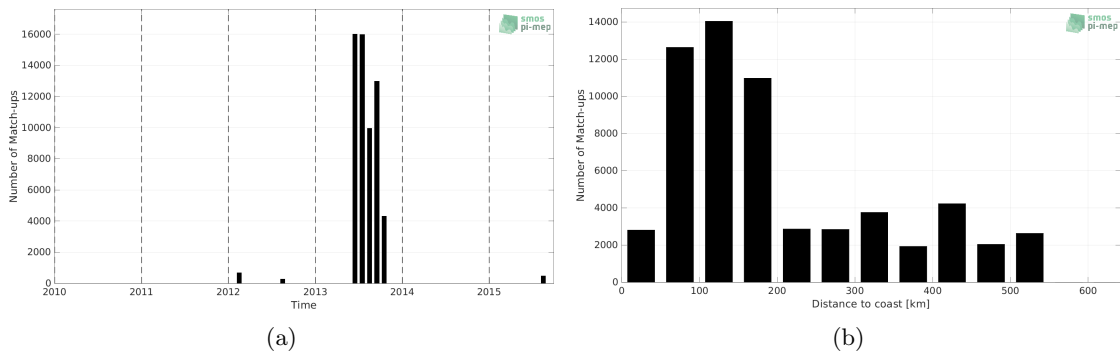
Figure 1: Number of match-ups between TSG (GOSUD-Sailing-ship) and SMOS SSS L3 Arctic v3.1 - 9 Days (BEC) SSS as a function of time (a) and as function of the distance to coast (b) over the Arctic Ocean Pi-MEP region and for the full satellite product period.
