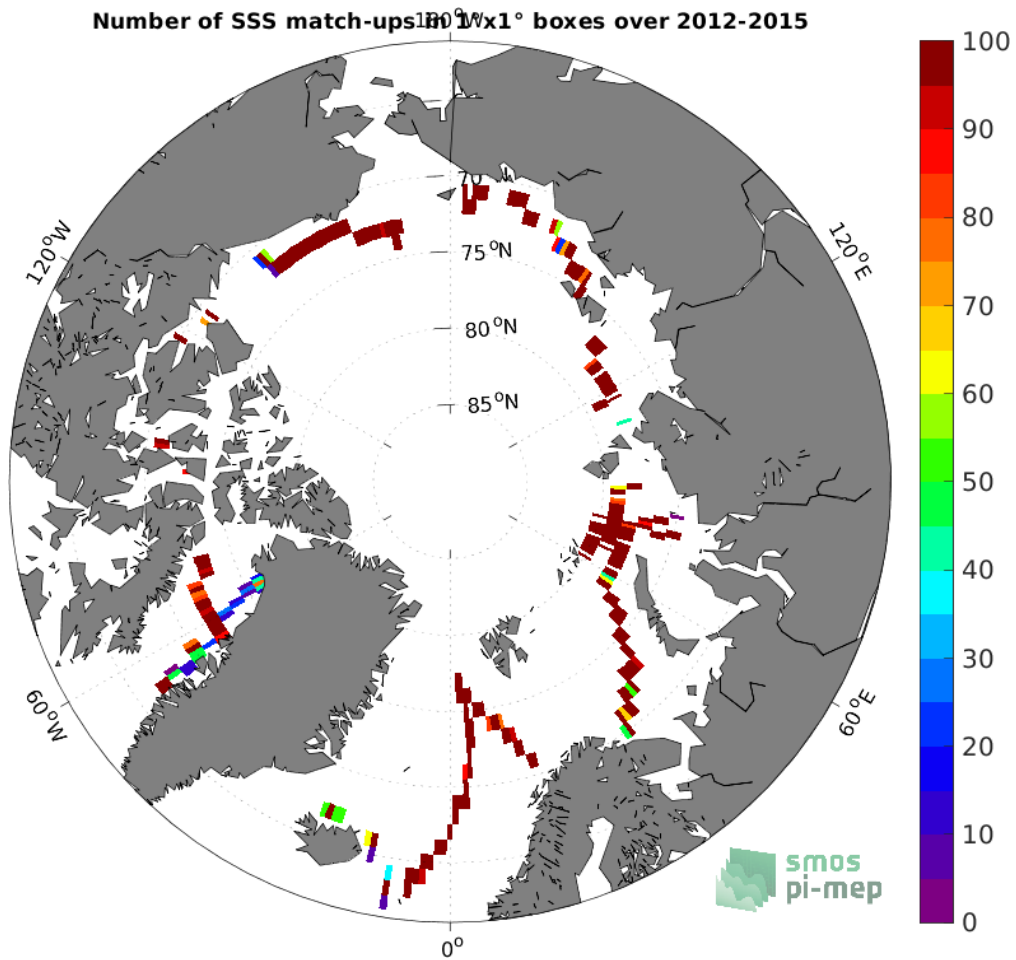
Figure 4: Number of SSS match-ups between TSG (GOSUD-Sailing-ship) SSS and the SMOS SSS L3 Arctic v3.1 - 9 Days (BEC) SSS product for the Arctic Ocean Pi-MEP region over 1^{\circ} \times 1^{\circ} boxes and for the full satellite product period.
