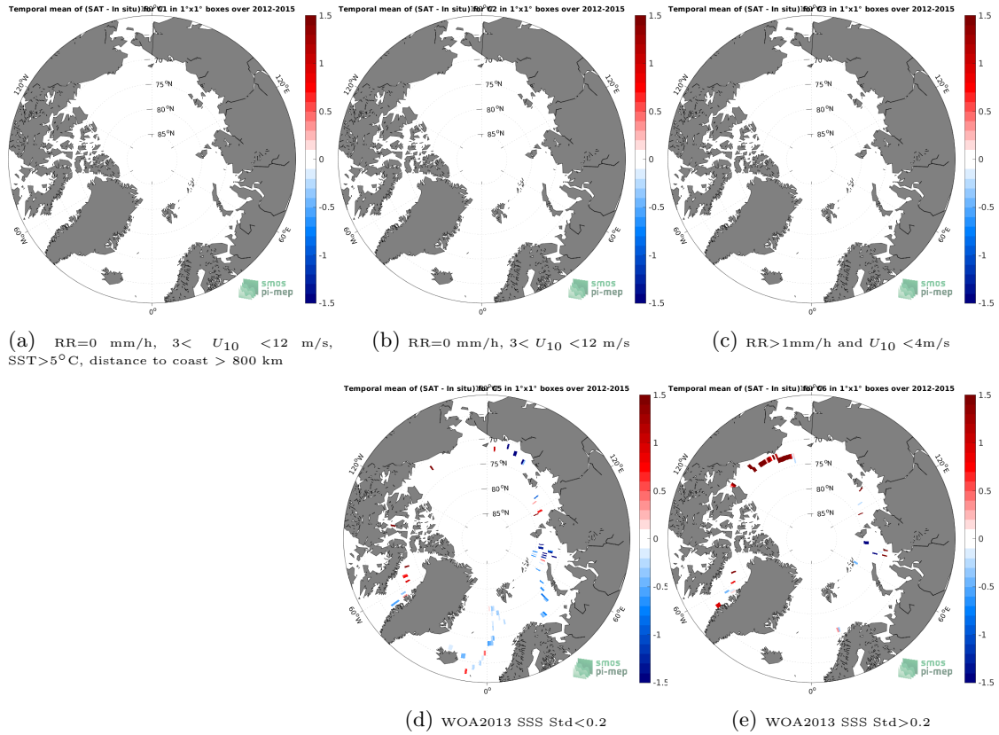
Figure 12: Temporal mean gridded over spatial boxes of size 1^\circ \times 1^\circ of \Delta SSS (SMOS SSS L3 Arctic v3.1 - 9 Days (BEC) - TSG (GOSUD-Sailing-ship)) for 5 different subdatasets corresponding to: RR=0 mm/h, 3 < U_{10} < 12 m/s, SST > 5°C, distance to coast > 800 km (a), RR=0 mm/h, 3 < U_{10} < 12 m/s (b), RR > 1mm/h and U_{10} < 4 m/s (c), WOA2013 SSS Std < 0.2 (d), WOA2013 SSS Std > 0.2 (e).
