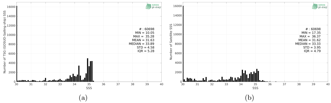
Figure 2: Histograms of SSS from TSG (GOSUD-Sailing-ship) (a) and SMOS SSS L3 Arctic v3.1 - 9 Days (BEC) (b) considering all match-up pairs per bins of 0.1 over the Arctic Ocean Pi-MEP region and for the full satellite product period.
