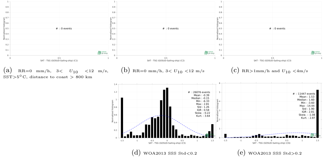
Figure 13: Normalized histogram of \Delta SSS (SMOS SSS L3 Arctic v3.1 - 9 Days (BEC) - TSG (GOSUD-Sailing-ship)) for 5 different subdatasets corresponding to: RR=0 mm/h, 3 < U_{10} < 12 m/s, SST > 5°C, distance to coast > 800 km (a), RR=0 mm/h, 3 < U_{10} < 12 m/s (b), RR > 1mm/h and U_{10} < 4 m/s (c), WOA2013 SSS Std < 0.2 (d), WOA2013 SSS Std > 0.2 (e).
