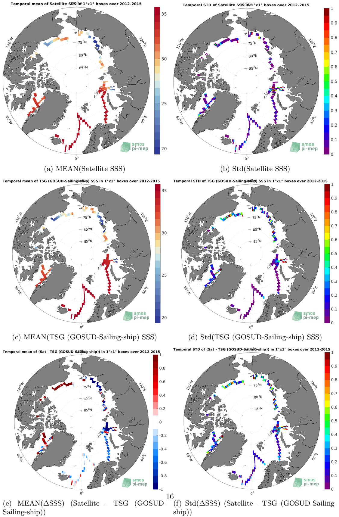
Figure 6: Temporal mean (left) and Std (right) of SSS from SMOS SSS L3 Arctic v3.1 - 9 Days (BEC) (top), TSG (GOSUD-Sailing-ship) (middle), and of \Delta SSS (Satellite - TSG (GOSUD-Sailing-ship)). Only match-up pairs are used to generate these maps.
