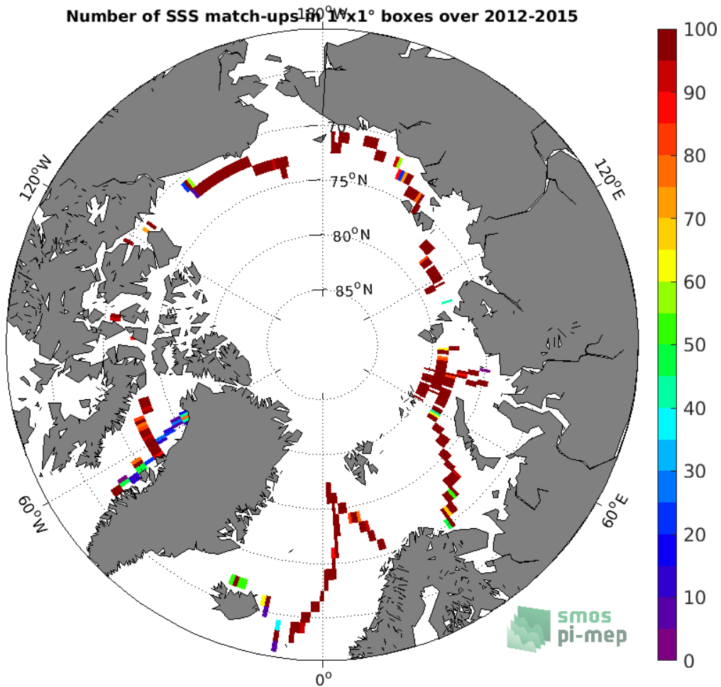
Figure 4: Number of SSS match-ups between TSG (GOSUD-Sailing-ship) SSS and the SMOS SSS L3 Arctic v3.1 - 9 Days (BEC) SSS product for the Arctic Ocean Pi-MEP region over 1^\circ \times 1^\circ boxes and for the full satellite product period.
