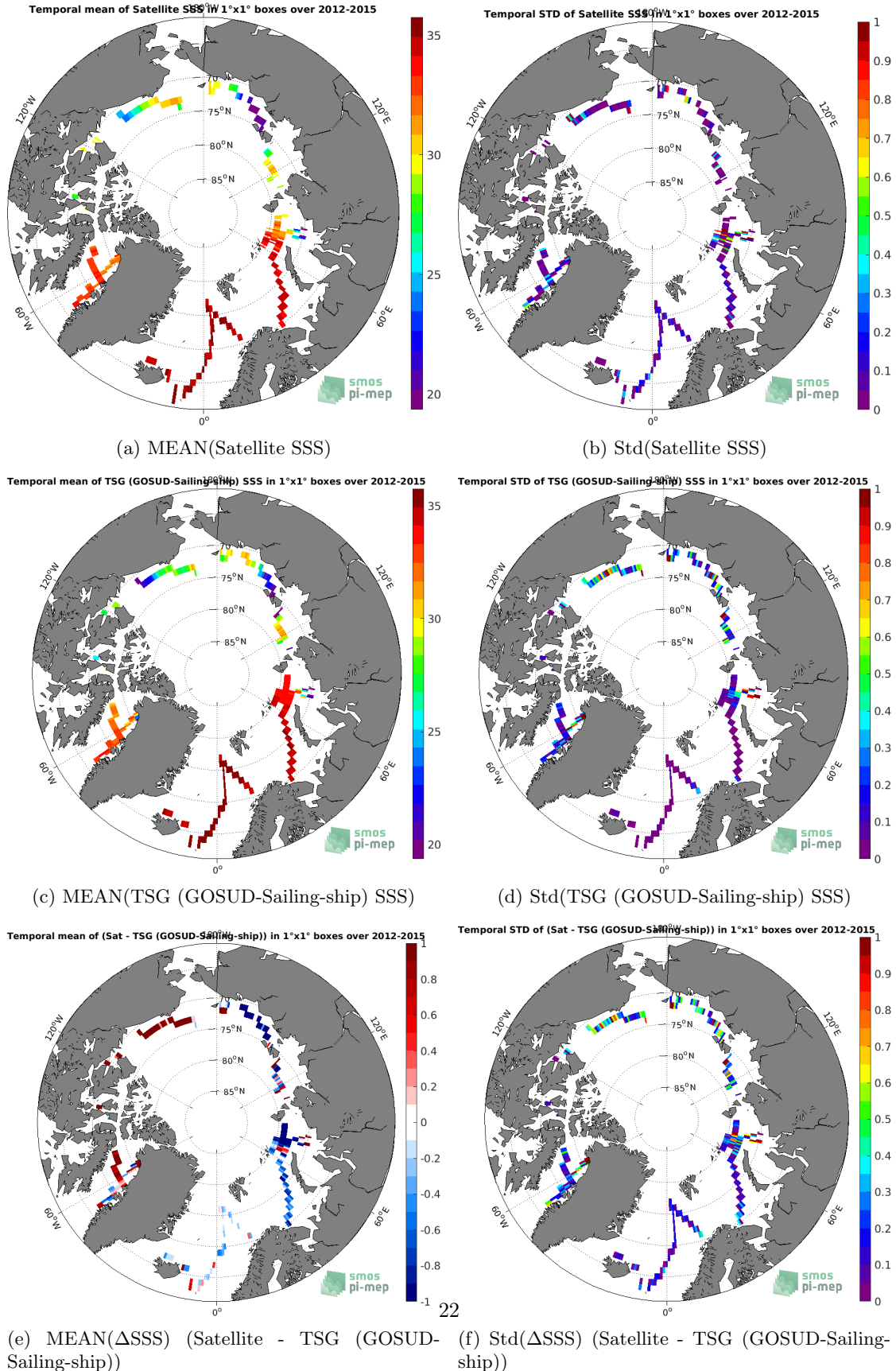
Figure 6: Temporal mean (left) and Std (right) of SSS from SMOS SSS L3 Arctic v3.1 - 9 Days (BEC) (top), TSG (GOSUD-Sailing-ship) (middle), and of \Delta SSS (Satellite - TSG (GOSUD-Sailing-ship)). Only match-up pairs are used to generate these maps.
