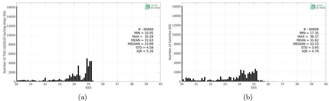
Figure 2: Histograms of SSS from TSG (GOSUD-Sailing-ship) (a) and SMOS SSS L3 Arctic v3.1 - 9 Days (BEC) (b) considering all match-up pairs per bins of 0.1 over the Arctic Ocean Pi-MEP region and for the full satellite product period.
