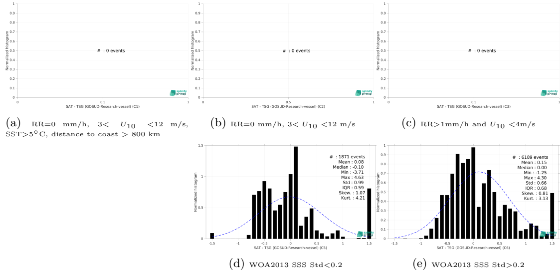
Figure 13: Normalized histogram of \Delta SSS (SMOS SSS L3 Arctic v3.1 - 9 Days (BEC) - TSG (GOSUD-Research-vessel)) for 5 different subdatasets corresponding to: RR=0 mm/h, 3 < U_{10} < 12 m/s, SST>5°C, distance to coast > 800 km (a), RR=0 mm/h, 3 < U_{10} < 12 m/s (b), RR>1mm/h and U_{10} < 4 m/s (c), WOA2013 SSS Std<0.2 (d), WOA2013 SSS Std>0.2 (e).
