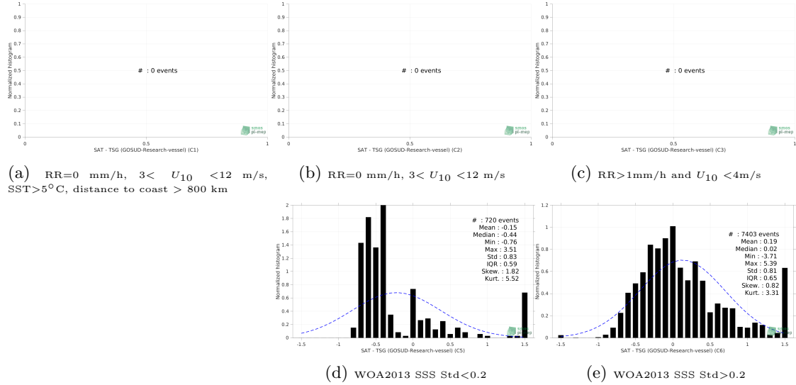
Figure 13: Normalized histogram of \Delta SSS (SMOS SSS L3 Arctic v3.1 - 9 Days (BEC) - TSG (GOSUD-Research-vessel)) for 5 different subdatasets corresponding to: RR=0 mm/h, 3 < U_{10} < 12 m/s, SST > 5°C, distance to coast > 800 km (a), RR=0 mm/h, 3 < U_{10} < 12 m/s (b), RR > 1mm/h and U_{10} < 4 m/s (c), WOA2013 SSS Std < 0.2 (d), WOA2013 SSS Std > 0.2 (e).
