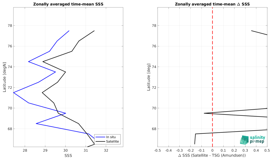
Figure 8: Left panel: Zonal mean SSS from SMOS SSS L3 Arctic v3.1 - 9 Days (BEC) satellite product (black) and from TSG (Amundsen) (blue). Right panel: Zonal mean of \Delta SSS (Satellite - TSG (Amundsen)) for all the collected Pi-MEP match-up pairs estimated over the full satellite product period.
