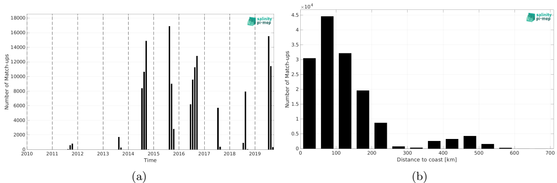
Figure 1: Number of match-ups between TSG (Amundsen) and SMOS SSS L3 Arctic v3.1 - 9 Days (BEC) SSS as a function of time (a) and as function of the distance to coast (b) over the Arctic Ocean Pi-MEP region and for the full satellite product period.
