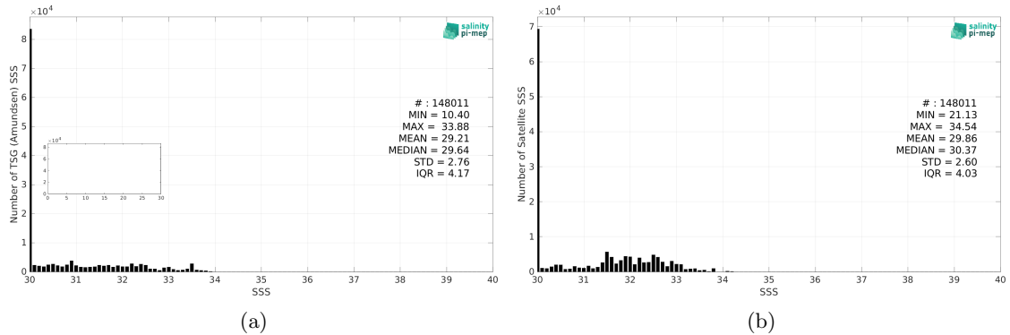
Figure 2: Histograms of SSS from TSG (Amundsen) (a) and SMOS SSS L3 Arctic v3.1 - 9 Days (BEC) (b) considering all match-up pairs per bins of 0.1 over the Arctic Ocean Pi-MEP region and for the full satellite product period.
