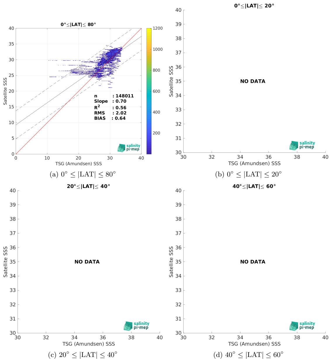
Figure 9: Contour maps of the concentration of SMOS SSS L3 Arctic v3.1 - 9 Days (BEC) SSS (y-axis) versus TSG (Amundsen) SSS (x-axis) at match-up pairs for different latitude bands. For each plot, the red line shows x=y . The black thin and dashed lines indicate a linear fit through the data cloud and the \pm 95\% confidence levels, respectively. The number match-up pairs n , the slope and R^2 coefficient of the linear fit, the root mean square (RMS) and the mean bias between satellite and in situ data are indicated for each latitude band in each plots.
