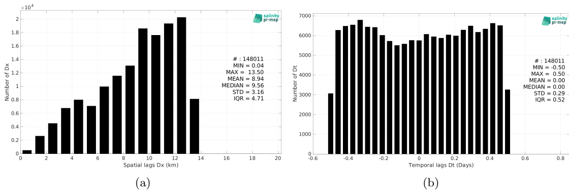
Figure 5: Histograms of the spatial (a) and temporal (b) lags between the location/time of the TSG (Amundsen) measurement and the date of the corresponding SMOS SSS L3 Arctic v3.1 - 9 Days (BEC) SSS pixel.
