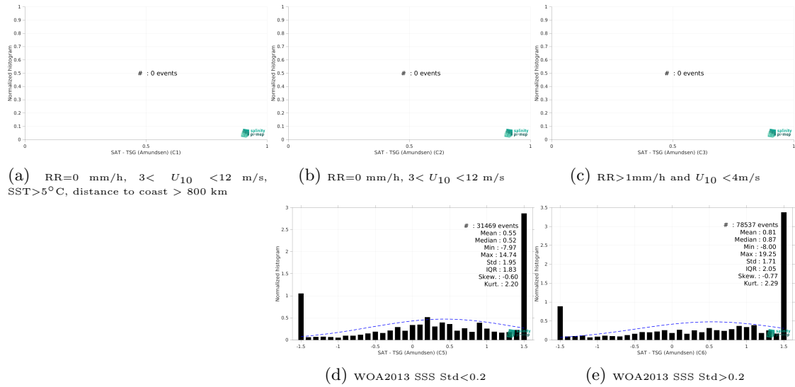
Figure 13: Normalized histogram of \Delta SSS (SMOS SSS L3 Arctic v3.1 - 9 Days (BEC) - TSG (Amundsen)) for 5 different subdatasets corresponding to: RR=0 mm/h, 3 < U_{10} < 12 m/s, SST > 5°C, distance to coast > 800 km (a), RR=0 mm/h, 3 < U_{10} < 12 m/s (b), RR > 1mm/h and U_{10} < 4 m/s (c), WOA2013 SSS Std < 0.2 (d), WOA2013 SSS Std > 0.2 (e).
