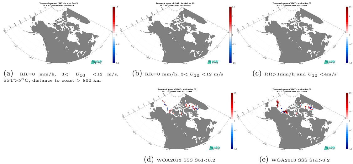
Figure 12: Temporal mean gridded over spatial boxes of size 1^{\circ}\times 1^{\circ} of \Delta\text{SSS} (SMOS SSS L3 Arctic v3.1 - 9 Days (BEC) - TSG (Amundsen)) for 5 different subdatasets corresponding to:RR=0 mm/h, 3 < U_{10} < 12 m/s, SST >5^{\circ}\text{C} , distance to coast > 800 km (a), RR=0 mm/h, 3 < U_{10} < 12 m/s (b), RR >1 mm/h and U_{10} < 4 m/s (c), WOA2013 SSS Std <0.2 (d), WOA2013 SSS Std >0.2 (e).
