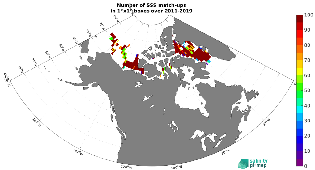
Figure 4: Number of SSS match-ups between TSG (Amundsen) SSS and the SMOS SSS L3 Arctic v3.1 - 9 Days (BEC) SSS product for the Arctic Ocean Pi-MEP region over 1°×1° boxes and for the full satellite product period.
