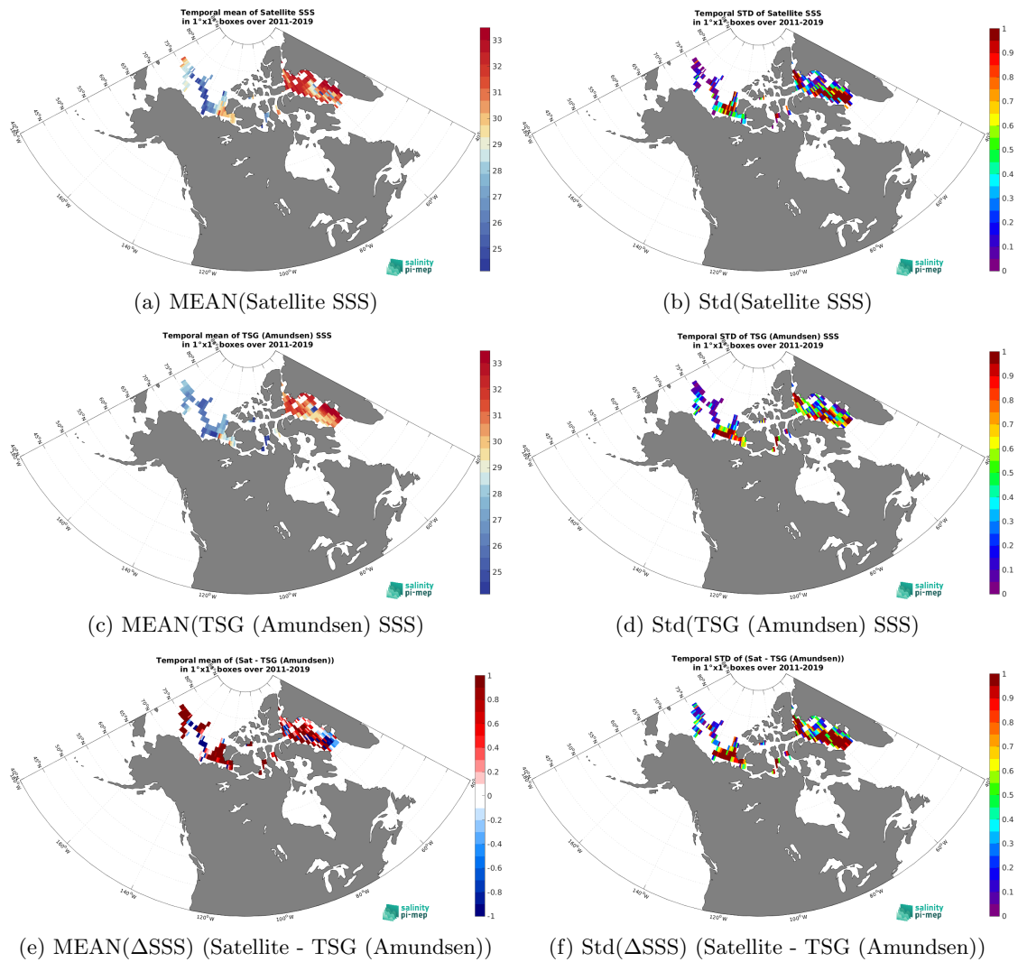
Figure 6: Temporal mean (left) and Std (right) of SSS from SMOS SSS L3 Arctic v3.1 - 9 Days (BEC) (top), TSG (Amundsen) (middle), and of \Delta SSS (Satellite - TSG (Amundsen)). Only match-up pairs are used to generate these maps.
