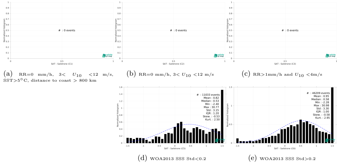
Figure 13: Normalized histogram of \Delta SSS (SMOS SSS L3 Arctic v3.1 - 9 Days (BEC) - Saldrone) for 5 different subdatasets corresponding to: RR=0 mm/h, 3 < U_{10} < 12 m/s, SST>5°C, distance to coast > 800 km (a), RR=0 mm/h, 3 < U_{10} < 12 m/s (b), RR>1mm/h and U_{10} < 4 m/s (c), WOA2013 SSS Std<0.2 (d), WOA2013 SSS Std>0.2 (e).
