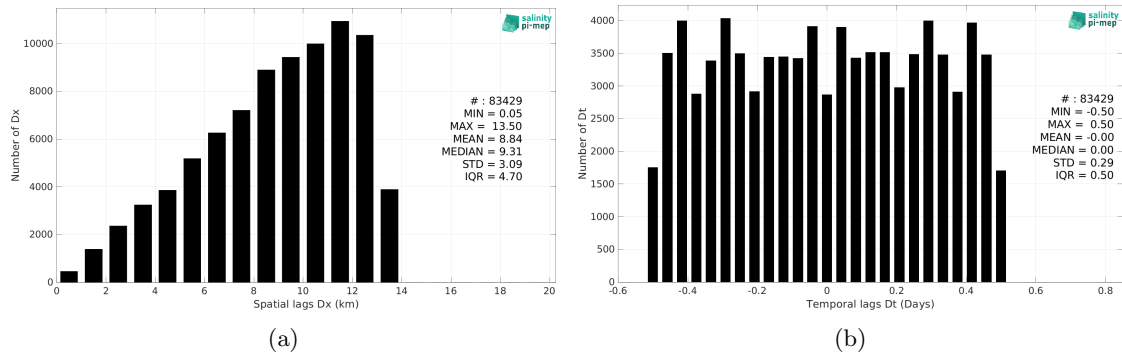
Figure 5: Histograms of the spatial (a) and temporal (b) lags between the location/time of the Saildrone measurement and the date of the corresponding SMOS SSS L3 Arctic v3.1 - 9 Days (BEC) SSS pixel.
