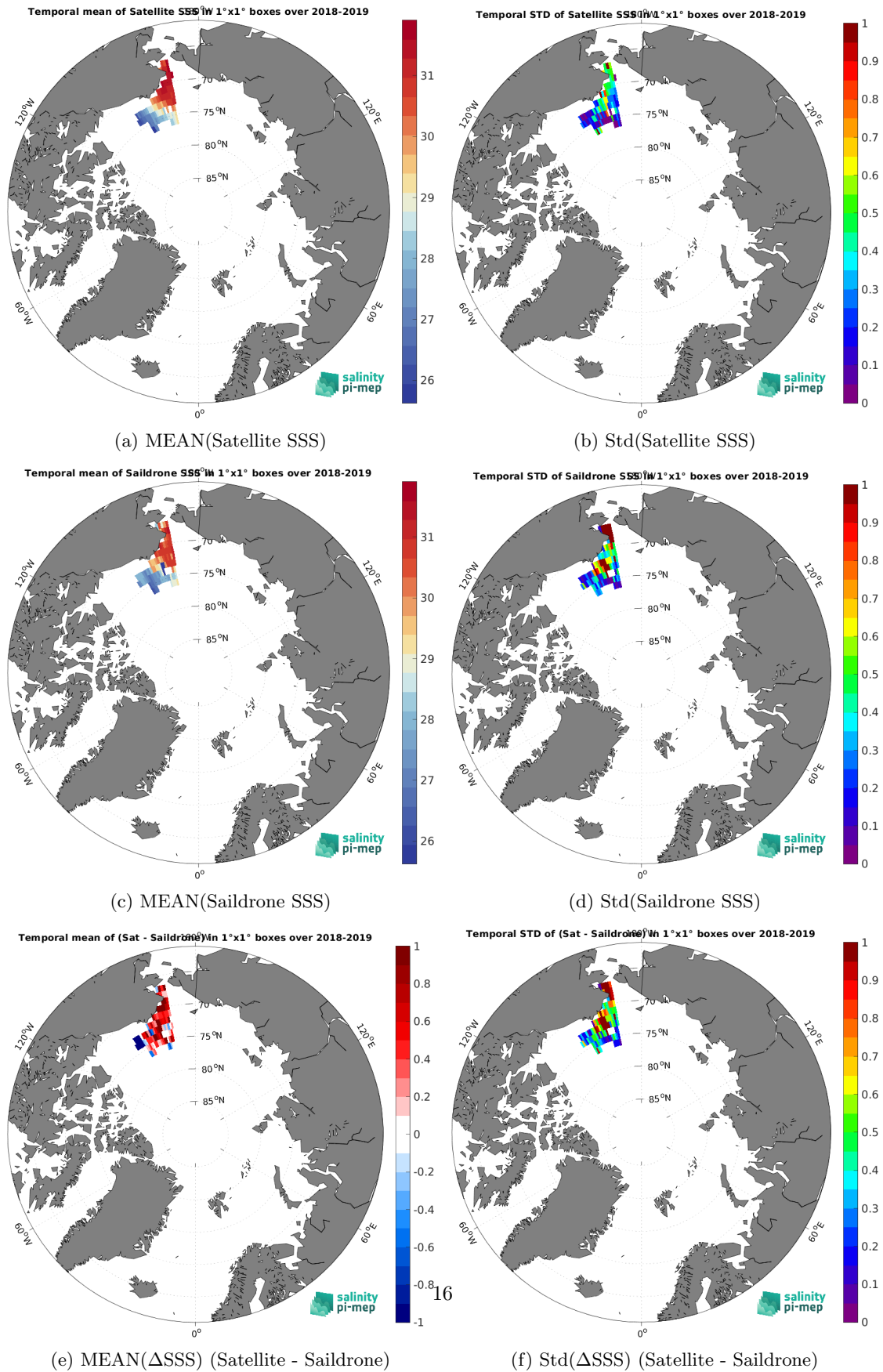
Figure 6: Temporal mean (left) and Std (right) of SSS from SMOS SSS L3 Arctic v3.1 - 9 Days (BEC) (top), Saildrone (middle), and of \Delta SSS (Satellite - Saildrone). Only match-up pairs are used to generate these maps.
