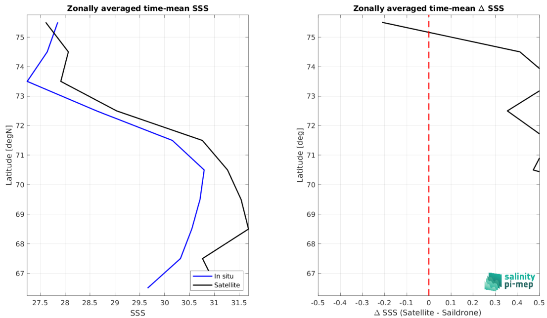
Figure 8: Left panel: Zonal mean SSS from SMOS SSS L3 Arctic v3.1 - 9 Days (BEC) satellite product (black) and from Sairdron (blue). Right panel: Zonal mean of \Delta SSS (Satellite - Sairdron) for all the collected Pi-MEP match-up pairs estimated over the full satellite product period.
