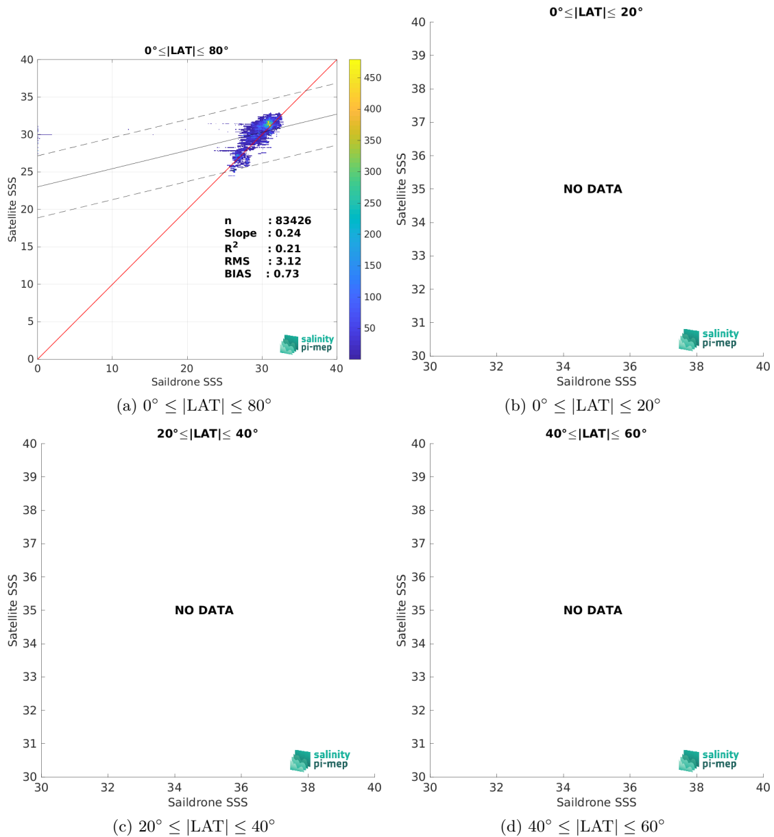
Figure 9: Contour maps of the concentration of SMOS SSS L3 Arctic v3.1 - 9 Days (BEC) SSS (y-axis) versus Saildrone SSS (x-axis) at match-up pairs for different latitude bands. For each plot, the red line shows x=y . The black thin and dashed lines indicate a linear fit through the data cloud and the \pm 95\% confidence levels, respectively. The number match-up pairs n , the slope and R^2 coefficient of the linear fit, the root mean square (RMS) and the mean bias between satellite and in situ data are indicated for each latitude band in each plots.
