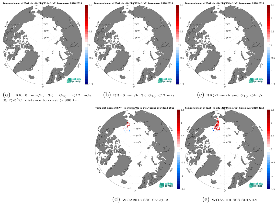
Figure 12: Temporal mean gridded over spatial boxes of size 1^{\circ}\times 1^{\circ} of \Delta\text{SSS} (SMOS SSS L3 Arctic v3.1 - 9 Days (BEC) - Sailability) for 5 different subdatasets corresponding to: RR=0 mm/h, 3 < U_{10} < 12 m/s, SST > 5^{\circ}\text{C} , distance to coast > 800 km (a), RR=0 mm/h, 3 < U_{10} < 12 m/s (b), RR > 1 mm/h and U_{10} < 4 m/s (c), WOA2013 SSS Std < 0.2 (d), WOA2013 SSS Std > 0.2 (e).
