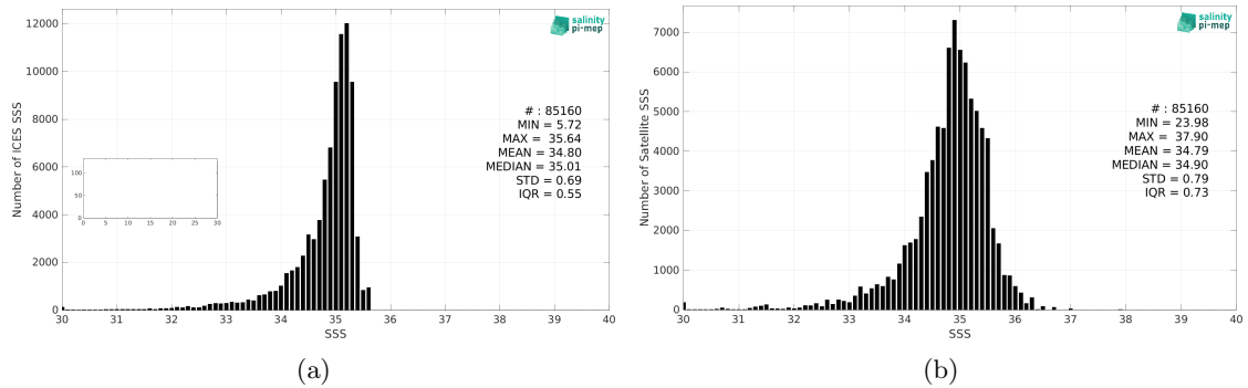
Figure 2: Histograms of SSS from ICES (a) and SMOS SSS L3 Arctic v3.1 - 9 Days (BEC) (b) considering all match-up pairs per bins of 0.1 over the Arctic Ocean Pi-MEP region and for the full satellite product period.
