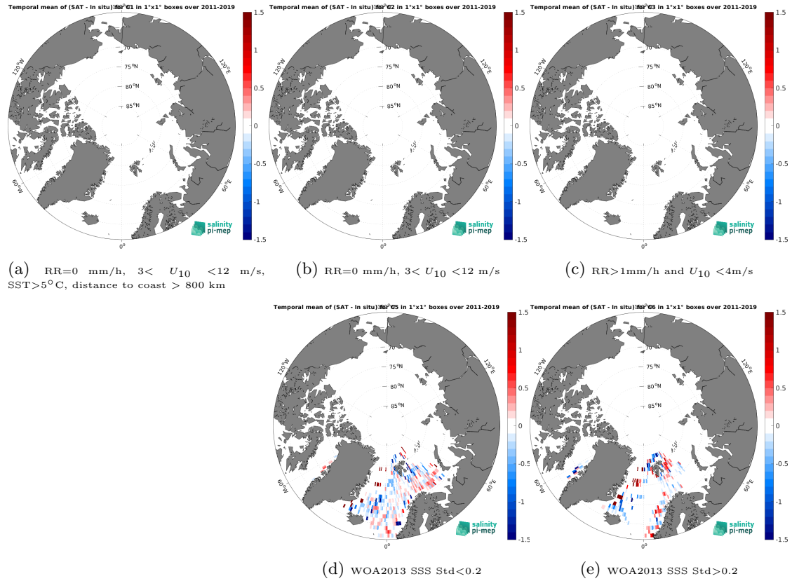
Figure 12: Temporal mean gridded over spatial boxes of size 1^{\circ}\times 1^{\circ} of \Delta\text{SSS} (SMOS SSS L3 Arctic v3.1 - 9 Days (BEC) - ICES) for 5 different subdatasets corresponding to:RR=0 mm/h, 3 < U_{10} < 12 m/s, SST > 5^{\circ}\text{C} , distance to coast > 800 km (a), RR=0 mm/h, 3 < U_{10} < 12 m/s (b), RR > 1 mm/h and U_{10} < 4 m/s (c), WOA2013 SSS Std < 0.2 (d), WOA2013 SSS Std > 0.2 (e).
