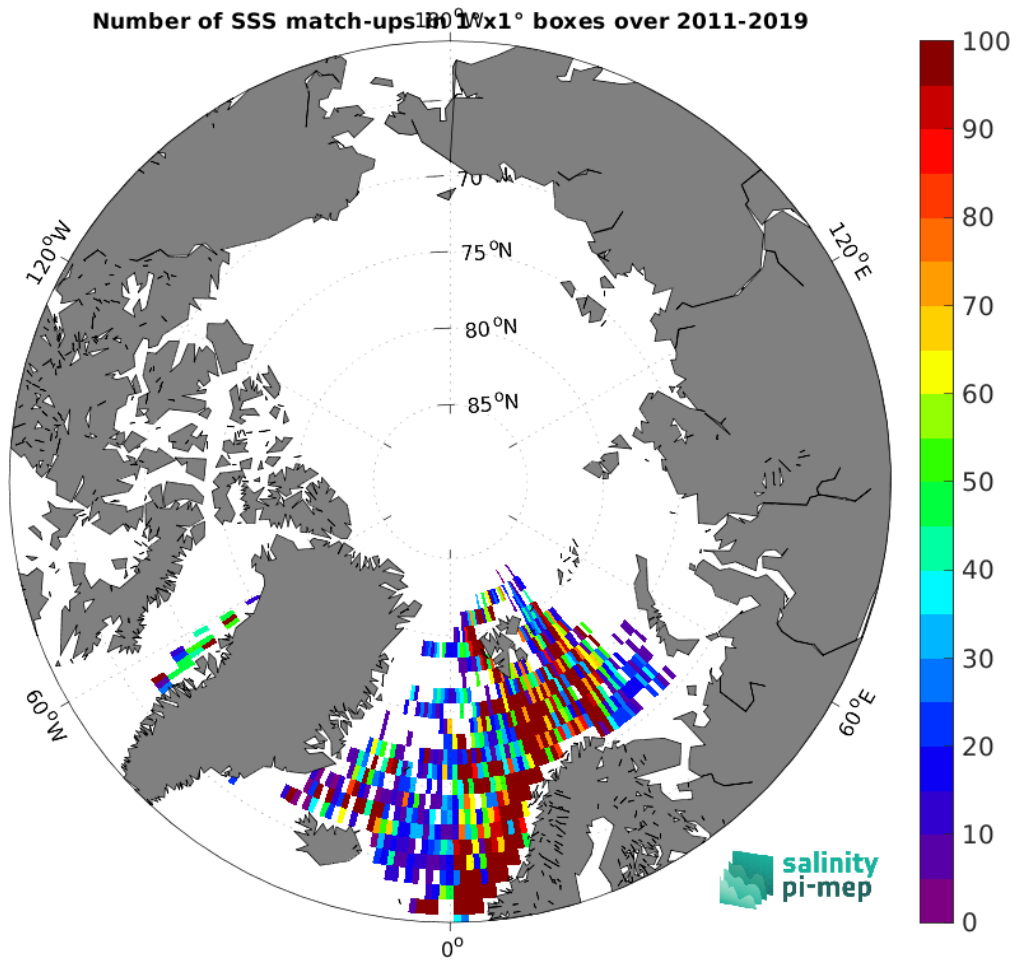
Figure 4: Number of SSS match-ups between ICES SSS and the SMOS SSS L3 Arctic v3.1 - 9 Days (BEC) SSS product for the Arctic Ocean Pi-MEP region over 1^\circ \times 1^\circ boxes and for the full satellite product period.
