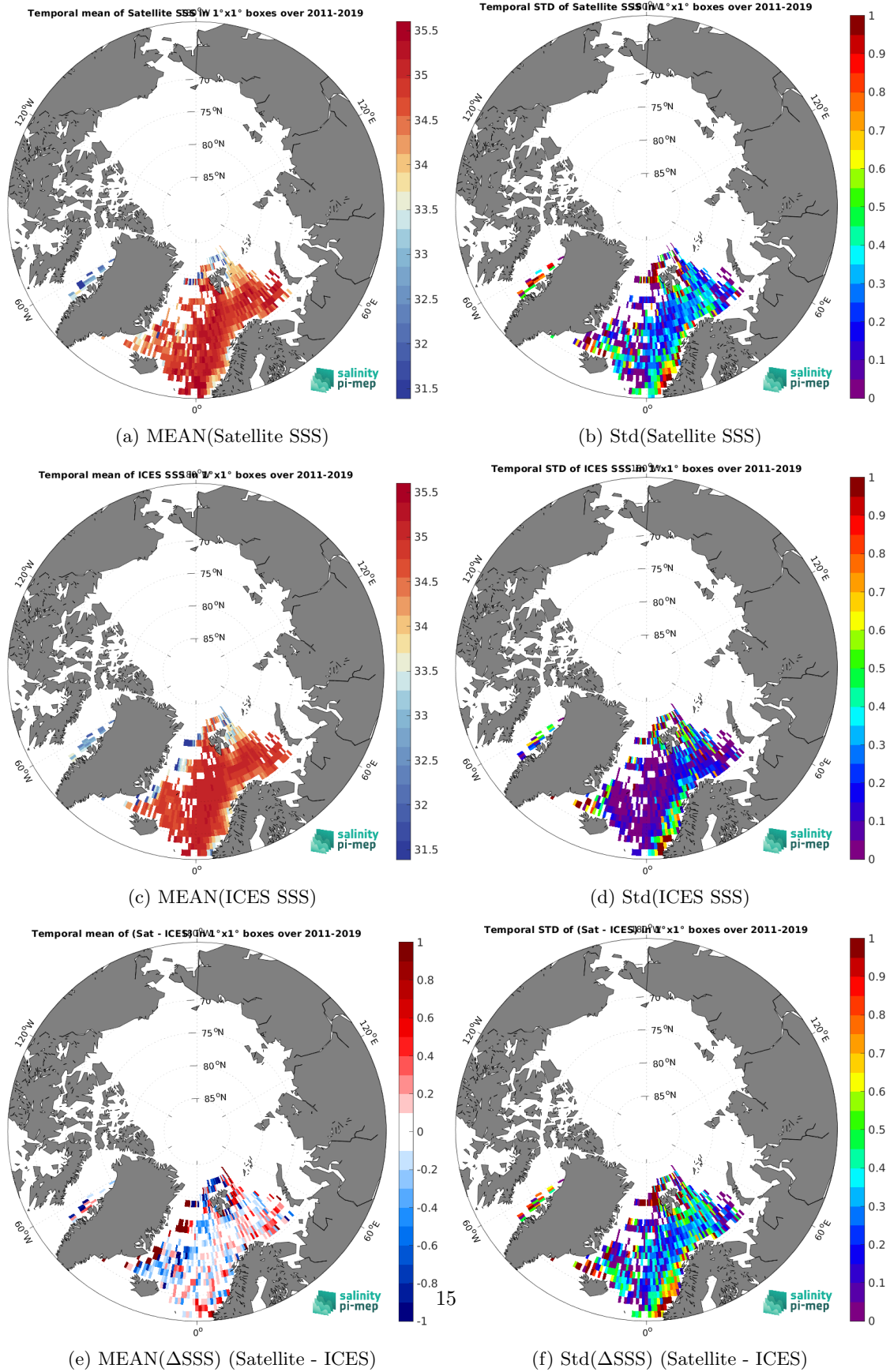
Figure 6: Temporal mean (left) and Std (right) of SSS from SMOS SSS L3 Arctic v3.1 - 9 Days (BEC) (top), ICES (middle), and of \Delta SSS (Satellite - ICES). Only match-up pairs are used to generate these maps.
