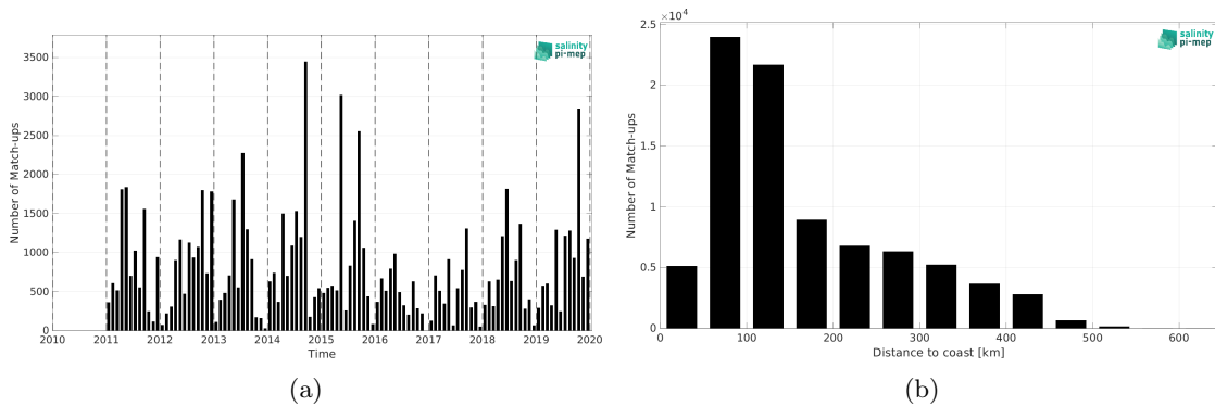
Figure 1: Number of match-ups between ICES and SMOS SSS L3 Arctic v3.1 - 9 Days (BEC) SSS as a function of time (a) and as function of the distance to coast (b) over the Arctic Ocean Pi-MEP region and for the full satellite product period.
