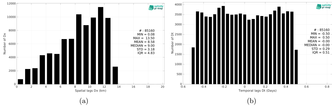
Figure 5: Histograms of the spatial (a) and temporal (b) lags between the location/time of the ICES measurement and the date of the corresponding SMOS SSS L3 Arctic v3.1 - 9 Days (BEC) SSS pixel.
