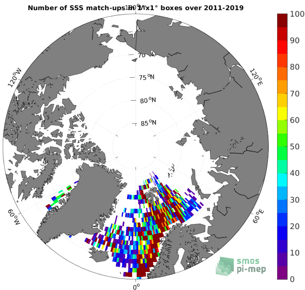
Figure 4: Number of SSS match-ups between ICES SSS and the SMOS SSS L3 Arctic v3.1 - 9 Days (BEC) SSS product for the Arctic Ocean Pi-MEP region over 1^{\circ} \times 1^{\circ} boxes and for the full satellite product period.
