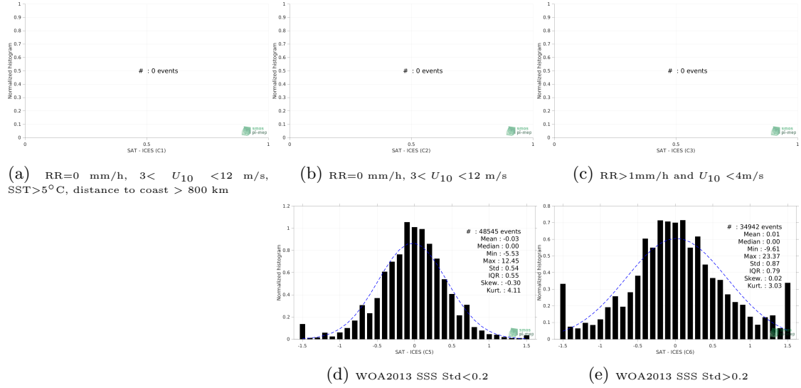
Figure 13: Normalized histogram of \Delta SSS (SMOS SSS L3 Arctic v3.1 - 9 Days (BEC) - ICES) for 5 different subdatasets corresponding to: RR=0 mm/h, 3 < U_{10} < 12 m/s, SST>5°C, distance to coast > 800 km (a), RR=0 mm/h, 3 < U_{10} < 12 m/s (b), RR>1mm/h and U_{10} < 4 m/s (c), WOA2013 SSS Std<0.2 (d), WOA2013 SSS Std>0.2 (e).
