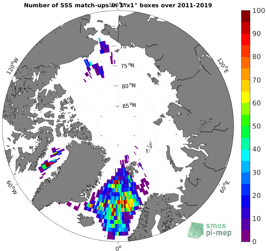
Figure 4: Number of SSS match-ups between Argo SSS and the SMOS SSS L3 Arctic v3.1 - 9 Days (BEC) SSS product for the Arctic Ocean Pi-MEP region over 1^\circ \times 1^\circ boxes and for the full satellite product period.
