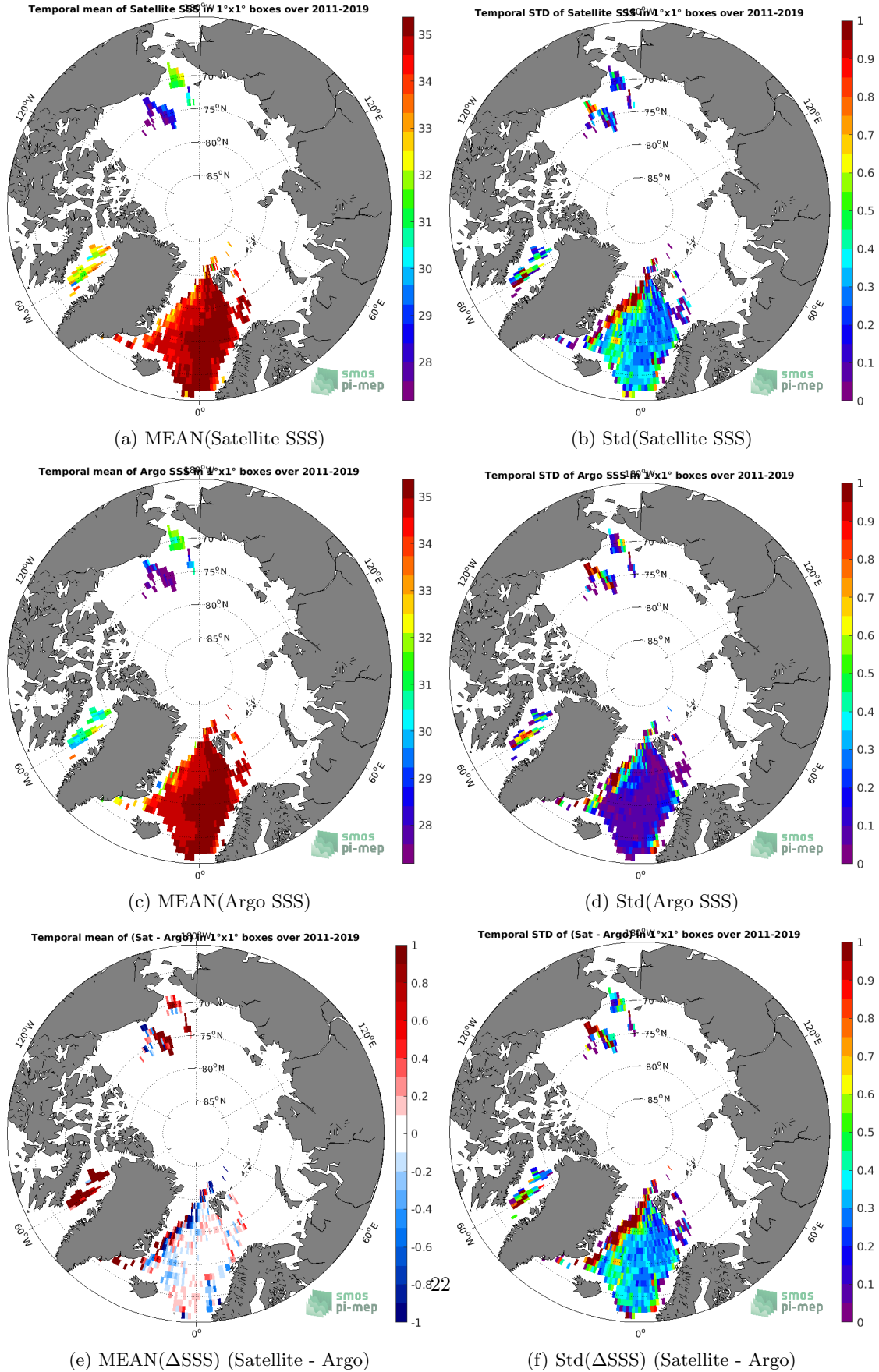
Figure 6: Temporal mean (left) and Std (right) of SSS from SMOS SSS L3 Arctic v3.1 - 9 Days (BEC) (top), Argo (middle), and of \Delta SSS (Satellite - Argo). Only match-up pairs are used to generate these maps.
