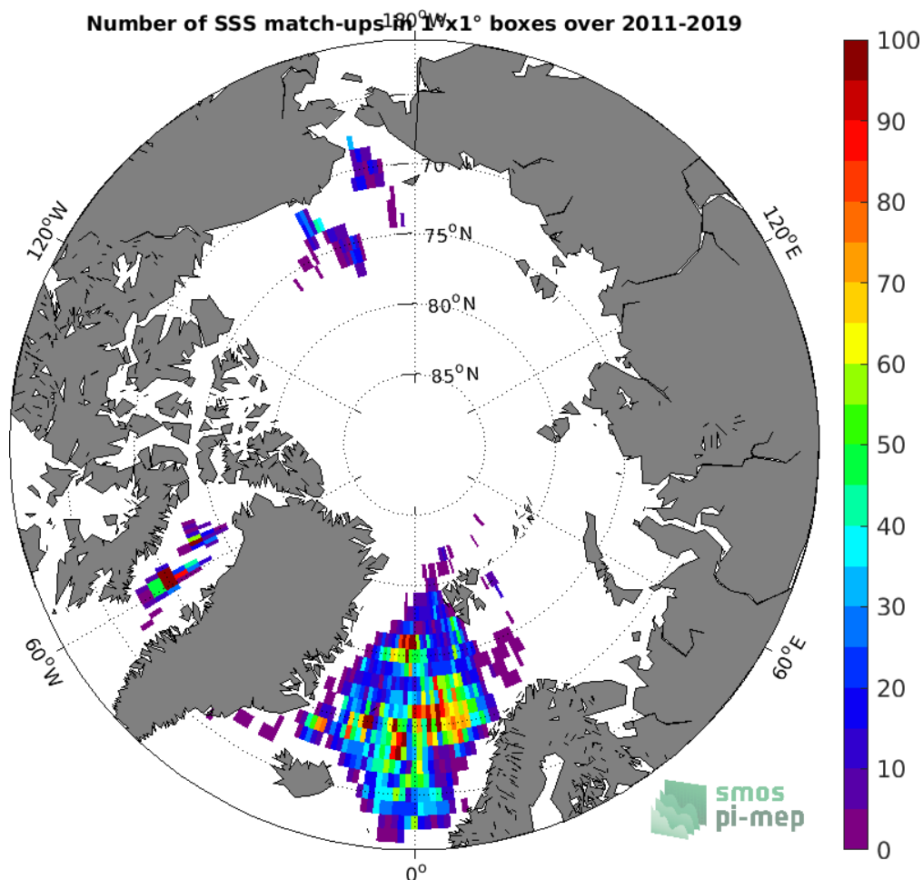
Figure 4: Number of SSS match-ups between Argo SSS and the SMOS SSS L3 Arctic v3.1 - 9 Days (BEC) SSS product for the Arctic Ocean Pi-MEP region over 1°x1° boxes and for the full satellite product period.
