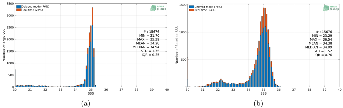
Figure 2: Histograms of SSS from Argo (a) and SMOS SSS L3 Arctic v3.1 - 9 Days (BEC) (b) considering all match-up pairs per bins of 0.1 over the Arctic Ocean Pi-MEP region and for the full satellite product period.
