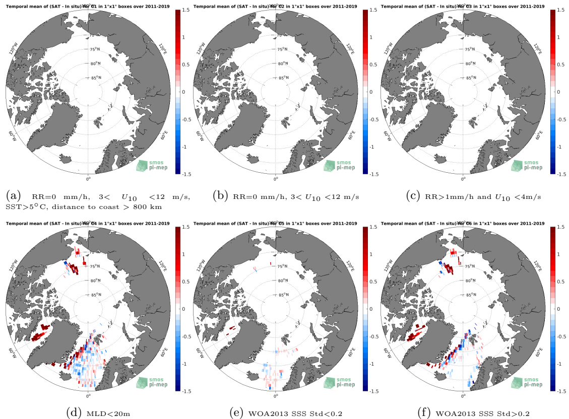
Figure 12: Temporal mean gridded over spatial boxes of size 1^{\circ}\times 1^{\circ} of \Delta\text{SSS} (SMOS SSS L3 Arctic v3.1 - 9 Days (BEC) - Argo) for 6 different subdatasets corresponding to:RR=0 mm/h, 3 < U_{10} < 12 m/s, SST >5^{\circ}\text{C} , distance to coast > 800 km (a), RR=0 mm/h, 3 < U_{10} < 12 m/s (b), RR >1 mm/h and U_{10} < 4 m/s (c),MLD <20 m (d),WOA2013 SSS Std <0.2 (e),WOA2013 SSS Std >0.2 (f).
