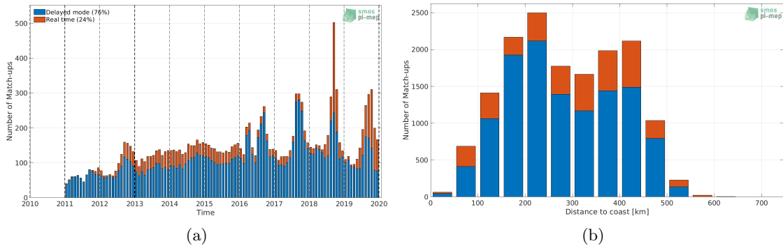
Figure 1: Number of match-ups between Argo and SMOS SSS L3 Arctic v3.1 - 9 Days (BEC) SSS as a function of time (a) and as function of the distance to coast (b) over the Arctic Ocean Pi-MEP region and for the full satellite product period.
