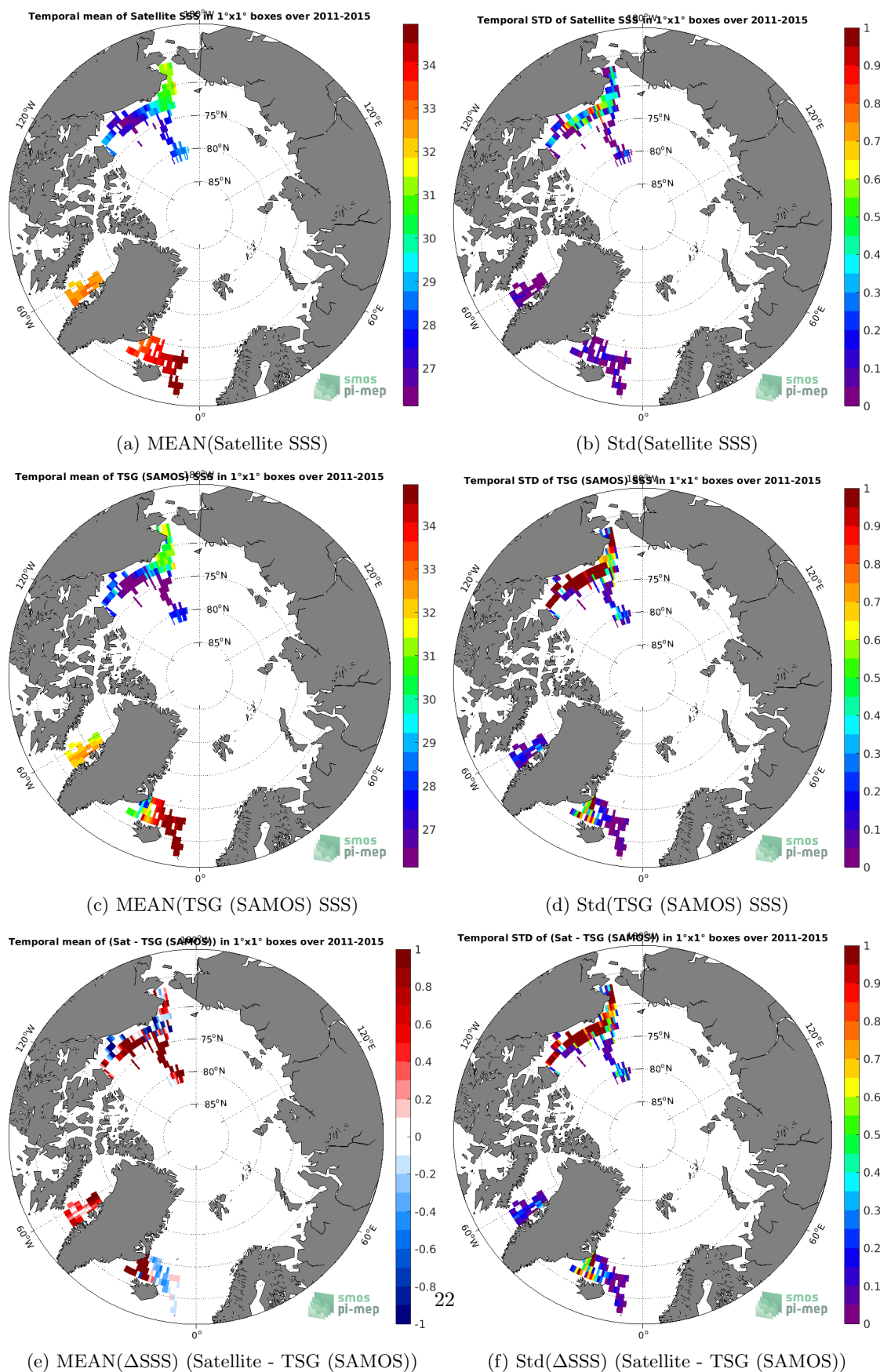
Figure 6: Temporal mean (left) and Std (right) of SSS from SMOS SSS L3 Arctic OA v2 - 9 Days (BEC) (top), TSG (SAMOS) (middle), and of \Delta SSS (Satellite - TSG (SAMOS)). Only match-up pairs are used to generate these maps.
