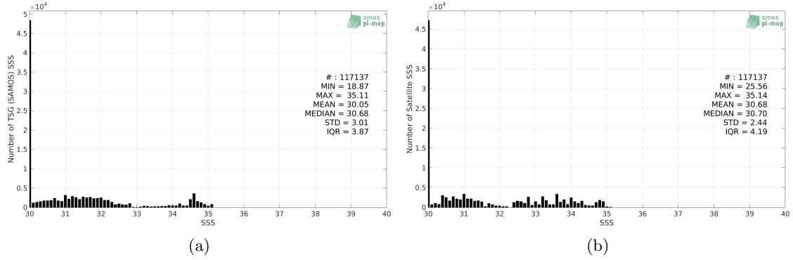
Figure 2: Histograms of SSS from TSG (SAMOS) (a) and SMOS SSS L3 Arctic OA v2 - 9 Days (BEC) (b) considering all match-up pairs per bins of 0.1 over the Arctic Ocean Pi-MEP region and for the full satellite product period.
