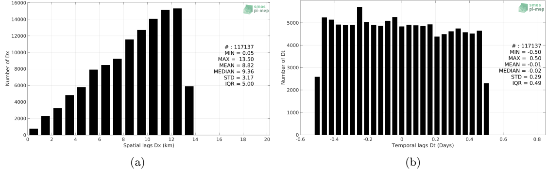
Figure 5: Histograms of the spatial (a) and temporal (b) lags between the time of the TSG (SAMOS) measurements and the date of the corresponding SMOS SSS L3 Arctic OA v2 - 9 Days (BEC) SSS product.
