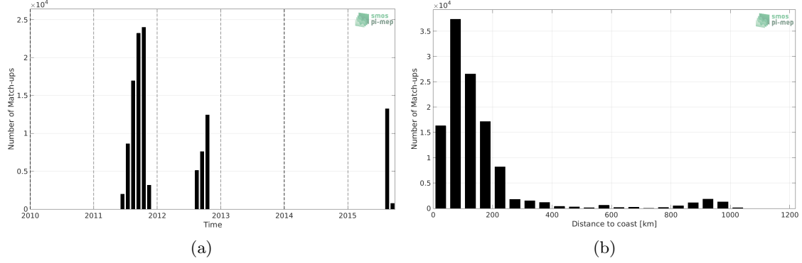
Figure 1: Number of match-ups between TSG (SAMOS) and SMOS SSS L3 Arctic OA v2 - 9 Days (BEC) SSS as a function of time (a) and as function of the distance to coast (b) over the Arctic Ocean Pi-MEP region and for the full satellite product period.
