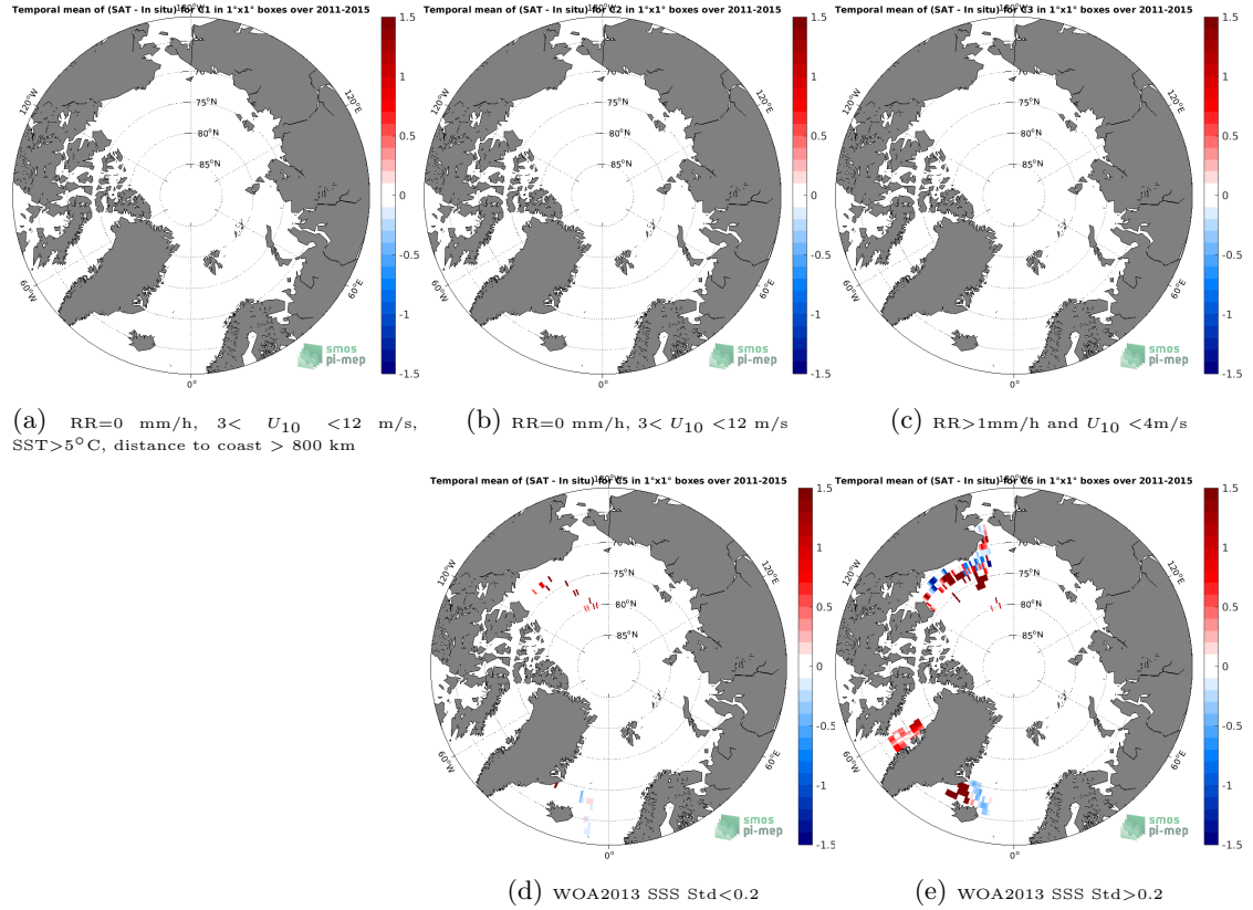
Figure 12: Temporal mean gridded over spatial boxes of size 1^{\circ}\times 1^{\circ} of \Delta\text{SSS} (SMOS SSS L3 Arctic OA v2 - 9 Days (BEC) - TSG (SAMOS)) for 5 different subdatasets corresponding to: RR=0 mm/h, 3 < U_{10} < 12 m/s, SST >5^{\circ}\text{C} , distance to coast > 800 km (a), RR=0 mm/h, 3 < U_{10} < 12 m/s (b), RR >1 mm/h and U_{10} < 4 m/s (c), WOA2013 SSS Std <0.2 (d), WOA2013 SSS Std >0.2 (e).
