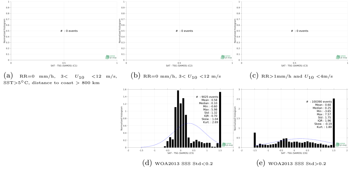
Figure 13: Normalized histogram of \Delta\text{SSS} (SMOS SSS L3 Arctic OA v2 - 9 Days (BEC) - TSG (SAMOS)) for 5 different subdatasets corresponding to: RR=0 mm/h, 3 < U_{10} < 12 m/s, SST > 5^\circ\text{C} , distance to coast > 800 km (a), RR=0 mm/h, 3 < U_{10} < 12 m/s (b), RR > 1 mm/h and U_{10} < 4 m/s (c), WOA2013 SSS Std < 0.2 (d), WOA2013 SSS Std > 0.2 (e).
