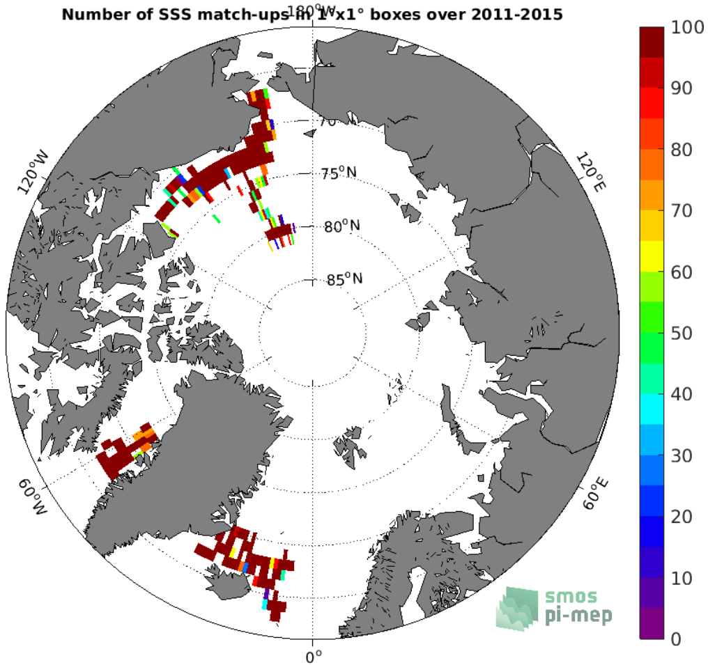
Figure 4: Number of SSS match-ups between TSG (SAMOS) SSS and the SMOS SSS L3 Arctic OA v2 - 9 Days (BEC) SSS product for the Arctic Ocean Pi-MEP region over 1°x1° boxes and for the full satellite product period.
