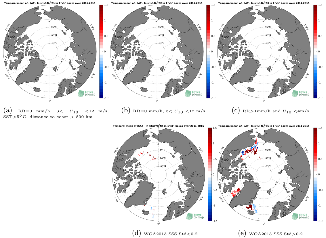
Figure 12: Temporal mean gridded over spatial boxes of size 1^{\circ}\times 1^{\circ} of \Delta\text{SSS} (SMOS L3 Arctic OA v2 - 9 Days (BEC) - TSG-SAMOS) for 5 different subdatasets corresponding to: RR=0 mm/h, 3 < U_{10} < 12 m/s, SST > 5^{\circ}\text{C} , distance to coast > 800 km (a), RR=0 mm/h, 3 < U_{10} < 12 m/s (b), RR > 1 mm/h and U_{10} < 4 m/s (c), WOA2013 SSS Std < 0.2 (d), WOA2013 SSS Std > 0.2 (e).
