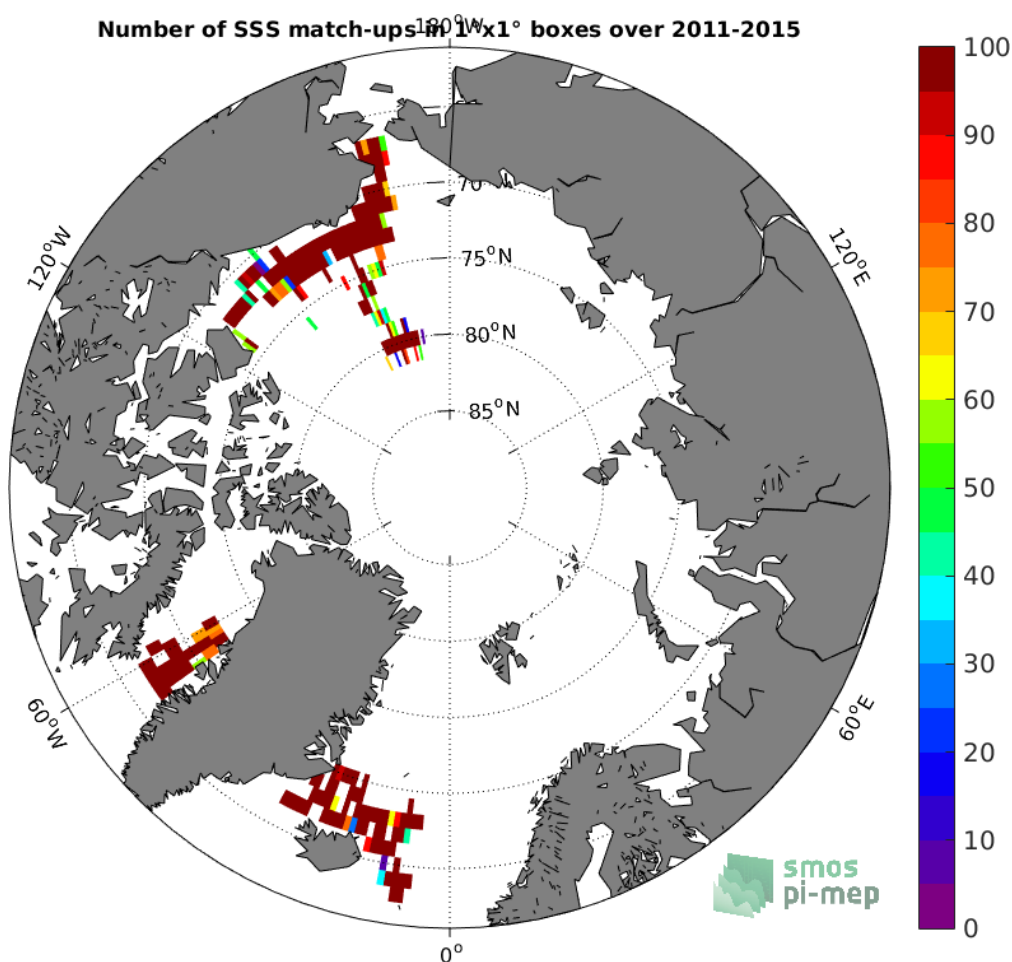
Figure 4: Number of SSS match-ups between TSG-SAMOS SSS and the SMOS L3 Arctic OA v2 - 9 Days (BEC) SSS product for the Arctic Ocean Pi-MEP region over 1^\circ \times 1^\circ boxes and for the full satellite product period.
