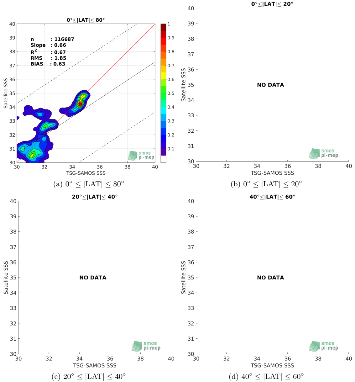
Figure 9: Contour maps of the concentration of SMOS L3 Arctic OA v2 - 9 Days (BEC) SSS (y-axis) versus TSG-SAMOS SSS (x-axis) at match-up pairs for different latitude bands. For each plot, the red line shows x=y . The black thin and dashed lines indicate a linear fit through the cloud and the \pm 95\% confidence levels, respectively. The number match-up pairs n , the slope and R^2 coefficient of the linear fit, the root mean square (RMS) and the mean bias between satellite and in situ data are indicated for each latitude band in each plots.
