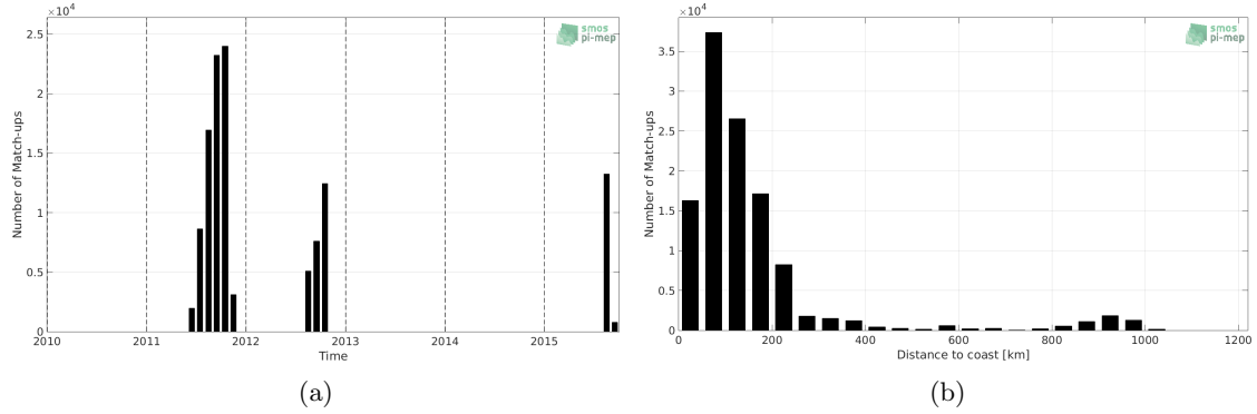
Figure 1: Number of match-ups between TSG-SAMOS and SMOS L3 Arctic OA v2 - 9 Days (BEC) SSS as a function of time (a) and as function of the distance to coast (b) over the Arctic Ocean Pi-MEP region and for the full satellite product period.
