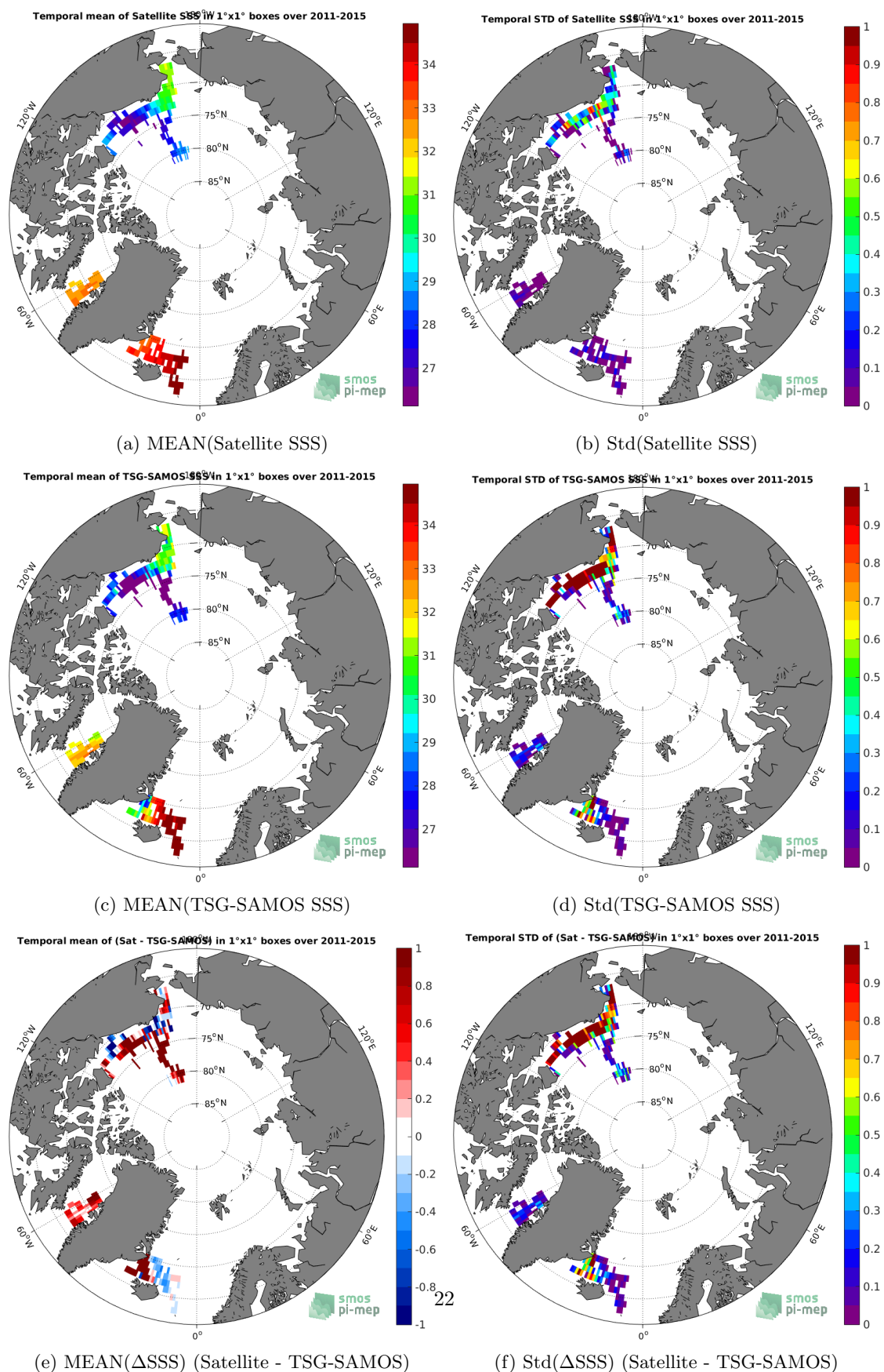
Figure 6: Temporal mean (left) and Std (right) of SSS from SMOS L3 Arctic OA v2 - 9 Days (BEC) (top), TSG-SAMOS (middle), and of \Delta SSS (Satellite - TSG-SAMOS). Only match-up pairs are used to generate these maps.
