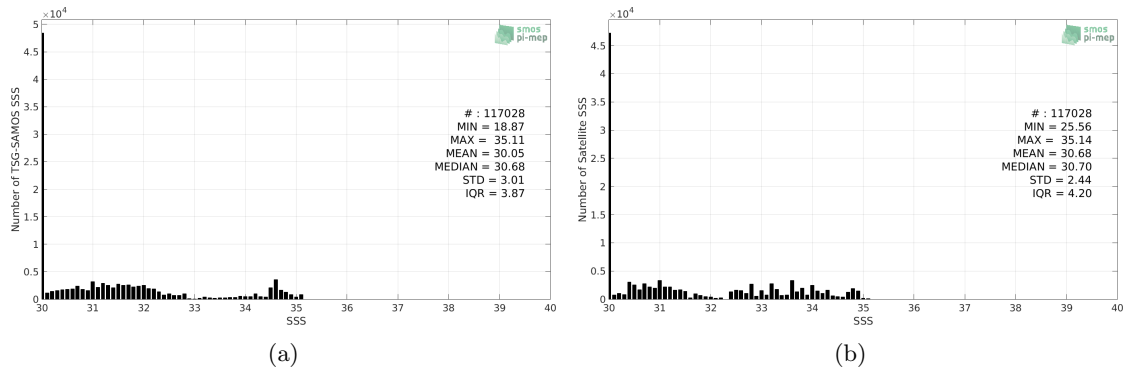
Figure 2: Histograms of SSS from TSG-SAMOS (a) and SMOS L3 Arctic OA v2 - 9 Days (BEC) (b) considering all match-up pairs per bins of 0.1 over the Arctic Ocean Pi-MEP region and for the full satellite product period.
