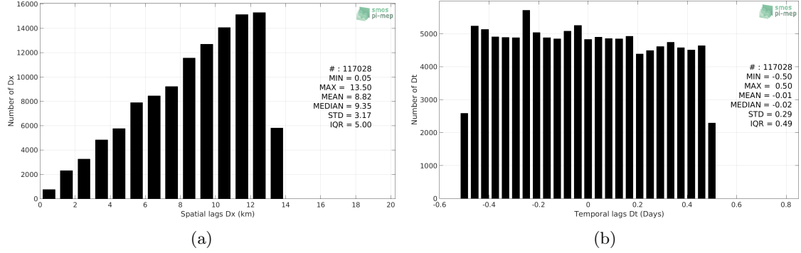
Figure 5: Histograms of the spatial (a) and temporal (b) lags between the time of the TSG-SAMOS measurements and the date of the corresponding SMOS L3 Arctic OA v2 - 9 Days (BEC) SSS product.
