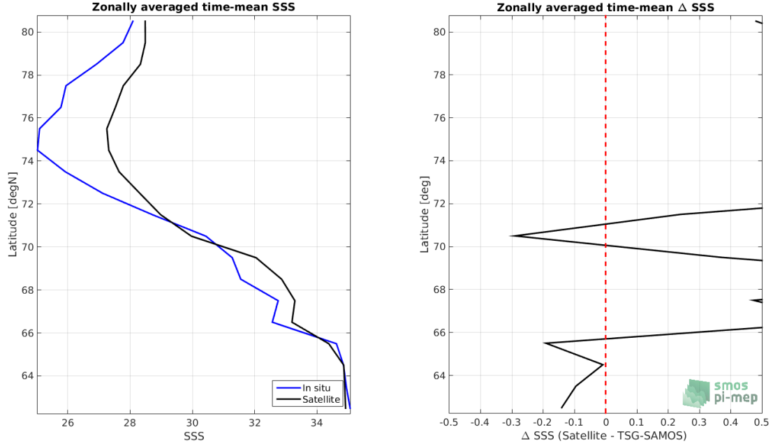
Figure 8: Left panel: Zonal mean SSS from SMOS L3 Arctic OA v2 - 9 Days (BEC) satellite product (black) and from TSG-SAMOS (blue). Right panel: Zonal mean of \Delta SSS (Satellite - TSG-SAMOS) for all the collected Pi-MEP match-up pairs estimated over the full satellite product period.
