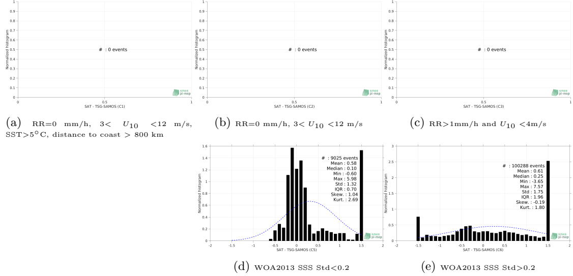
Figure 13: Normalized histogram of \Delta\text{SSS} (SMOS L3 Arctic OA v2 - 9 Days (BEC) - TSG-SAMOS) for 5 different subdatasets corresponding to: RR=0 mm/h, 3 < U_{10} < 12 m/s, SST > 5^{\circ}\text{C} , distance to coast > 800 km (a), RR=0 mm/h, 3 < U_{10} < 12 m/s (b), RR > 1\text{mm/h} and U_{10} < 4\text{m/s} (c), WOA2013 SSS Std < 0.2 (d), WOA2013 SSS Std > 0.2 (e).
