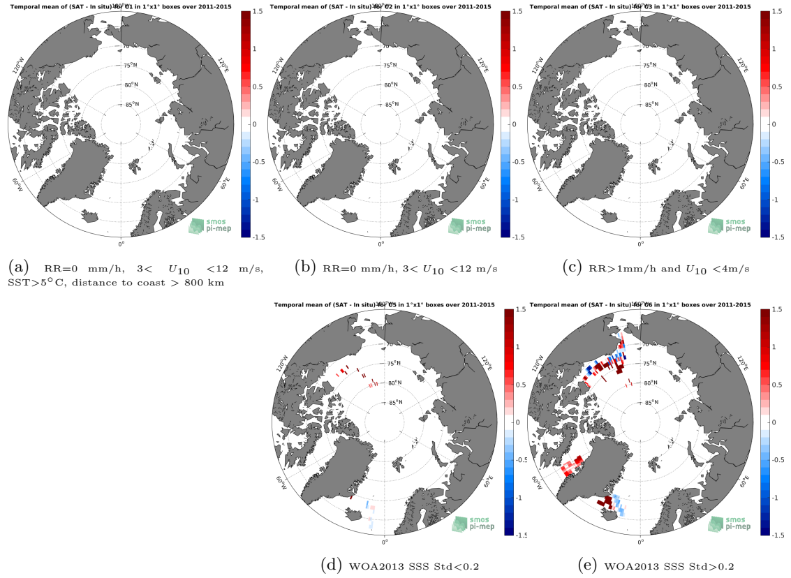
Figure 12: Temporal mean gridded over spatial boxes of size 1^\circ \times 1^\circ of \Delta SSS (SMOS-L3-BEC-ARCTIC-OA-V2-9DAYS-0.25DEG - TSG-SAMOS) for 5 different subdatasets corresponding to: RR=0 mm/h, 3 < U_{10} < 12 m/s, SST >5^\circ\text{C} , distance to coast > 800 km (a), RR=0 mm/h, 3 < U_{10} < 12 m/s (b), RR >1 mm/h and U_{10} < 4 m/s (c), WOA2013 SSS Std <0.2 (d), WOA2013 SSS Std >0.2 (e).
