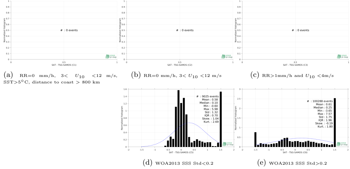
Figure 13: Normalized histogram of \Delta\text{SSS} (SMOS-L3-BEC-ARCTIC-OA-V2-9DAYS-0.25DEG - TSG-SAMOS) for 5 different subdatasets corresponding to: RR=0 mm/h, 3 < U_{10} < 12 m/s, SST > 5^\circ\text{C} , distance to coast > 800 km (a), RR=0 mm/h, 3 < U_{10} < 12 m/s (b), RR > 1\text{mm/h} and U_{10} < 4\text{m/s} (c), WOA2013 SSS Std<0.2 (d), WOA2013 SSS Std>0.2 (e).
