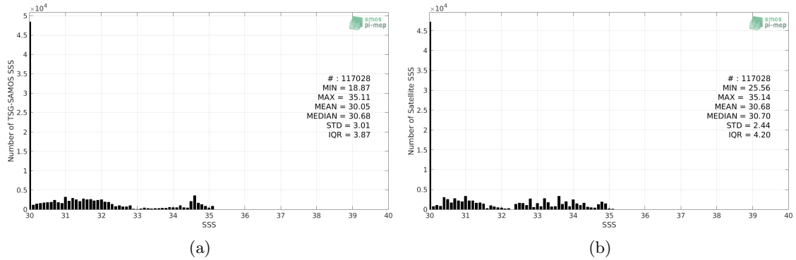
Figure 2: Histograms of SSS from TSG-SAMOS (a) and SMOS-L3-BEC-ARCTIC-OA-V2-9DAYS-0.25DEG (b) considering all match-up pairs per bins of 0.1 over the Arctic Ocean Pi-MEP region and for the full satellite product period.
