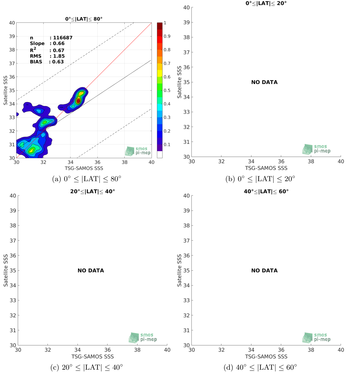
Figure 9: Contour maps of the concentration of SMOS-L3-BEC-ARCTIC-OA-V2-9DAYS-0.25DEG SSS (y-axis) versus TSG-SAMOS SSS (x-axis) at match-up pairs for different latitude bands. For each plot, the red line shows x=y . The black thin and dashed lines indicate a linear fit through the data cloud and the \pm 95\% confidence levels, respectively. The number match-up pairs n , the slope and R^2 coefficient of the linear fit, the root mean square (RMS) and the mean bias between satellite and in situ data are indicated for each latitude band in each plots.
