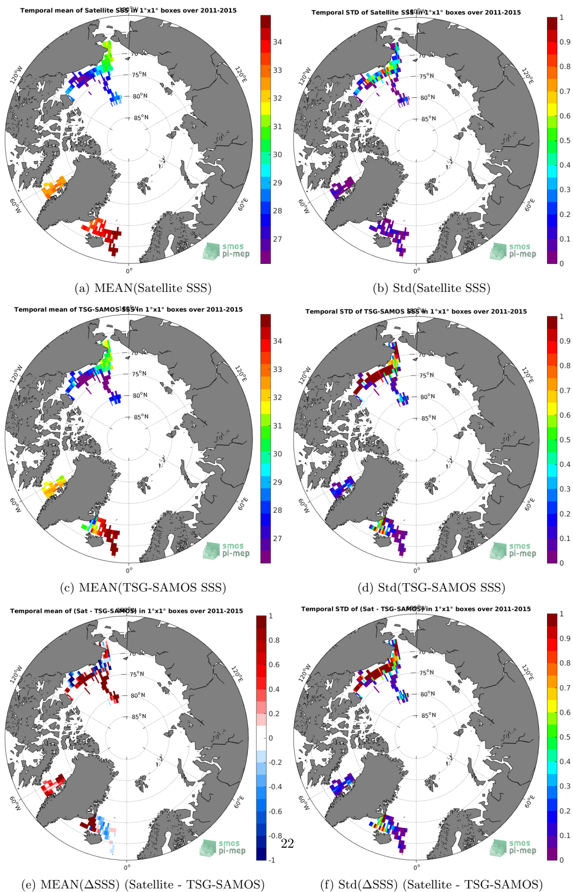
Figure 6: Temporal mean (left) and Std (right) of SSS from SMOS-L3-BEC-ARCTIC-OA-V2-9DAYS-0.25DEG (top), TSG-SAMOS (middle), and of \Delta SSS (Satellite - TSG-SAMOS). Only match-up pairs are used to generate these maps.
