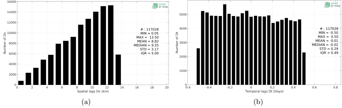
Figure 5: Histograms of the spatial (a) and temporal (b) lags between the time of the TSG-SAMOS measurements and the date of the corresponding SMOS-L3-BEC-ARCTIC-OA-V2-9DAYS-0.25DEG SSS product.
