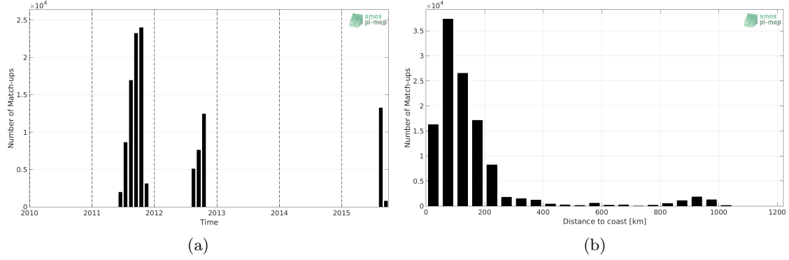
Figure 1: Number of match-ups between TSG-SAMOS and SMOS-L3-BEC-ARCTIC-OA-V2-9DAYS-0.25DEG SSS as a function of time (a) and as function of the distance to coast (b) over the Arctic Ocean Pi-MEP region and for the full satellite product period.
