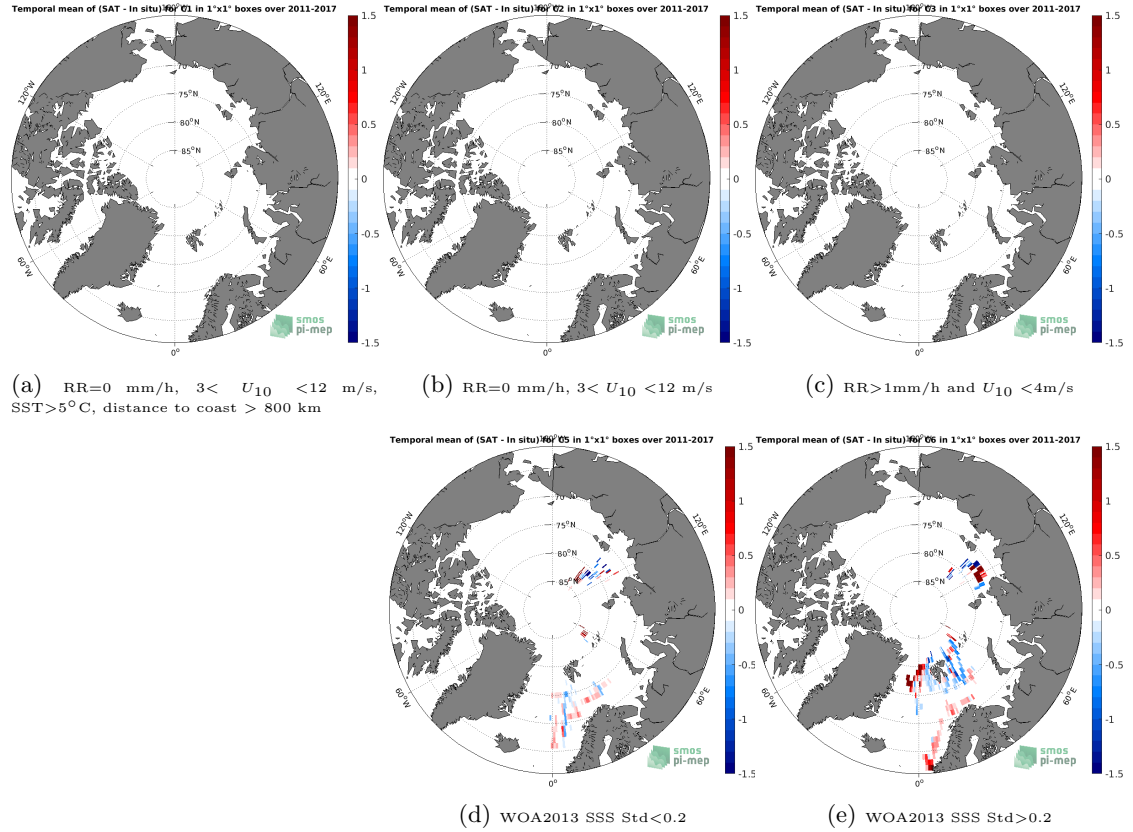
Figure 12: Temporal mean gridded over spatial boxes of size 1^{\circ}\times 1^{\circ} of \Delta\text{SSS} (SMOS SSS L3 Arctic OA v2 - 9 Days (BEC) - TSG (Polarstern)) for 5 different subdatasets corresponding to: RR=0 mm/h, 3 < U_{10} < 12 m/s, SST >5^{\circ}\text{C} , distance to coast > 800 km (a), RR=0 mm/h, 3 < U_{10} < 12 m/s (b), RR >1 mm/h and U_{10} < 4 m/s (c), WOA2013 SSS Std <0.2 (d), WOA2013 SSS Std >0.2 (e).
