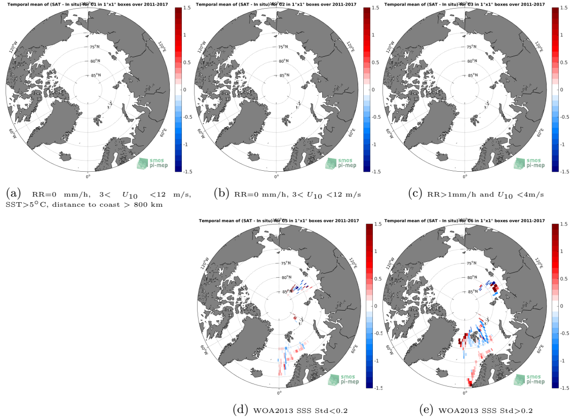
Figure 12: Temporal mean gridded over spatial boxes of size 1^{\circ}\times 1^{\circ} of \Delta\text{SSS} (SMOS L3 Arctic OA v2 - 9 Days (BEC) - TSG-POLARSTERN) for 5 different subdatasets corresponding to: RR=0 mm/h, 3 < U_{10} < 12 m/s, SST > 5^{\circ}\text{C} , distance to coast > 800 km (a), RR=0 mm/h, 3 < U_{10} < 12 m/s (b), RR > 1 mm/h and U_{10} < 4 m/s (c), WOA2013 SSS Std < 0.2 (d), WOA2013 SSS Std > 0.2 (e).
