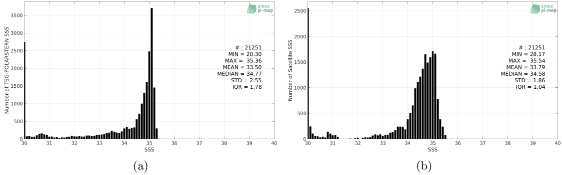
Figure 2: Histograms of SSS from TSG-POLARSTERN (a) and SMOS L3 Arctic OA v2 - 9 Days (BEC) (b) considering all match-up pairs per bins of 0.1 over the Arctic Ocean Pi-MEP region and for the full satellite product period.
