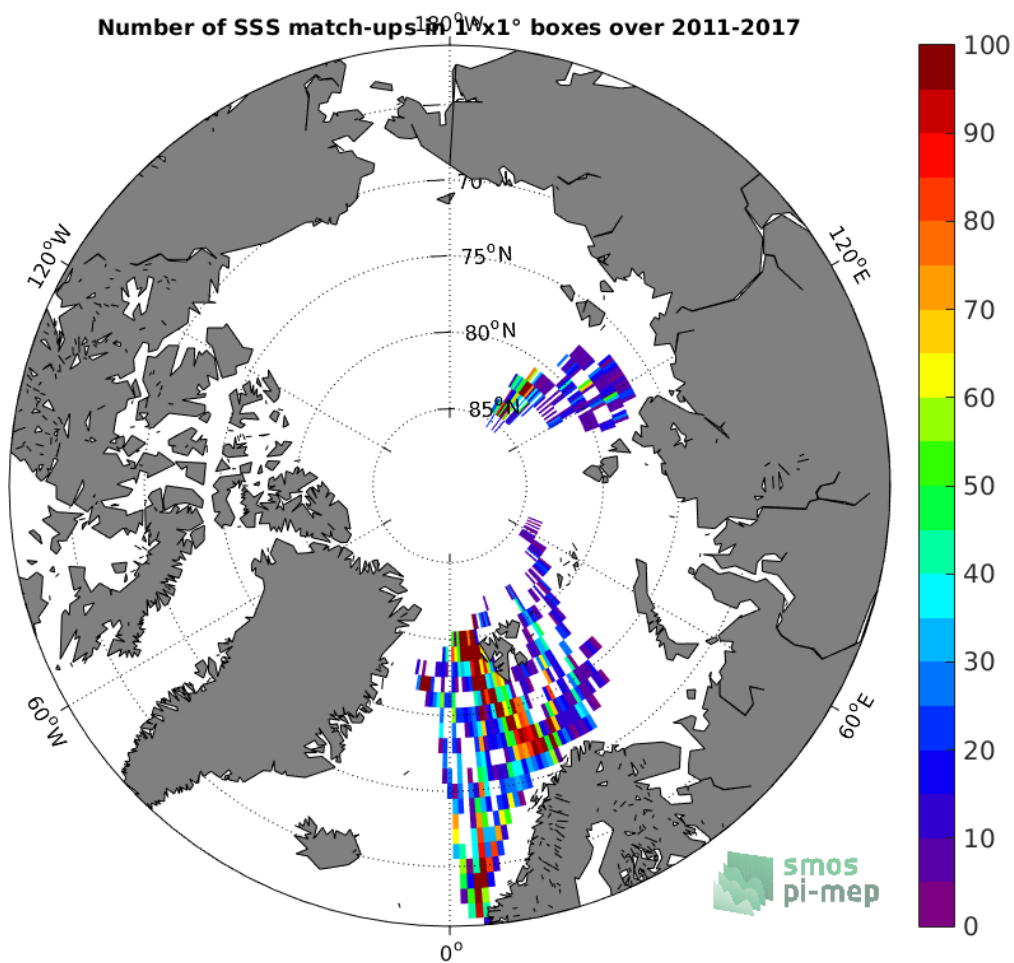
Figure 4: Number of SSS match-ups between TSG-POLARSTERN SSS and the SMOS L3 Arctic OA v2 - 9 Days (BEC) SSS product for the Arctic Ocean Pi-MEP region over 1°x1° boxes and for the full satellite product period.
