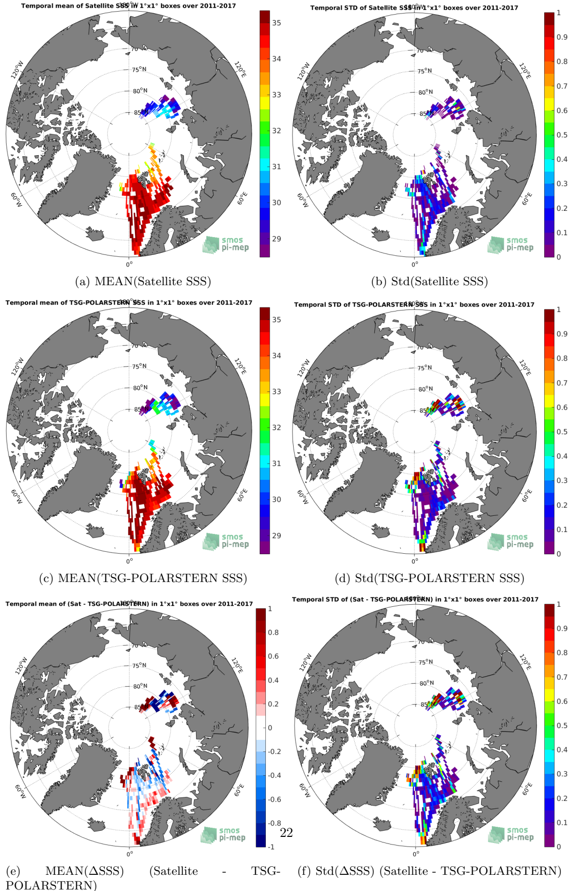
Figure 6: Temporal mean (left) and Std (right) of SSS from SMOS L3 Arctic OA v2 - 9 Days (BEC) (top), TSG-POLARSTERN (middle), and of \Delta SSS (Satellite - TSG-POLARSTERN). Only match-up pairs are used to generate these maps.
