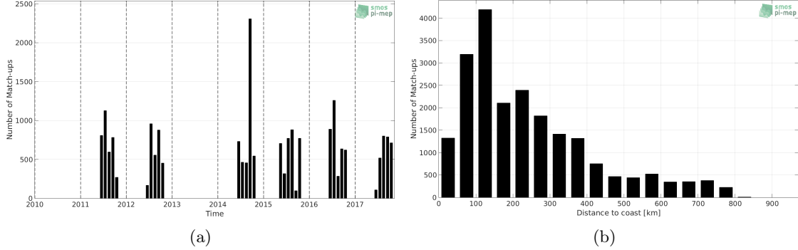
Figure 1: Number of match-ups between TSG-POLARSTERN and SMOS L3 Arctic OA v2 - 9 Days (BEC) SSS as a function of time (a) and as function of the distance to coast (b) over the Arctic Ocean Pi-MEP region and for the full satellite product period.
