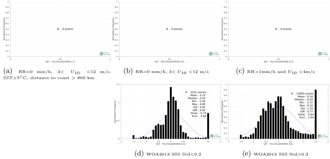
Figure 13: Normalized histogram of \Delta\text{SSS} (SMOS L3 Arctic OA v2 - 9 Days (BEC) - TSG-POLARSTERN) for 5 different subdatasets corresponding to: RR=0 mm/h, 3 < U_{10} < 12 m/s, SST >5^{\circ}\text{C} , distance to coast > 800 km (a), RR=0 mm/h, 3 < U_{10} < 12 m/s (b), RR>1\text{mm/h} and U_{10} < 4\text{m/s} (c), WOA2013 SSS Std <0.2 (d), WOA2013 SSS Std >0.2 (e).
