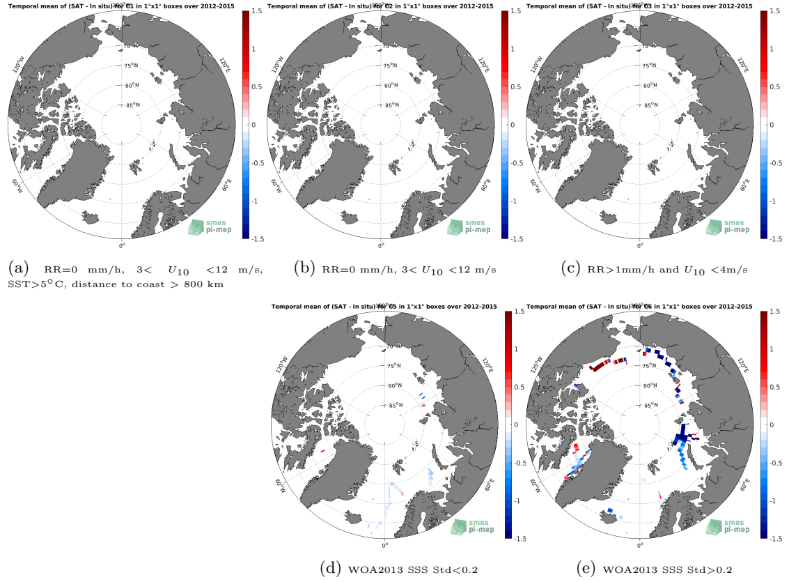
Figure 12: Temporal mean gridded over spatial boxes of size 1^\circ \times 1^\circ of \Delta SSS (SMOS SSS L3 Arctic OA v2 - 9 Days (BEC) - TSG (GOSUD-Sailing-ship)) for 5 different subdatasets corresponding to: RR=0 mm/h, 3 < U_{10} < 12 m/s, SST>5°C, distance to coast > 800 km (a), RR=0 mm/h, 3 < U_{10} < 12 m/s (b), RR>1mm/h and U_{10} < 4 m/s (c), WOA2013 SSS Std<0.2 (d), WOA2013 SSS Std>0.2 (e).
