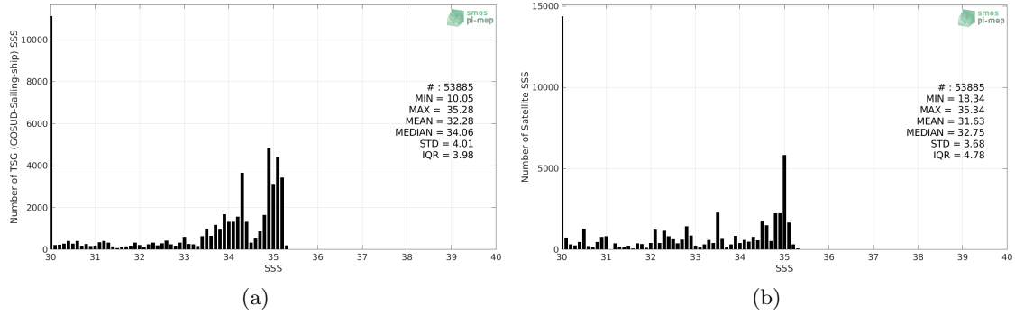
Figure 2: Histograms of SSS from TSG (GOSUD-Sailing-ship) (a) and SMOS SSS L3 Arctic OA v2 - 9 Days (BEC) (b) considering all match-up pairs per bins of 0.1 over the Arctic Ocean Pi-MEP region and for the full satellite product period.
