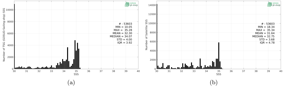
Figure 2: Histograms of SSS from TSG (GOSUD-Sailing-ship) (a) and SMOS SSS L3 Arctic OA v2 - 9 Days (BEC) (b) considering all match-up pairs per bins of 0.1 over the Arctic Ocean Pi-MEP region and for the full satellite product period.
