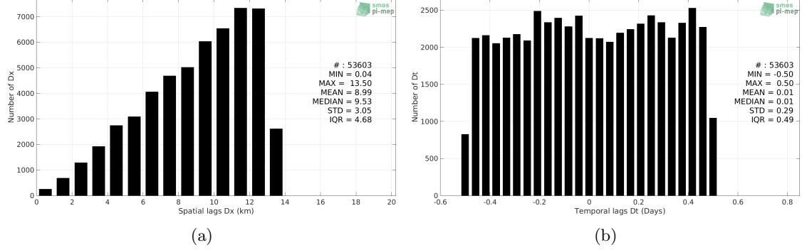
Figure 5: Histograms of the spatial (a) and temporal (b) lags between the time of the TSG (GOSUD-Sailing-ship) measurements and the date of the corresponding SMOS SSS L3 Arctic OA v2 - 9 Days (BEC) SSS product.
