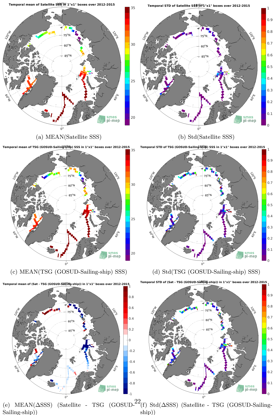
Figure 6: Temporal mean (left) and Std (right) of SSS from SMOS SSS L3 Arctic OA v2 - 9 Days (BEC) (top), TSG (GOSUD-Sailing-ship) (middle), and of \Delta SSS (Satellite - TSG (GOSUD-Sailing-ship)). Only match-up pairs are used to generate these maps.
