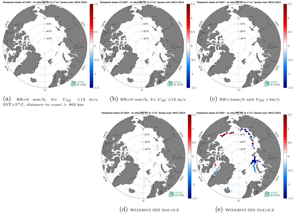
Figure 12: Temporal mean gridded over spatial boxes of size 1^\circ \times 1^\circ of \Delta\text{SSS} (SMOS SSS L3 Arctic OA v2 - 9 Days (BEC) - TSG (GOSUD-Sailing-ship)) for 5 different subdatasets corresponding to: RR=0 mm/h, 3 < U_{10} < 12 m/s, SST > 5^\circ\text{C} , distance to coast > 800 km (a), RR=0 mm/h, 3 < U_{10} < 12 m/s (b), RR > 1 mm/h and U_{10} < 4 m/s (c), WOA2013 SSS Std < 0.2 (d), WOA2013 SSS Std > 0.2 (e).
