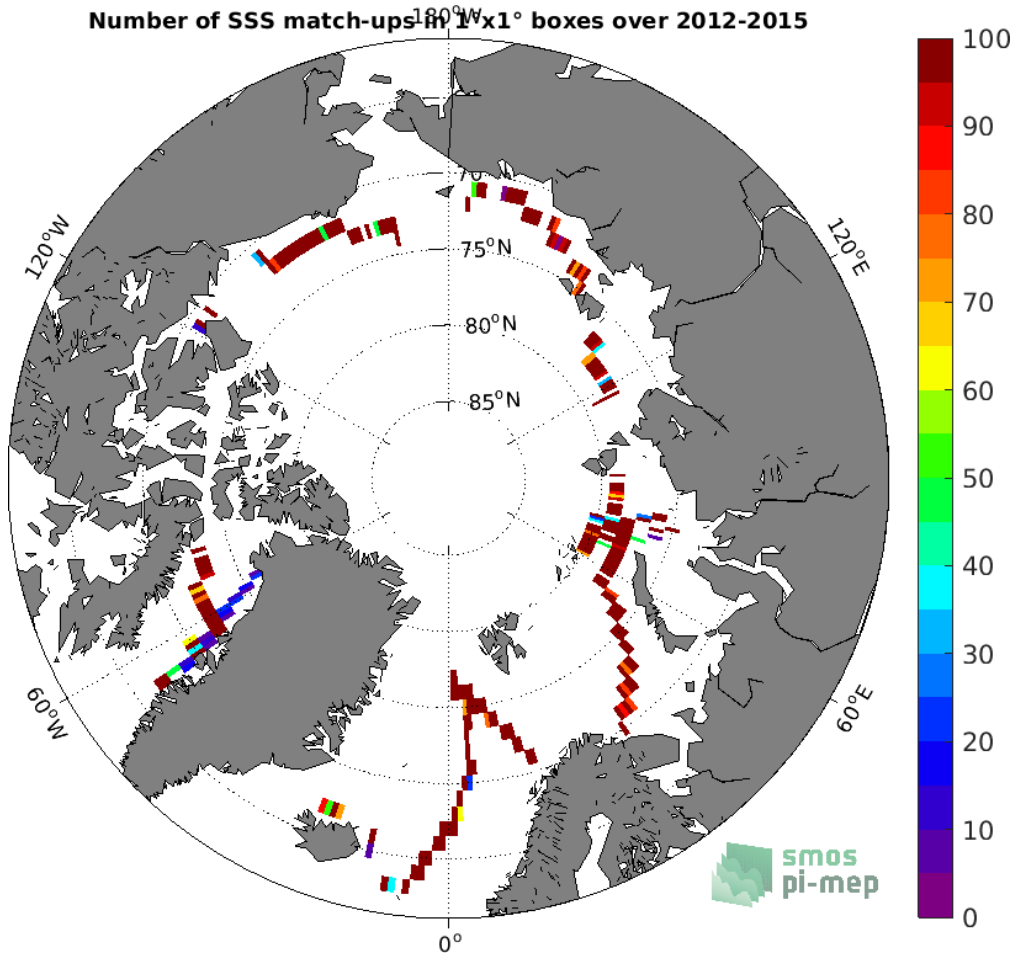
Figure 4: Number of SSS match-ups between TSG (GOSUD-Sailing-ship) SSS and the SMOS SSS L3 Arctic OA v2 - 9 Days (BEC) SSS product for the Arctic Ocean Pi-MEP region over 1^\circ \times 1^\circ boxes and for the full satellite product period.
