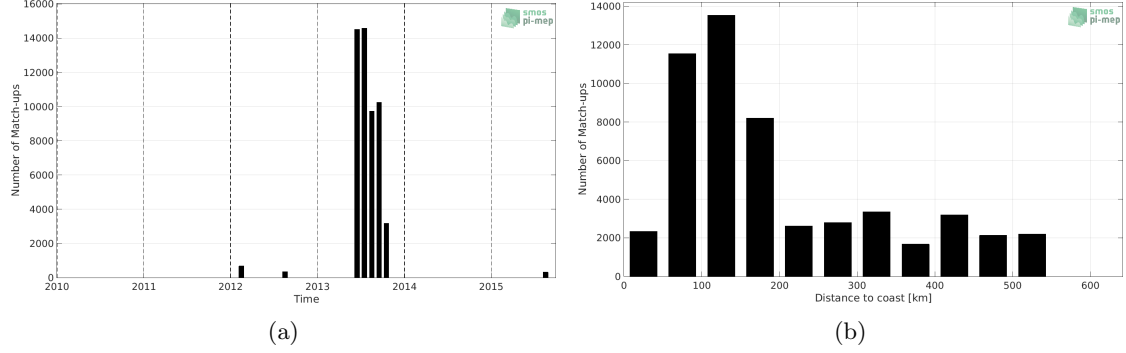
Figure 1: Number of match-ups between TSG (GOSUD-Sailing-ship) and SMOS SSS L3 Arctic OA v2 - 9 Days (BEC) SSS as a function of time (a) and as function of the distance to coast (b) over the Arctic Ocean Pi-MEP region and for the full satellite product period.
