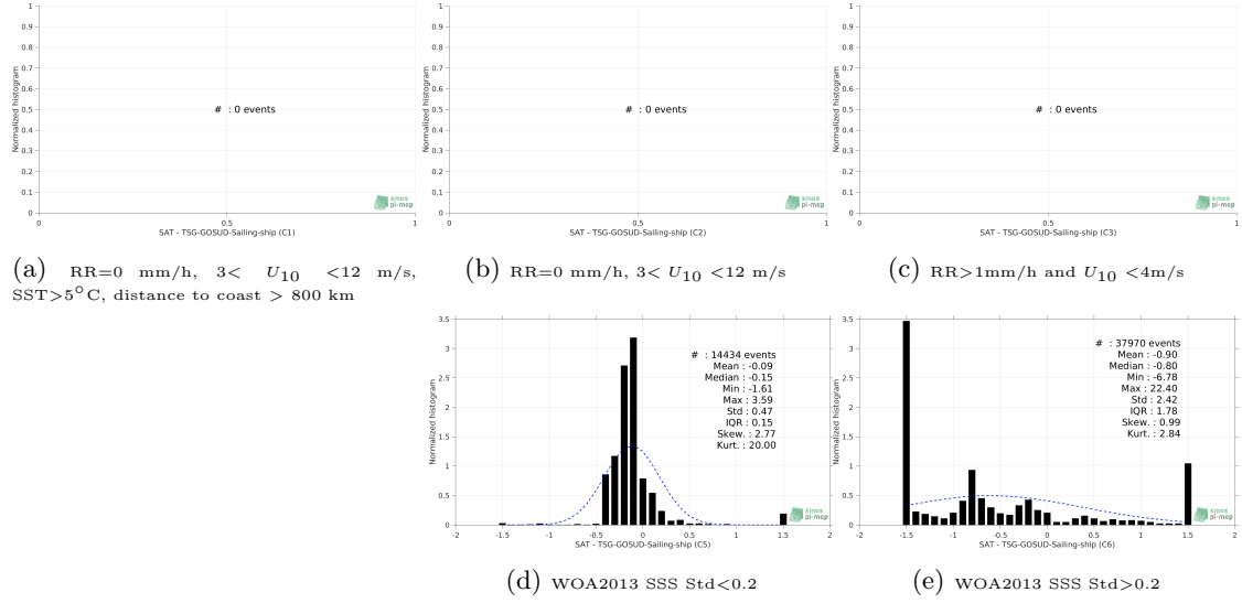
Figure 13: Normalized histogram of \Delta\text{SSS} (SMOS-L3-BEC-ARCTIC-OA-V2-9DAYS-0.25DEG - TSG-GOSUD-Sailing-ship) for 5 different subdatasets corresponding to: RR=0 mm/h, 3 < U_{10} < 12 m/s, SST > 5^{\circ}\text{C} , distance to coast > 800 km (a), RR=0 mm/h, 3 < U_{10} < 12 m/s (b), RR > 1\text{mm/h} and U_{10} < 4\text{m/s} (c), WOA2013 SSS Std<0.2 (d), WOA2013 SSS Std>0.2 (e).
