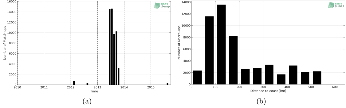
Figure 1: Number of match-ups between TSG-GOSUD-Sailing-ship and SMOS-L3-BEC-ARCTIC-OA-V2-9DAYS-0.25DEG SSS as a function of time (a) and as function of the distance to coast (b) over the Arctic Ocean Pi-MEP region and for the full satellite product period.
