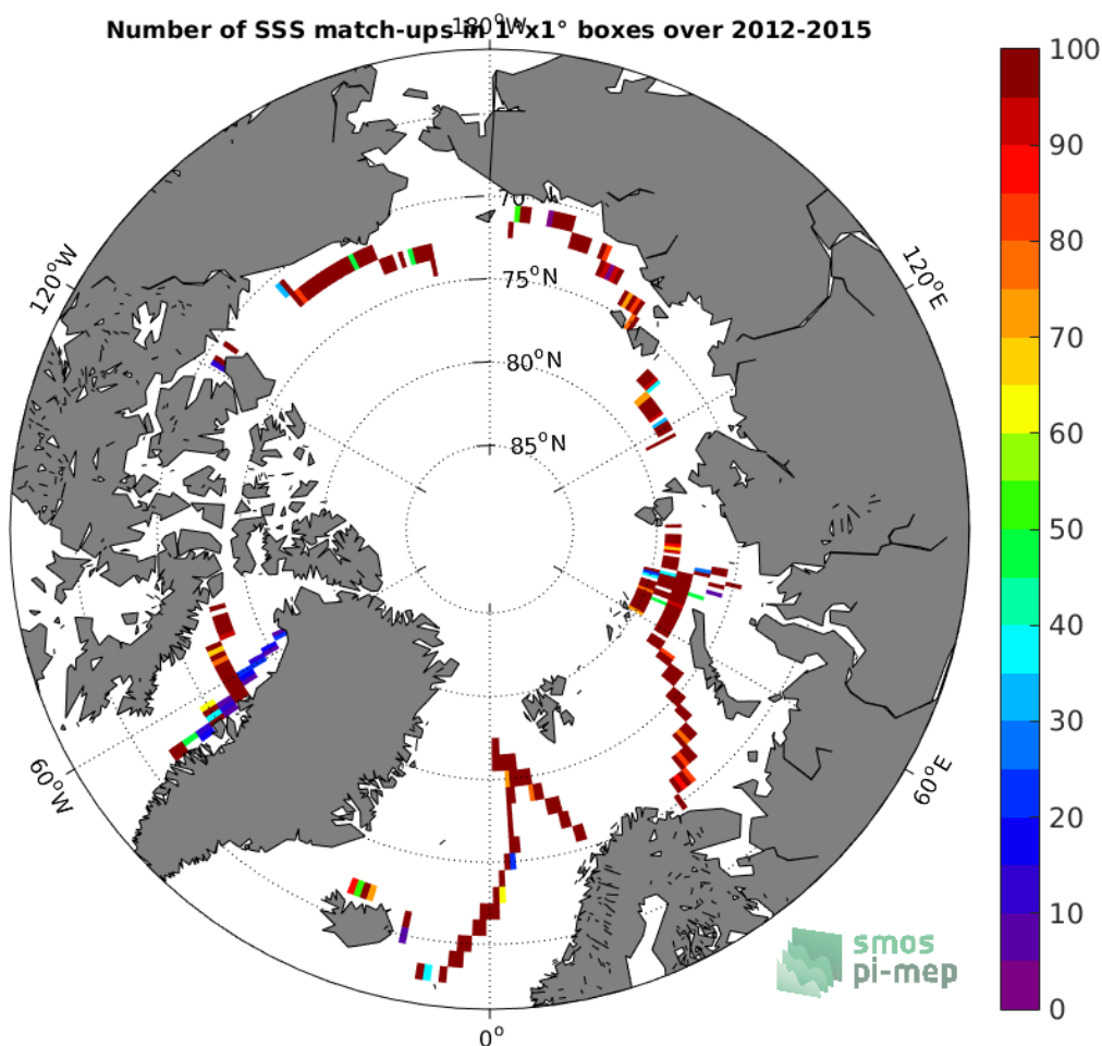
Figure 4: Number of SSS match-ups between TSG-GOSUD-Sailing-ship SSS and the SMOS-L3-BEC-ARCTIC-OA-V2-9DAYS-0.25DEG SSS product for the Arctic Ocean Pi-MEP region over 1^\circ \times 1^\circ boxes and for the full satellite product period.
