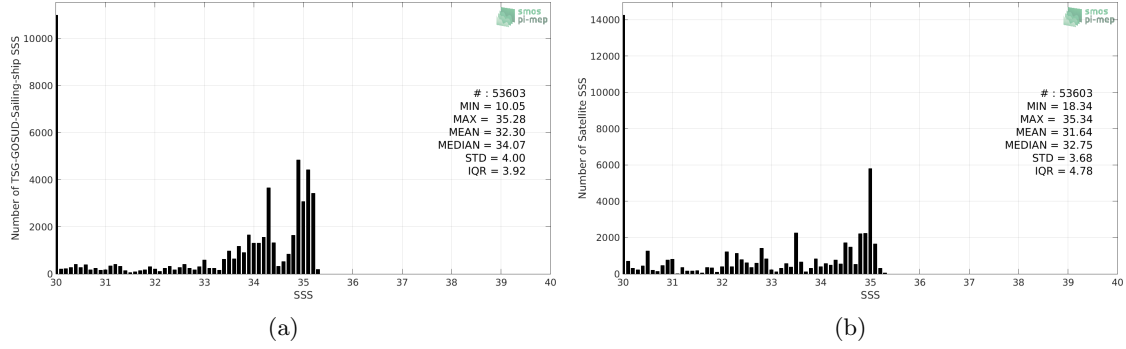
Figure 2: Histograms of SSS from TSG-GOSUD-Sailing-ship (a) and SMOS-L3-BEC-ARCTIC-OA-V2-9DAYS-0.25DEG (b) considering all match-up pairs per bins of 0.1 over the Arctic Ocean Pi-MEP region and for the full satellite product period.
