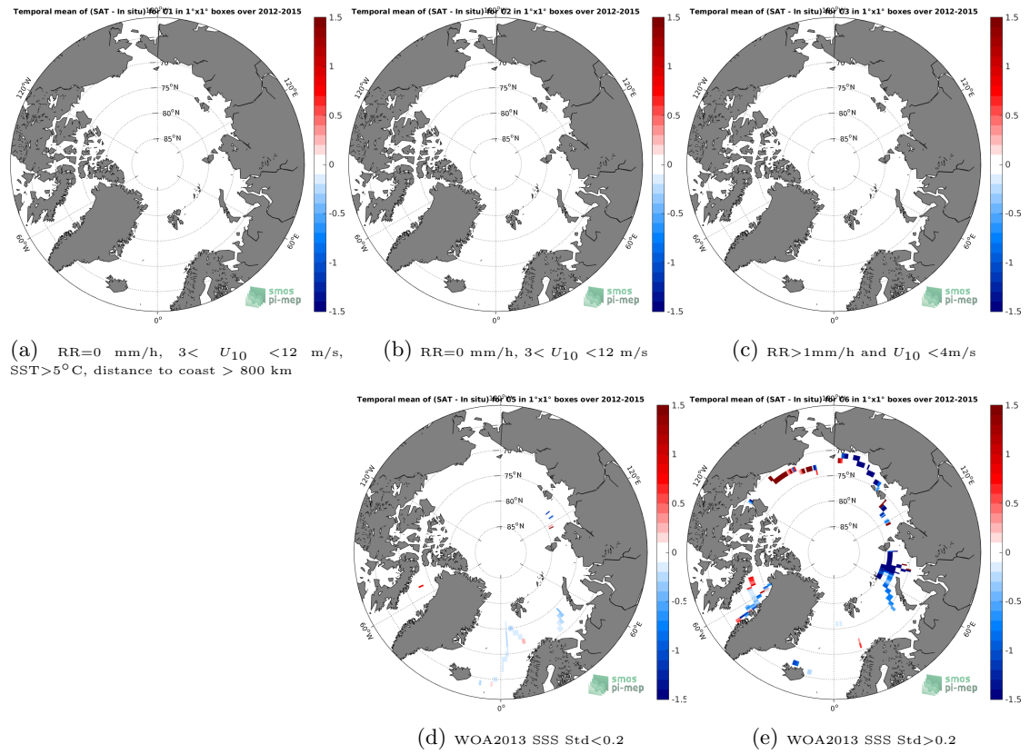
Figure 12: Temporal mean gridded over spatial boxes of size 1^\circ \times 1^\circ of \Delta SSS (SMOS-L3-BEC-ARCTIC-OA-V2-9DAYS-0.25DEG - TSG-GOSUD-Sailing-ship) for 5 different subdatasets corresponding to: RR=0 mm/h, 3 < U_{10} < 12 m/s, SST >5^\circ\text{C} , distance to coast > 800 km (a), RR=0 mm/h, 3 < U_{10} < 12 m/s (b), RR >1 mm/h and U_{10} < 4 m/s (c), WOA2013 SSS Std <0.2 (d), WOA2013 SSS Std >0.2 (e).
