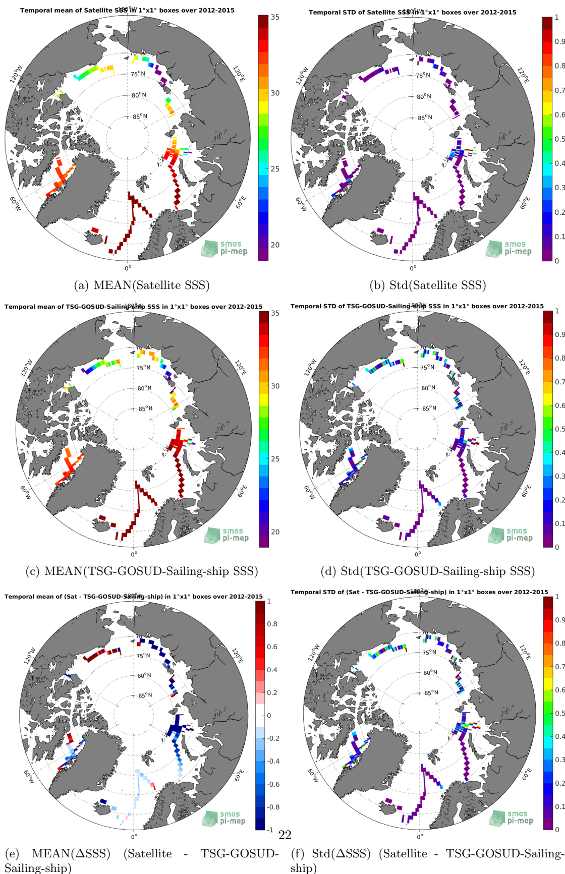
Figure 6: Temporal mean (left) and Std (right) of SSS from SMOS-L3-BEC-ARCTIC-OA-V2-9DAYS-0.25DEG (top), TSG-GOSUD-Sailing-ship (middle), and of \Delta SSS (Satellite - TSG-GOSUD-Sailing-ship). Only match-up pairs are used to generate these maps.
