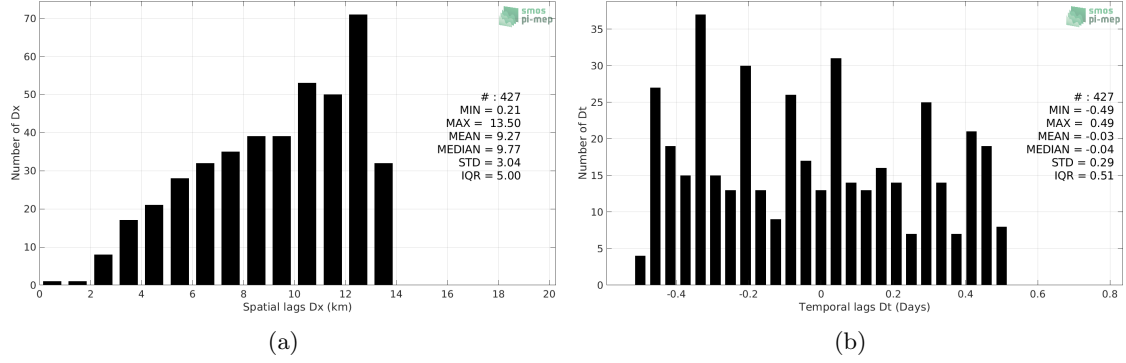
Figure 5: Histograms of the spatial (a) and temporal (b) lags between the location/time of the Marine mammals measurement and the date of the corresponding SMOS SSS L3 Arctic OA v2 - 9 Days (BEC) SSS pixel.
