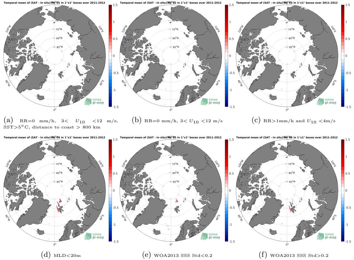
Figure 12: Temporal mean gridded over spatial boxes of size 1^{\circ} \times 1^{\circ} of \Delta\text{SSS} (SMOS SSS L3 Arctic OA v2 - 9 Days (BEC) - Marine mammals) for 6 different subdatasets corresponding to: RR=0 mm/h, 3 < U_{10} < 12 m/s, SST > 5^{\circ}\text{C} , distance to coast > 800 km (a), RR=0 mm/h, 3 < U_{10} < 12 m/s (b), RR > 1 mm/h and U_{10} < 4 m/s (c), MLD < 20 m (d), WOA2013 SSS Std < 0.2 (e), WOA2013 SSS Std > 0.2 (f).
