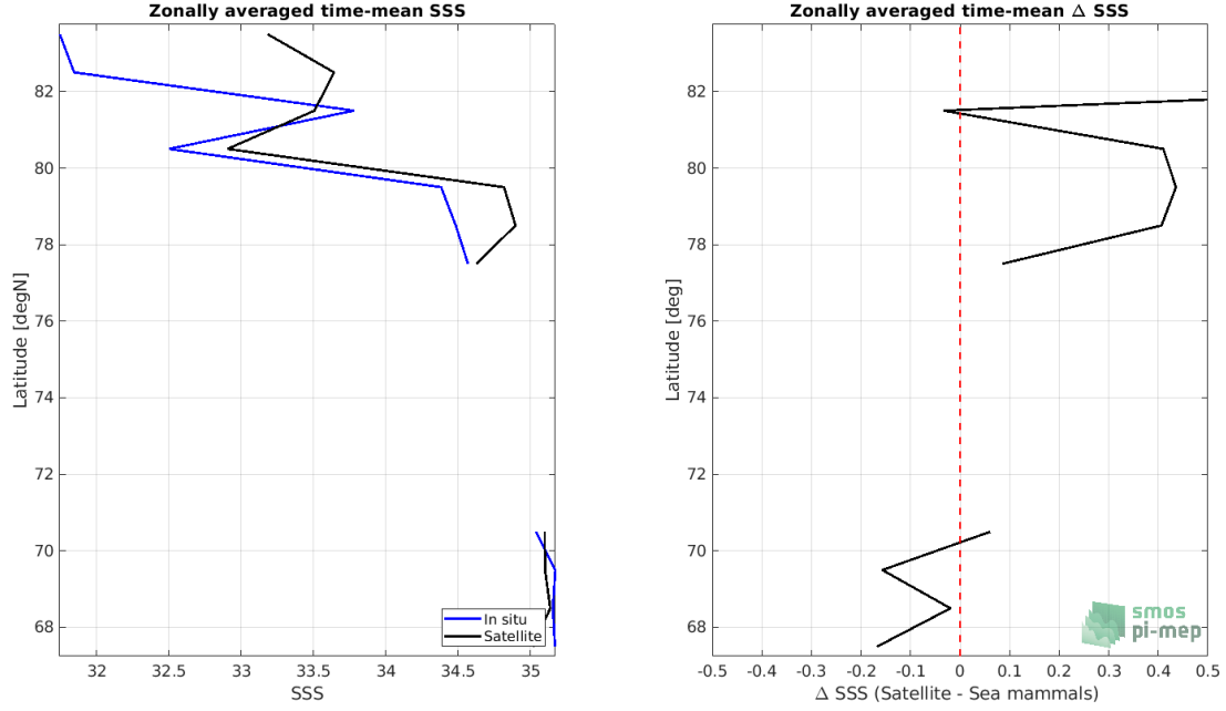
Figure 8: Left panel: Zonal mean SSS from SMOS SSS L3 Arctic OA v2 - 9 Days (BEC) satellite product (black) and from Marine mammals (blue). Right panel: Zonal mean of \Delta SSS (Satellite - Marine mammals) for all the collected Pi-MEP match-up pairs estimated over the full satellite product period.
