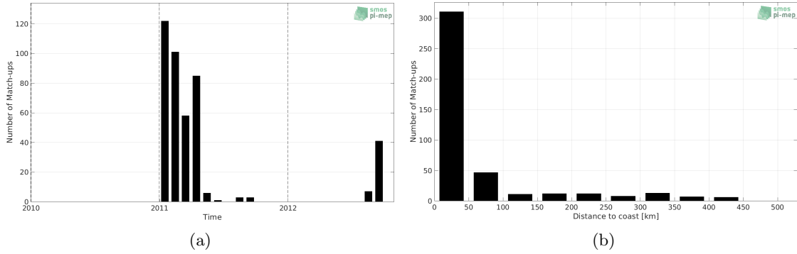
Figure 1: Number of match-ups between Marine mammals and SMOS SSS L3 Arctic OA v2 - 9 Days (BEC) SSS as a function of time (a) and as function of the distance to coast (b) over the Arctic Ocean Pi-MEP region and for the full satellite product period.
