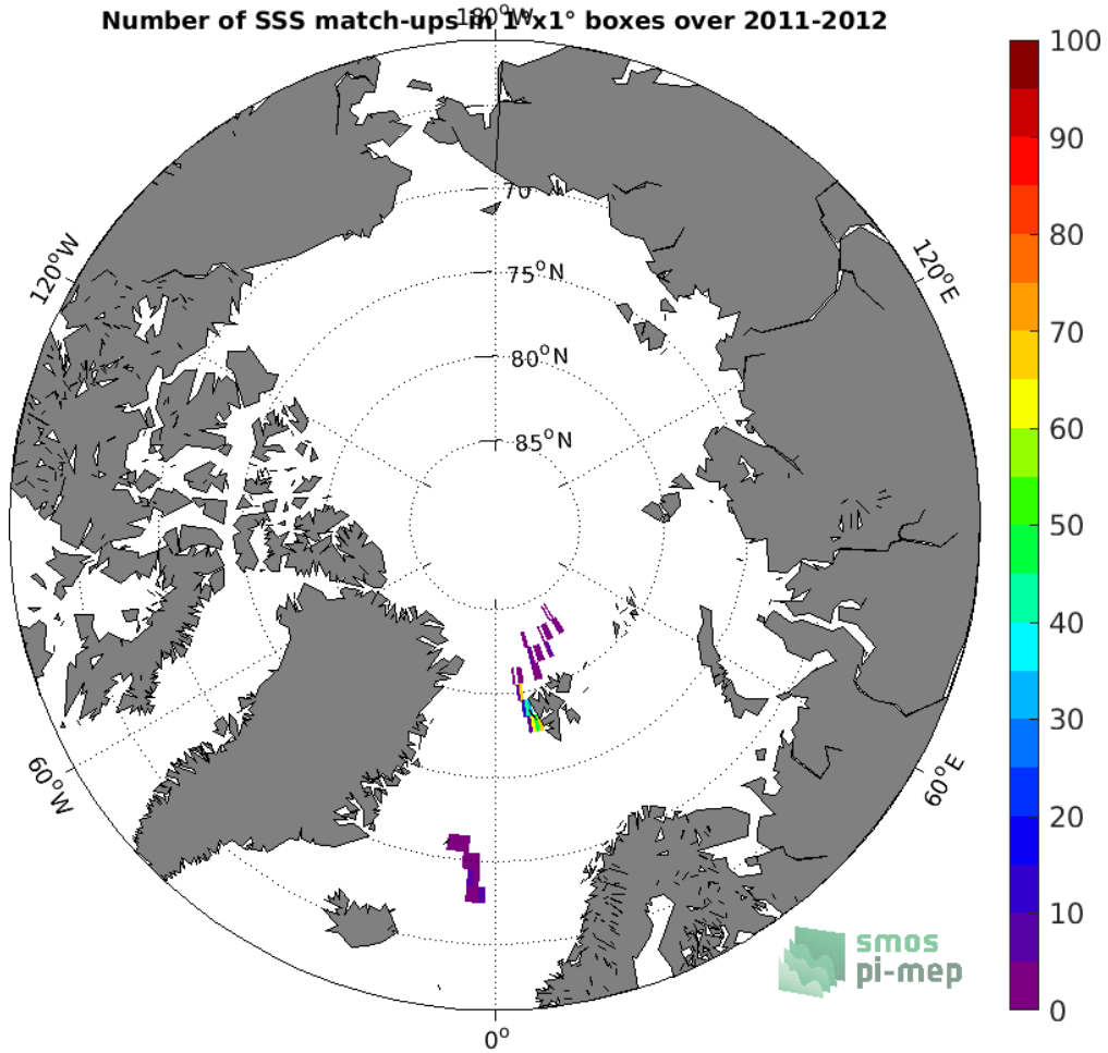
Figure 4: Number of SSS match-ups between Marine mammals SSS and the SMOS SSS L3 Arctic OA v2 - 9 Days (BEC) SSS product for the Arctic Ocean Pi-MEP region over 1^\circ \times 1^\circ boxes and for the full satellite product period.
