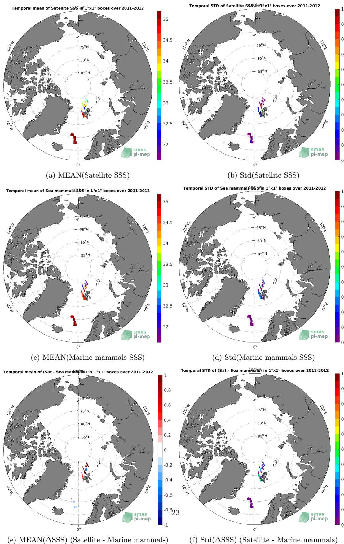
Figure 6: Temporal mean (left) and Std (right) of SSS from SMOS SSS L3 Arctic OA v2 - 9 Days (BEC) (top), Marine mammals (middle), and of \Delta SSS (Satellite - Marine mammals). Only match-up pairs are used to generate these maps.
