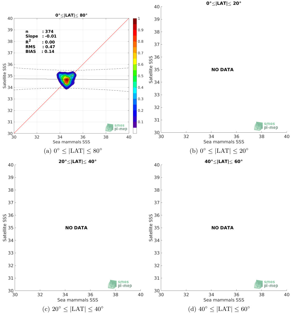
Figure 9: Contour maps of the concentration of SMOS SSS L3 Arctic OA v2 - 9 Days (BEC) SSS (y-axis) versus Marine mammals SSS (x-axis) at match-up pairs for different latitude bands. For each plot, the red line shows x=y . The black thin and dashed lines indicate a linear fit through the data cloud and the \pm 95\% confidence levels, respectively. The number match-up pairs n , the slope and R^2 coefficient of the linear fit, the root mean square (RMS) and the mean bias between satellite and in situ data are indicated for each latitude band in each plots.
