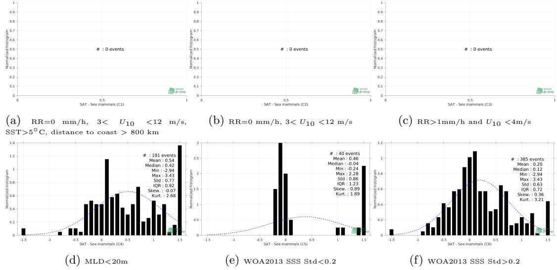
Figure 13: Normalized histogram of \Delta SSS (SMOS SSS L3 Arctic OA v2 - 9 Days (BEC) - Marine mammals) for 6 different subdatasets corresponding to: RR=0 mm/h, 3 < U_{10} < 12 m/s, SST>5°C, distance to coast > 800 km (a), RR=0 mm/h, 3 < U_{10} < 12 m/s (b), RR>1mm/h and U_{10} < 4 m/s (c), MLD<20m (d), WOA2013 SSS Std<0.2 (e), WOA2013 SSS Std>0.2 (f).
