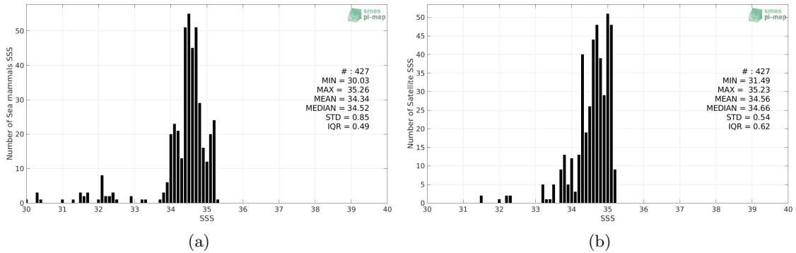
Figure 2: Histograms of SSS from Marine mammals (a) and SMOS SSS L3 Arctic OA v2 - 9 Days (BEC) (b) considering all match-up pairs per bins of 0.1 over the Arctic Ocean Pi-MEP region and for the full satellite product period.
