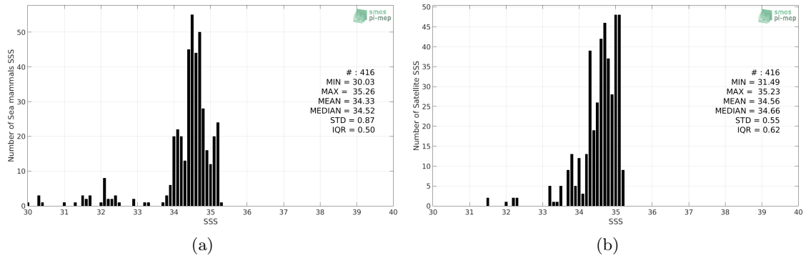
Figure 2: Histograms of SSS from Sea mammals (a) and SMOS L3 Arctic OA v2 - 9 Days (BEC) (b) considering all match-up pairs per bins of 0.1 over the Arctic Ocean Pi-MEP region and for the full satellite product period.
