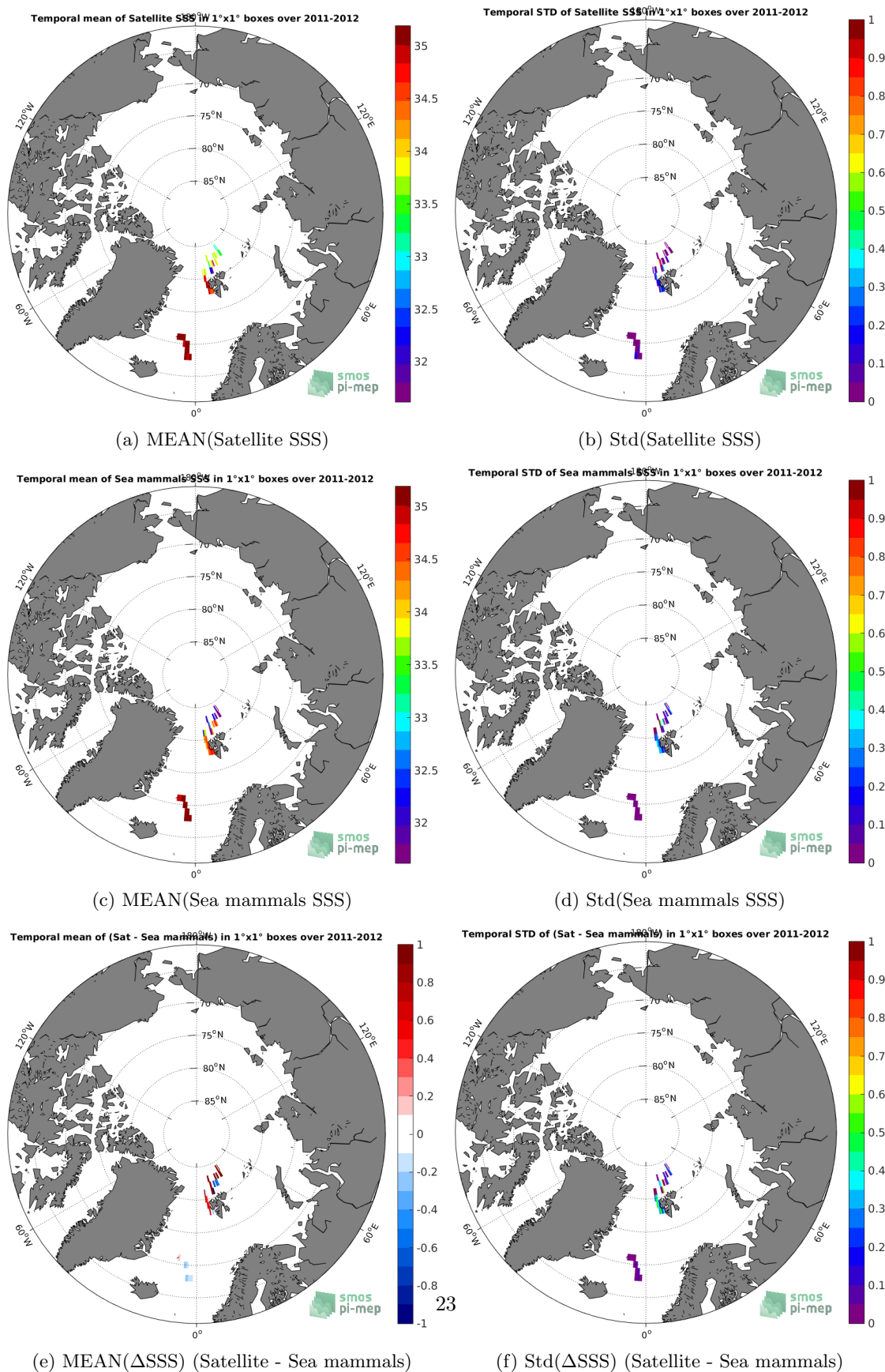
Figure 6: Temporal mean (left) and Std (right) of SSS from SMOS L3 Arctic OA v2 - 9 Days (BEC) (top), Sea mammals (middle), and of \Delta SSS (Satellite - Sea mammals). Only match-up pairs are used to generate these maps.
