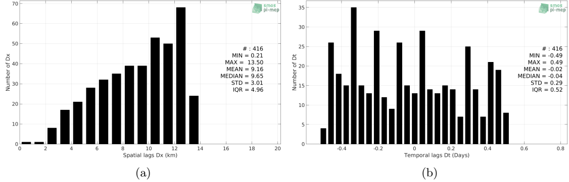
Figure 5: Histograms of the spatial (a) and temporal (b) lags between the time of the Sea mammals measurements and the date of the corresponding SMOS L3 Arctic OA v2 - 9 Days (BEC) SSS product.
