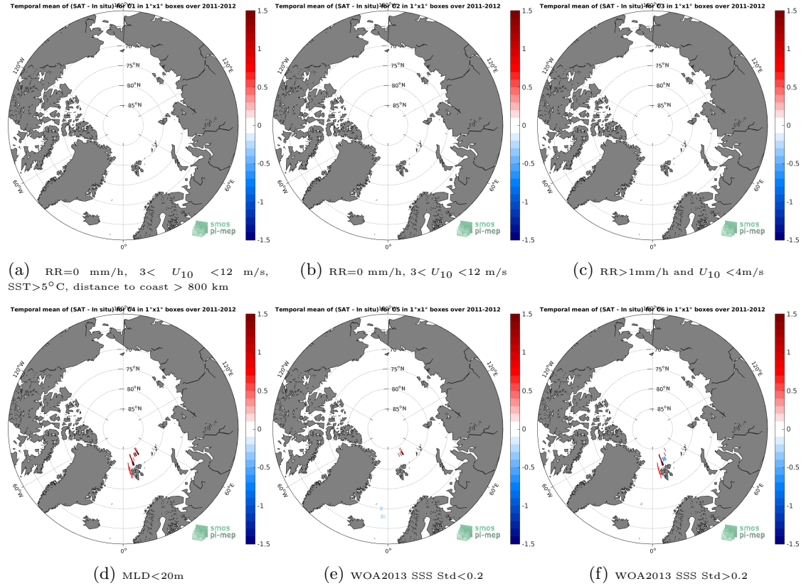
Figure 12: Temporal mean gridded over spatial boxes of size 1^{\circ}\times 1^{\circ} of \Delta\text{SSS} (SMOS L3 Arctic OA v2 - 9 Days (BEC) - Sea mammals) for 6 different subdatasets corresponding to:RR=0 mm/h, 3 < U_{10} < 12 m/s, SST >5^{\circ}\text{C} , distance to coast > 800 km (a), RR=0 mm/h, 3 < U_{10} < 12 m/s (b), RR >1 mm/h and U_{10} < 4 m/s (c),MLD <20 m (d),WOA2013 SSS Std <0.2 (e),WOA2013 SSS Std >0.2 (f).
