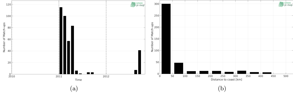
Figure 1: Number of match-ups between Sea mammals and SMOS L3 Arctic OA v2 - 9 Days (BEC) SSS as a function of time (a) and as function of the distance to coast (b) over the Arctic Ocean Pi-MEP region and for the full satellite product period.
