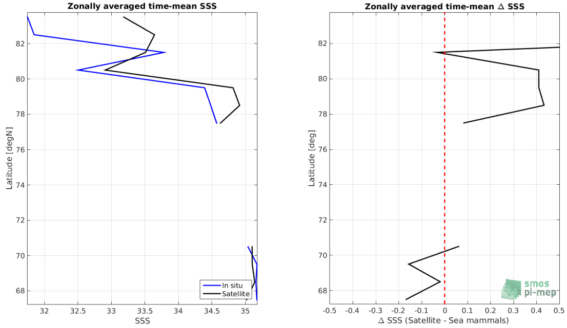
Figure 8: Left panel: Zonal mean SSS from SMOS L3 Arctic OA v2 - 9 Days (BEC) satellite product (black) and from Sea mammals (blue). Right panel: Zonal mean of \Delta SSS (Satellite - Sea mammals) for all the collected Pi-MEP match-up pairs estimated over the full satellite product period.
