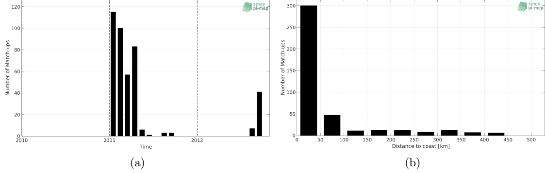
Figure 1: Number of match-ups between Sea mammals and SMOS-L3-BEC-ARCTIC-OA-V2-9DAYS-0.25DEG SSS as a function of time (a) and as function of the distance to coast (b) over the Arctic Ocean Pi-MEP region and for the full satellite product period.
