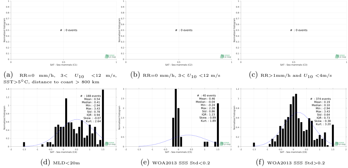
Figure 13: Normalized histogram of \Delta SSS (SMOS-L3-BEC-ARCTIC-OA-V2-9DAYS-0.25DEG - Sea mammals) for 6 different subdatasets corresponding to: RR=0 mm/h, 3 < U_{10} < 12 m/s, SST > 5^\circ\text{C} , distance to coast > 800 km (a), RR=0 mm/h, 3 < U_{10} < 12 m/s (b), RR > 1\text{mm/h} and U_{10} < 4\text{m/s} (c), MLD < 20\text{m} (d), WOA2013 SSS Std < 0.2 (e), WOA2013 SSS Std > 0.2 (f).
