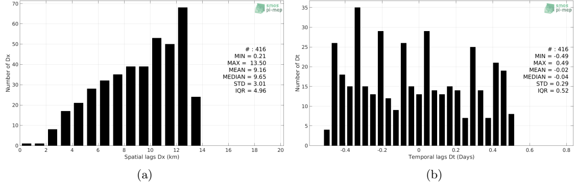
Figure 5: Histograms of the spatial (a) and temporal (b) lags between the time of the Sea mammals measurements and the date of the corresponding SMOS-L3-BEC-ARCTIC-OA-V2-9DAYS-0.25DEG SSS product.
