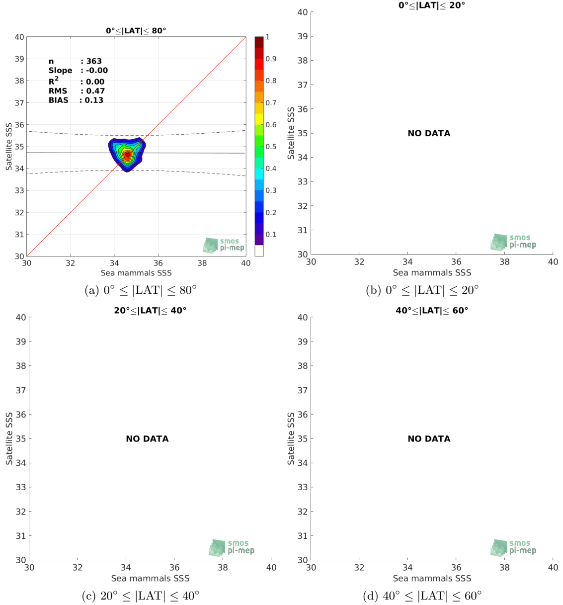
Figure 9: Contour maps of the concentration of SMOS-L3-BEC-ARCTIC-OA-V2-9DAYS-0.25DEG SSS (y-axis) versus Sea mammals SSS (x-axis) at match-up pairs for different latitude bands. For each plot, the red line shows x=y . The black thin and dashed lines indicate a linear fit through the data cloud and the \pm 95\% confidence levels, respectively. The number match-up pairs n , the slope and R^2 coefficient of the linear fit, the root mean square (RMS) and the mean bias between satellite and in situ data are indicated for each latitude band in each plots.
