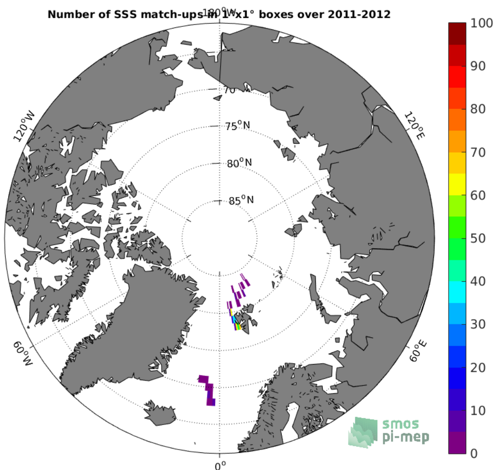
Figure 4: Number of SSS match-ups between Sea mammals SSS and the SMOS-L3-BEC-ARCTIC-OA-V2-9DAYS-0.25DEG SSS product for the Arctic Ocean Pi-MEP region over 1^\circ \times 1^\circ boxes and for the full satellite product period.
