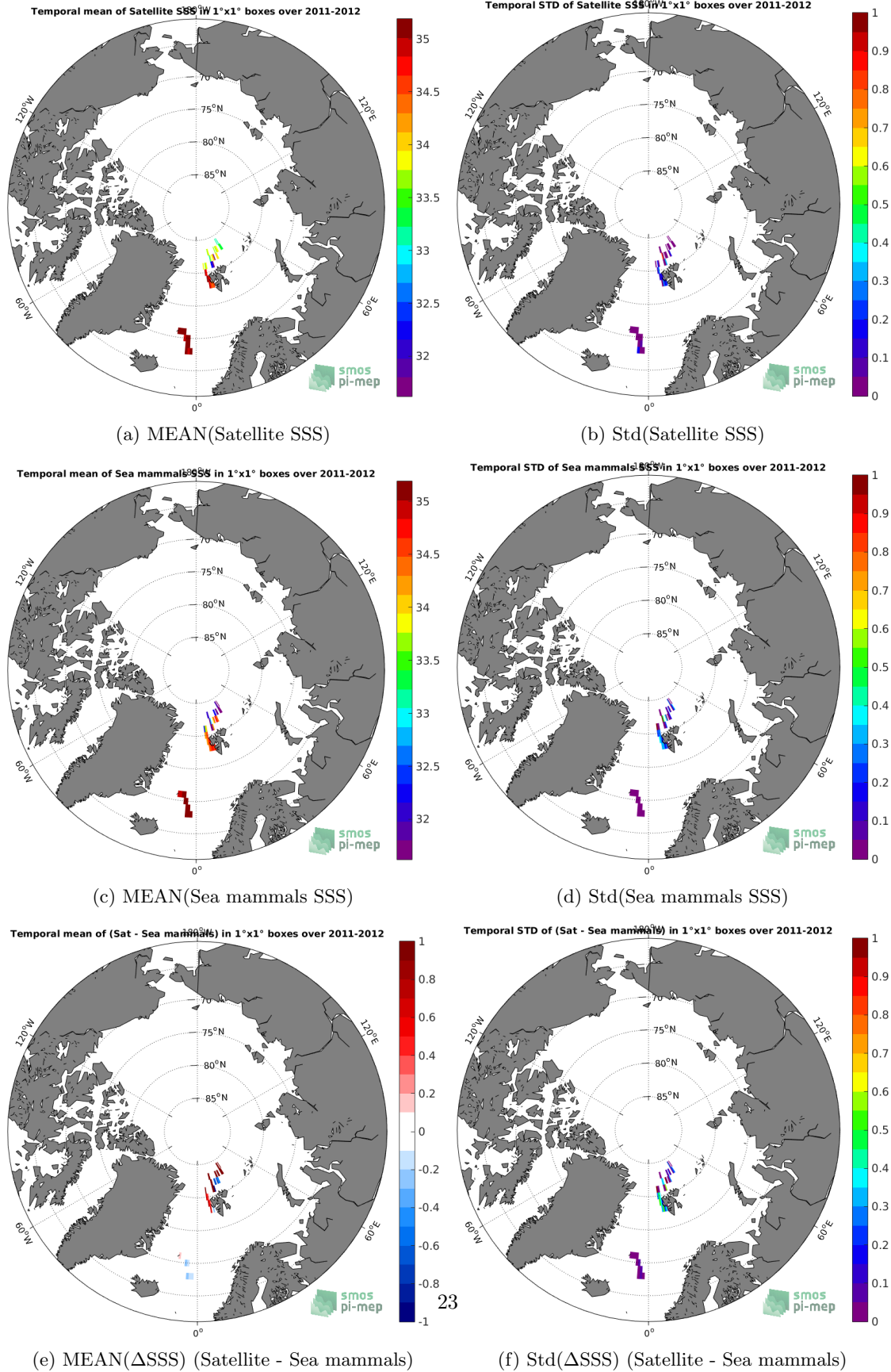
Figure 6: Temporal mean (left) and Std (right) of SSS from SMOS-L3-BEC-ARCTIC-OA-V2-9DAYS-0.25DEG (top), Sea mammals (middle), and of \Delta SSS (Satellite - Sea mammals). Only match-up pairs are used to generate these maps.
