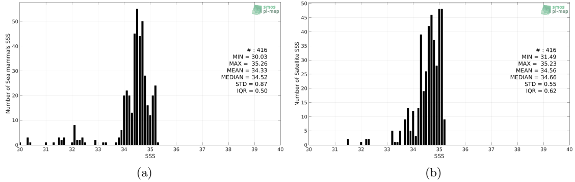
Figure 2: Histograms of SSS from Sea mammals (a) and SMOS-L3-BEC-ARCTIC-OA-V2-9DAYS-0.25DEG (b) considering all match-up pairs per bins of 0.1 over the Arctic Ocean Pi-MEP region and for the full satellite product period.
