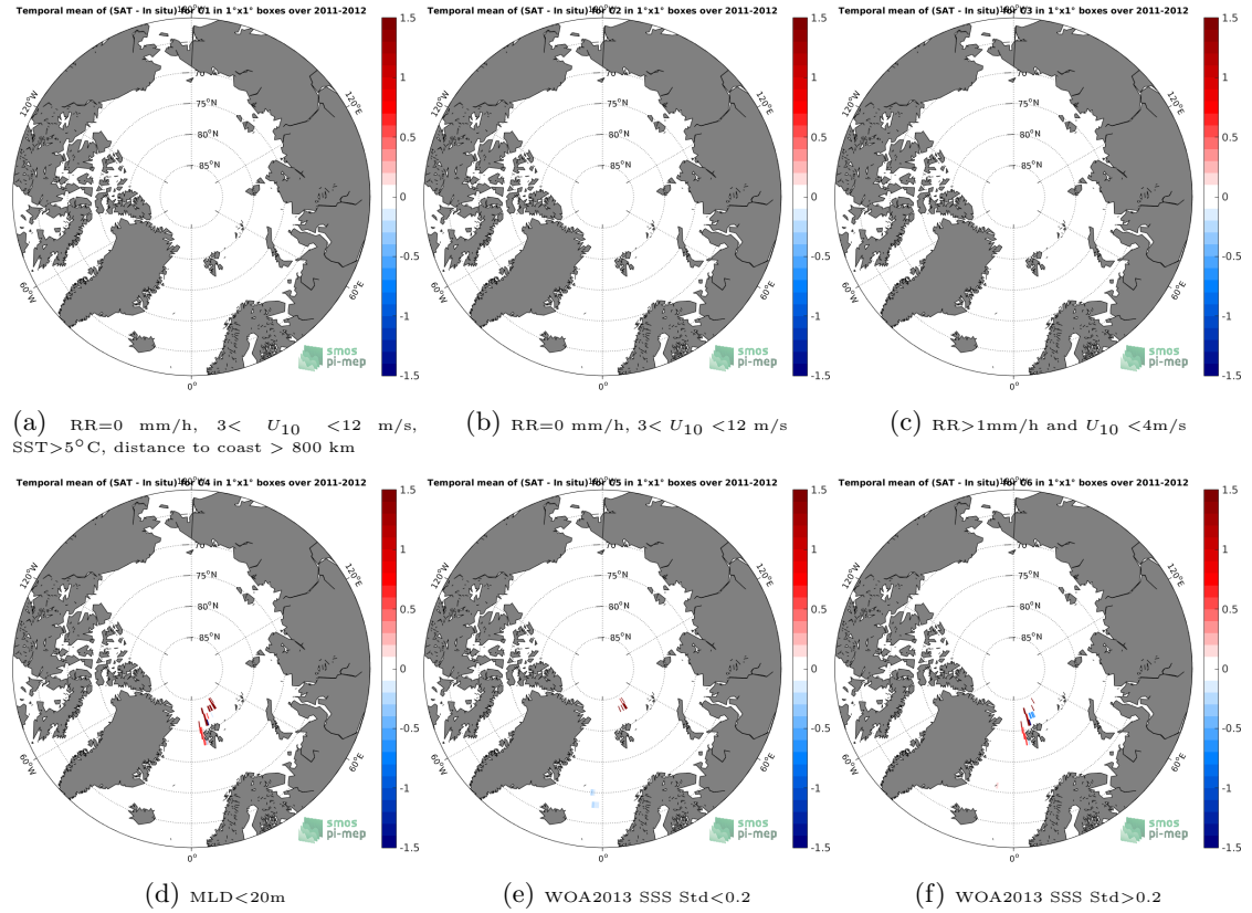
Figure 12: Temporal mean gridded over spatial boxes of size 1^\circ \times 1^\circ of \Delta SSS (SMOS-L3-BEC-ARCTIC-OA-V2-9DAYS-0.25DEG - Sea mammals) for 6 different subdatasets corresponding to: RR=0 mm/h, 3 < U_{10} < 12 m/s, SST > 5^\circ C , distance to coast > 800 km (a), RR=0 mm/h, 3 < U_{10} < 12 m/s (b), RR > 1 mm/h and U_{10} < 4 m/s (c), MLD < 20 m (d), WOA2013 SSS Std < 0.2 (e), WOA2013 SSS Std > 0.2 (f).
