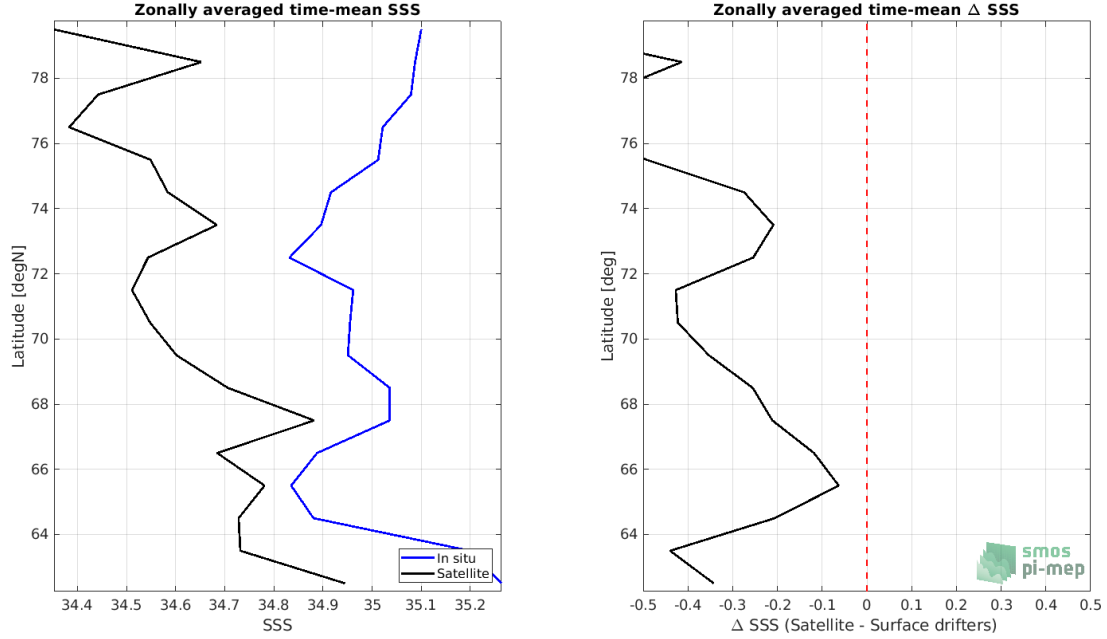
Figure 7: Left panel: Zonal mean SSS from SMOS SSS L3 Arctic OA v2 - 9 Days (BEC) satellite product (black) and from Surface drifters (blue). Right panel: Zonal mean of \Delta SSS (Satellite - Surface drifters) for all the collected Pi-MEP match-up pairs estimated over the full satellite product period.
