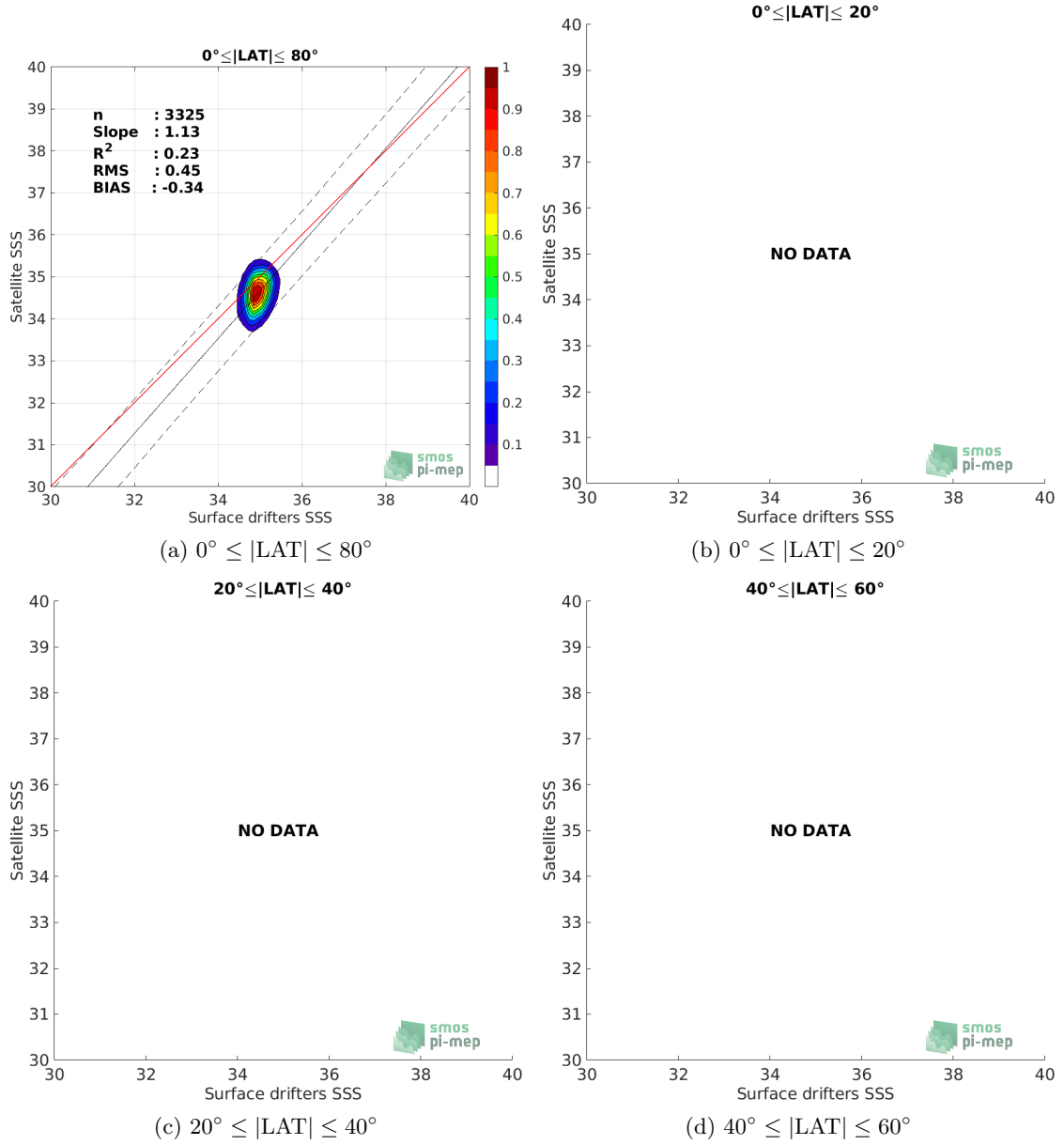
Figure 8: Contour maps of the concentration of SMOS SSS L3 Arctic OA v2 - 9 Days (BEC) SSS (y-axis) versus Surface drifters SSS (x-axis) at match-up pairs for different latitude bands. For each plot, the red line shows x=y . The black thin and dashed lines indicate a linear fit through the data cloud and the \pm 95\% confidence levels, respectively. The number match-up pairs n , the slope and R^2 coefficient of the linear fit, the root mean square (RMS) and the mean bias between satellite and in situ data are indicated for each latitude band in each plots.
