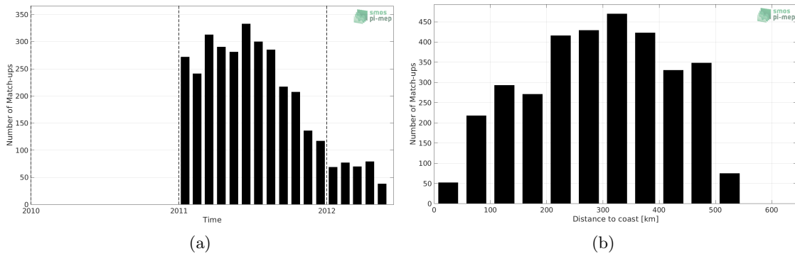
Figure 1: Number of match-ups between Surface drifters and SMOS SSS L3 Arctic OA v2 - 9 Days (BEC) SSS as a function of time (a) and as function of the distance to coast (b) over the Arctic Ocean Pi-MEP region and for the full satellite product period.
