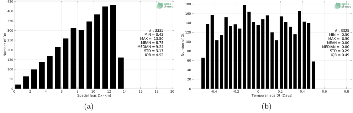
Figure 4: Histograms of the spatial (a) and temporal (b) lags between the location/time of the Surface drifters measurement and the date of the corresponding SMOS SSS L3 Arctic OA v2 - 9 Days (BEC) SSS pixel.
