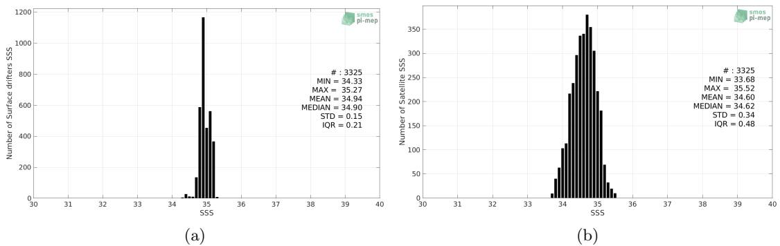
Figure 2: Histograms of SSS from Surface drifters (a) and SMOS SSS L3 Arctic OA v2 - 9 Days (BEC) (b) considering all match-up pairs per bins of 0.1 over the Arctic Ocean Pi-MEP region and for the full satellite product period.
