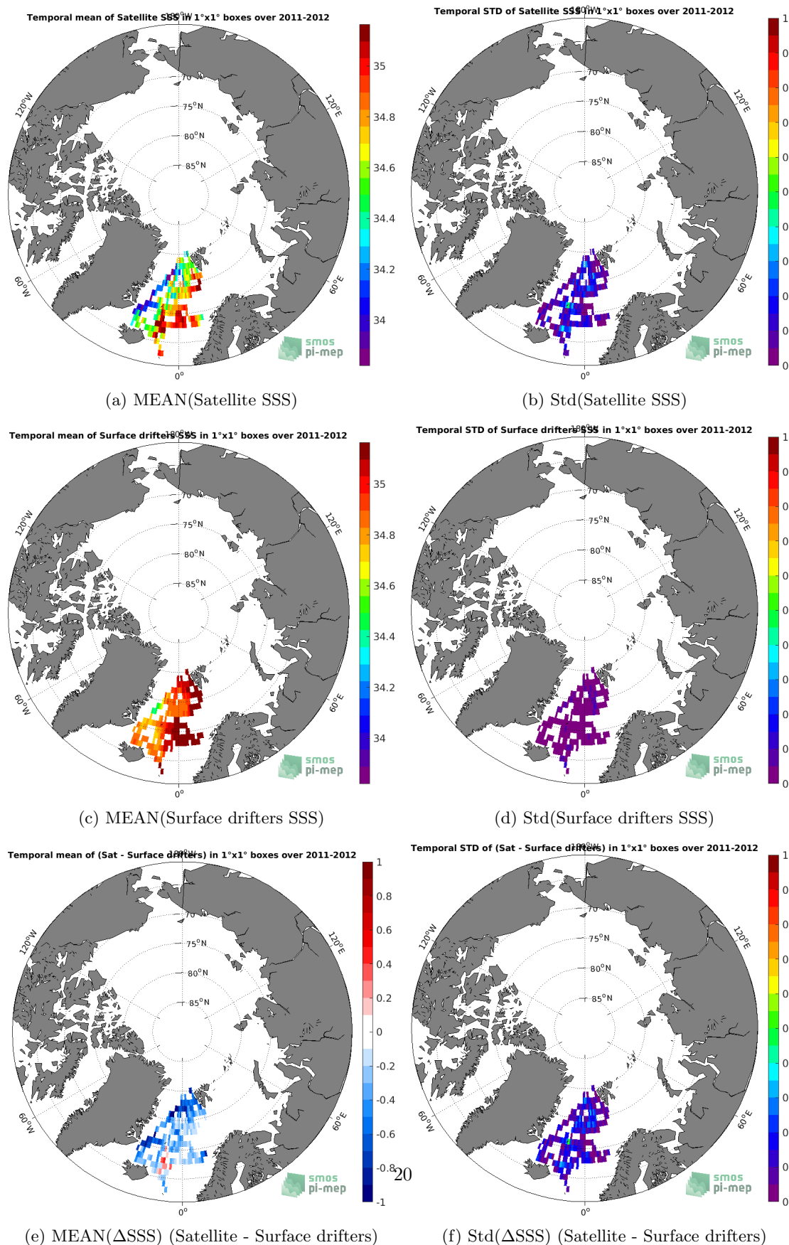
Figure 5: Temporal mean (left) and Std (right) of SSS from SMOS SSS L3 Arctic OA v2 - 9 Days (BEC) (top), Surface drifters (middle), and of \Delta SSS (Satellite - Surface drifters). Only match-up pairs are used to generate these maps.
