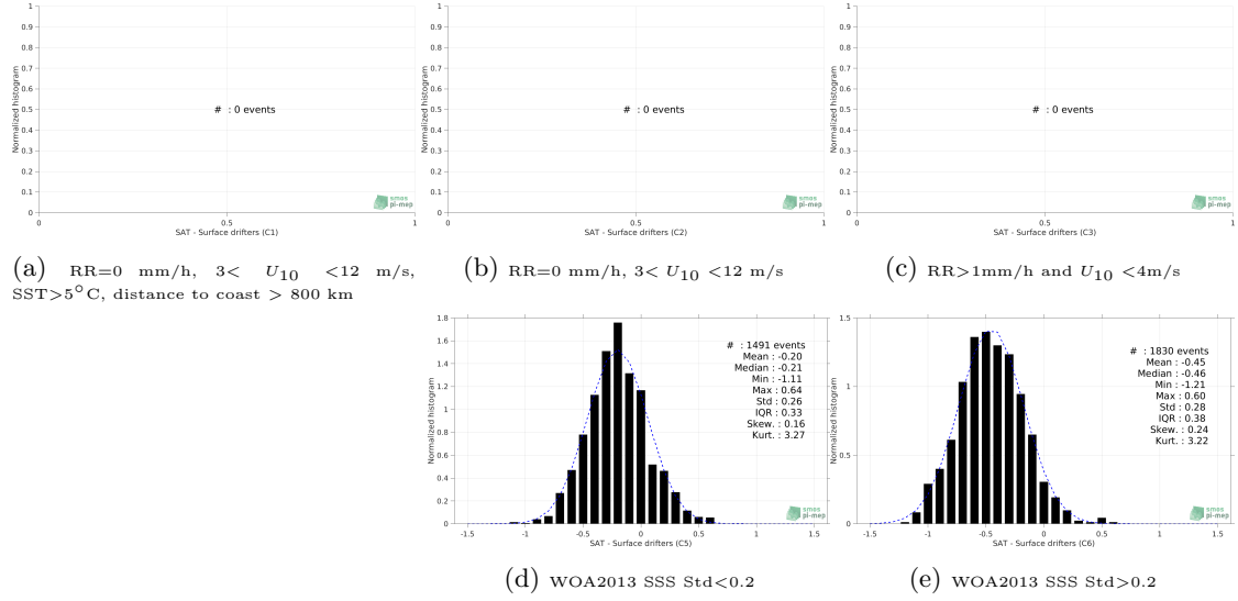
Figure 12: Normalized histogram of \Delta\text{SSS} (SMOS SSS L3 Arctic OA v2 - 9 Days (BEC) - Surface drifters) for 5 different subdatasets corresponding to: RR=0 mm/h, 3 < U_{10} < 12 m/s, SST > 5^\circ\text{C} , distance to coast > 800 km (a), RR=0 mm/h, 3 < U_{10} < 12 m/s (b), RR > 1\text{mm/h} and U_{10} < 4\text{m/s} (c), WOA2013 SSS Std <0.2 (d), WOA2013 SSS Std >0.2 (e).
