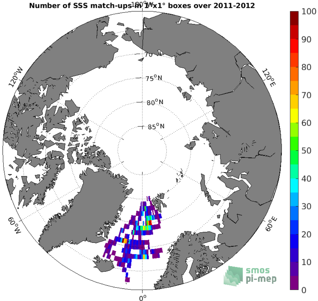
Figure 3: Number of SSS match-ups between Surface drifters SSS and the SMOS SSS L3 Arctic OA v2 - 9 Days (BEC) SSS product for the Arctic Ocean Pi-MEP region over 1^\circ \times 1^\circ boxes and for the full satellite product period.
