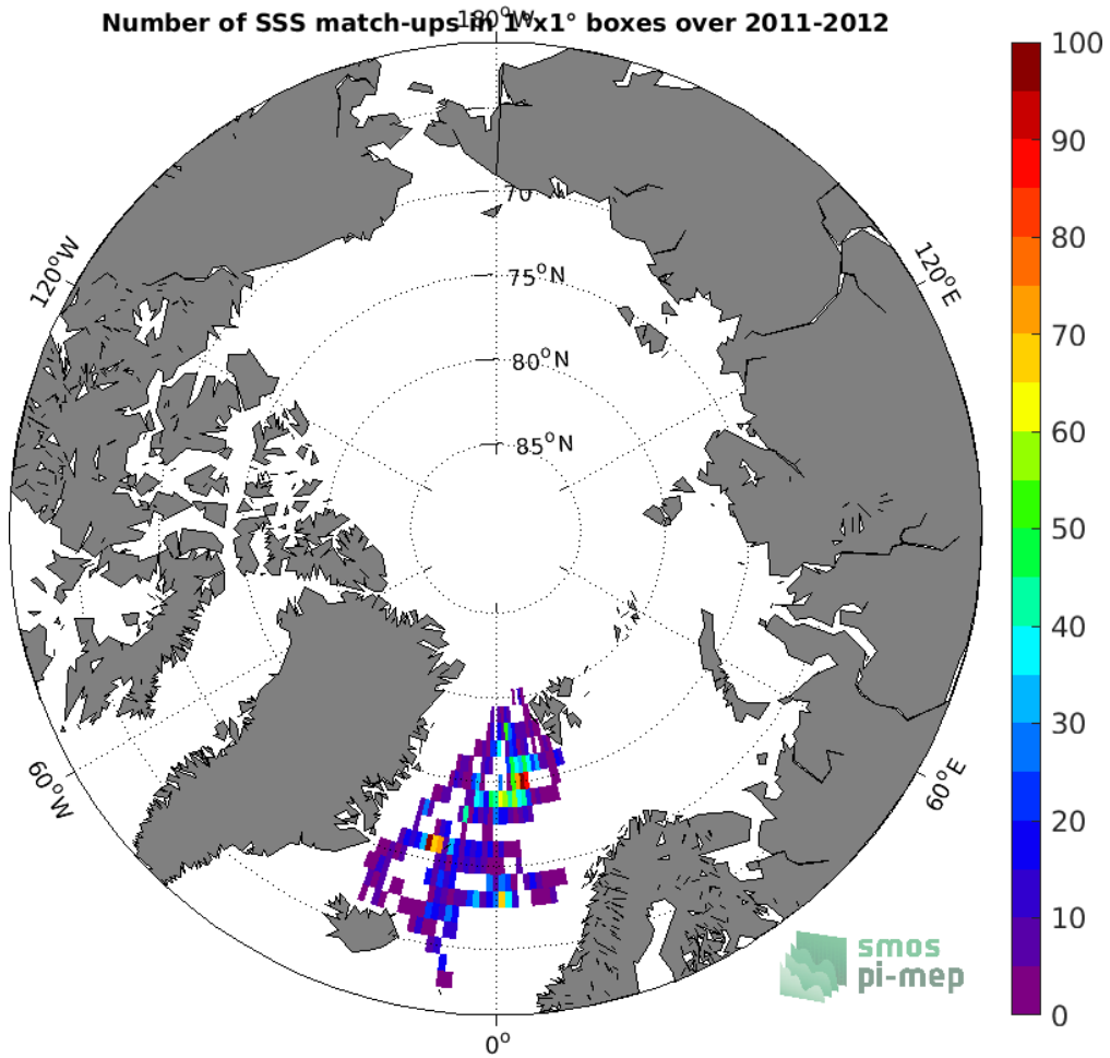
Figure 3: Number of SSS match-ups between Surface drifters SSS and the SMOS SSS L3 Arctic OA v2 - 9 Days (BEC) SSS product for the Arctic Ocean Pi-MEP region over 1°x1° boxes and for the full satellite product period.
