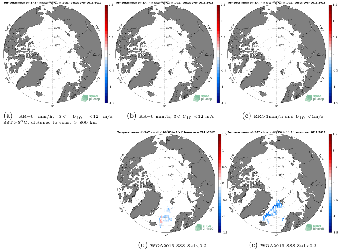
Figure 11: Temporal mean gridded over spatial boxes of size 1^{\circ}\times 1^{\circ} of \Delta\text{SSS} (SMOS SSS L3 Arctic OA v2 - 9 Days (BEC) - Surface drifters) for 5 different subdatasets corresponding to: RR=0 mm/h, 3 < U_{10} < 12 m/s, SST >5^{\circ}\text{C} , distance to coast > 800 km (a), RR=0 mm/h, 3 < U_{10} < 12 m/s (b), RR >1 mm/h and U_{10} < 4 m/s (c), WOA2013 SSS Std <0.2 (d), WOA2013 SSS Std >0.2 (e).
