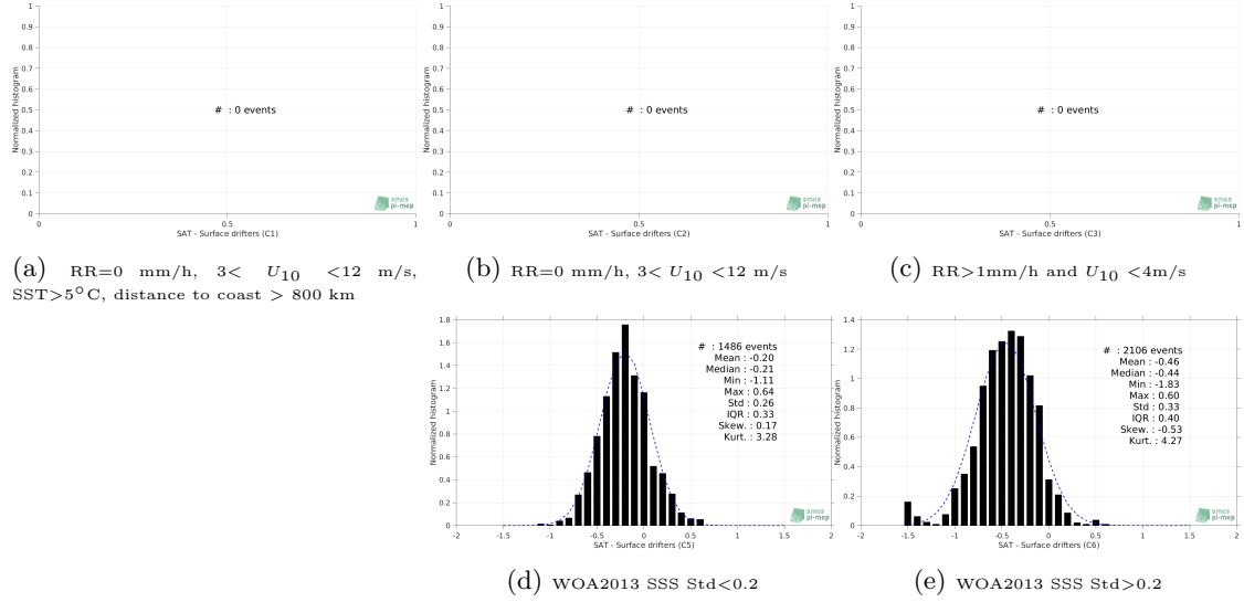
Figure 12: Normalized histogram of \Delta\text{SSS} (SMOS L3 Arctic OA v2 - 9 Days (BEC) - Surface drifters) for 5 different subdatasets corresponding to: RR=0 mm/h, 3 < U_{10} < 12 m/s, SST >5^{\circ}\text{C} , distance to coast > 800 km (a), RR=0 mm/h, 3 < U_{10} < 12 m/s (b), RR>1\text{mm/h} and U_{10} < 4\text{m/s} (c), WOA2013 SSS Std <0.2 (d), WOA2013 SSS Std >0.2 (e).
