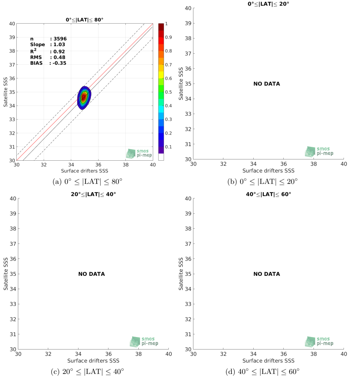
Figure 8: Contour maps of the concentration of SMOS L3 Arctic OA v2 - 9 Days (BEC) SSS (y-axis) versus Surface drifters SSS (x-axis) at match-up pairs for different latitude bands. For each plot, the red line shows x=y . The black thin and dashed lines indicate a linear fit through the cloud and the \pm 95\% confidence levels, respectively. The number match-up pairs n , the slope and R^2 coefficient of the linear fit, the root mean square (RMS) and the mean bias between satellite and in situ data are indicated for each latitude band in each plots.
