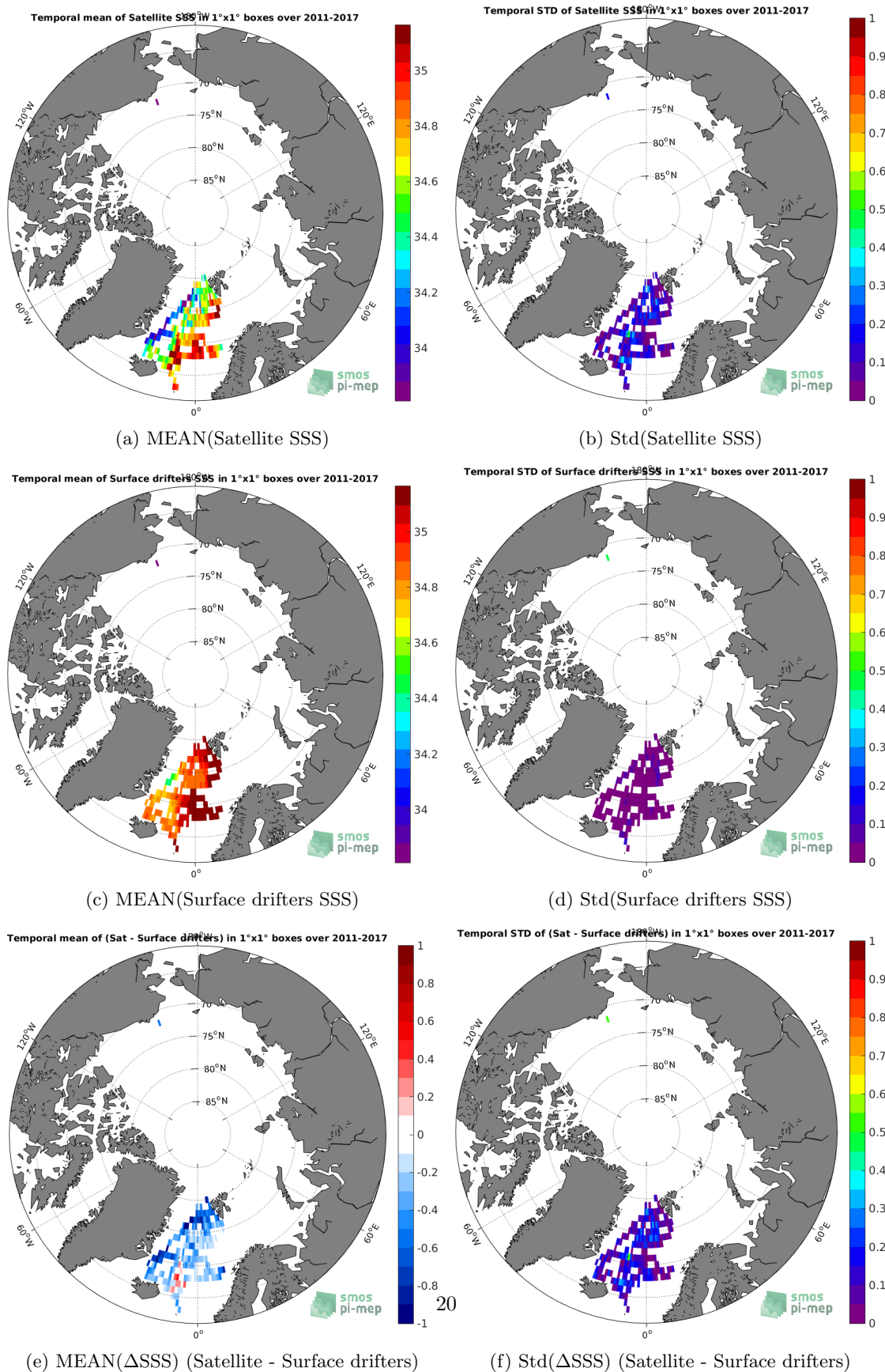
Figure 5: Temporal mean (left) and Std (right) of SSS from SMOS L3 Arctic OA v2 - 9 Days (BEC) (top), Surface drifters (middle), and of \Delta SSS (Satellite - Surface drifters). Only match-up pairs are used to generate these maps.
