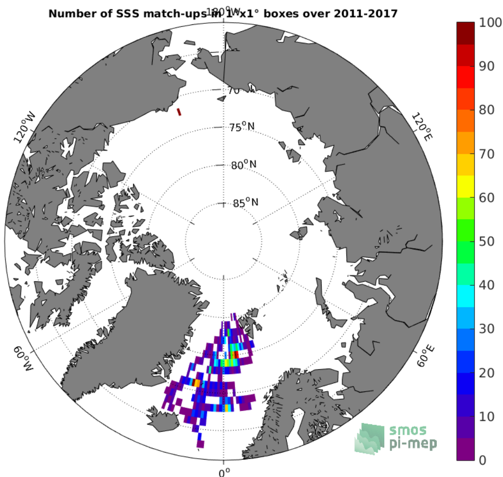
Figure 3: Number of SSS match-ups between Surface drifters SSS and the SMOS L3 Arctic OA v2 - 9 Days (BEC) SSS product for the Arctic Ocean Pi-MEP region over 1^\circ \times 1^\circ boxes and for the full satellite product period.
