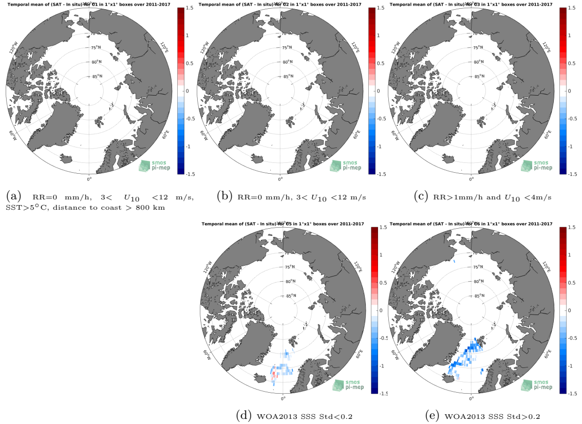
Figure 11: Temporal mean gridded over spatial boxes of size 1^{\circ}\times 1^{\circ} of \Delta\text{SSS} (SMOS L3 Arctic OA v2 - 9 Days (BEC) - Surface drifters) for 5 different subdatasets corresponding to: \text{RR}=0 mm/h, 3 < U_{10} < 12 m/s, \text{SST} > 5^{\circ}\text{C} , distance to coast > 800 km (a), \text{RR}=0 mm/h, 3 < U_{10} < 12 m/s (b), \text{RR} > 1 mm/h and U_{10} < 4 m/s (c), WOA2013 SSS Std < 0.2 (d), WOA2013 SSS Std > 0.2 (e).
