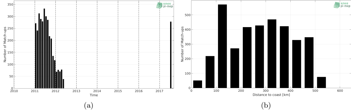
Figure 1: Number of match-ups between Surface drifters and SMOS L3 Arctic OA v2 - 9 Days (BEC) SSS as a function of time (a) and as function of the distance to coast (b) over the Arctic Ocean Pi-MEP region and for the full satellite product period.
