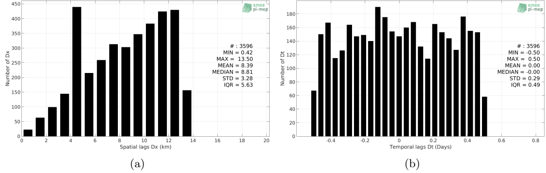
Figure 4: Histograms of the spatial (a) and temporal (b) lags between the time of the Surface drifters measurements and the date of the corresponding SMOS L3 Arctic OA v2 - 9 Days (BEC) SSS product.
