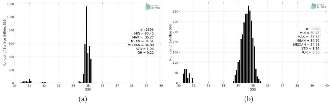
Figure 2: Histograms of SSS from Surface drifters (a) and SMOS L3 Arctic OA v2 - 9 Days (BEC) (b) considering all match-up pairs per bins of 0.1 over the Arctic Ocean Pi-MEP region and for the full satellite product period.
