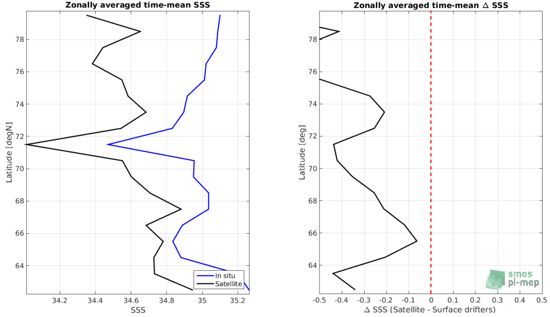
Figure 7: Left panel: Zonal mean SSS from SMOS L3 Arctic OA v2 - 9 Days (BEC) satellite product (black) and from Surface drifters (blue). Right panel: Zonal mean of \Delta SSS (Satellite - Surface drifters) for all the collected Pi-MEP match-up pairs estimated over the full satellite product period.
