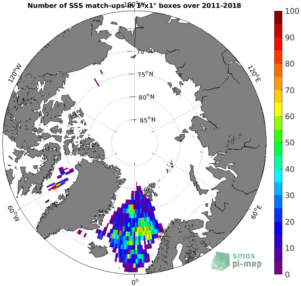
Figure 4: Number of SSS match-ups between Argo SSS and the SMOS SSS L3 Arctic OA v2 - 9 Days (BEC) SSS product for the Arctic Ocean Pi-MEP region over 1^\circ \times 1^\circ boxes and for the full satellite product period.
