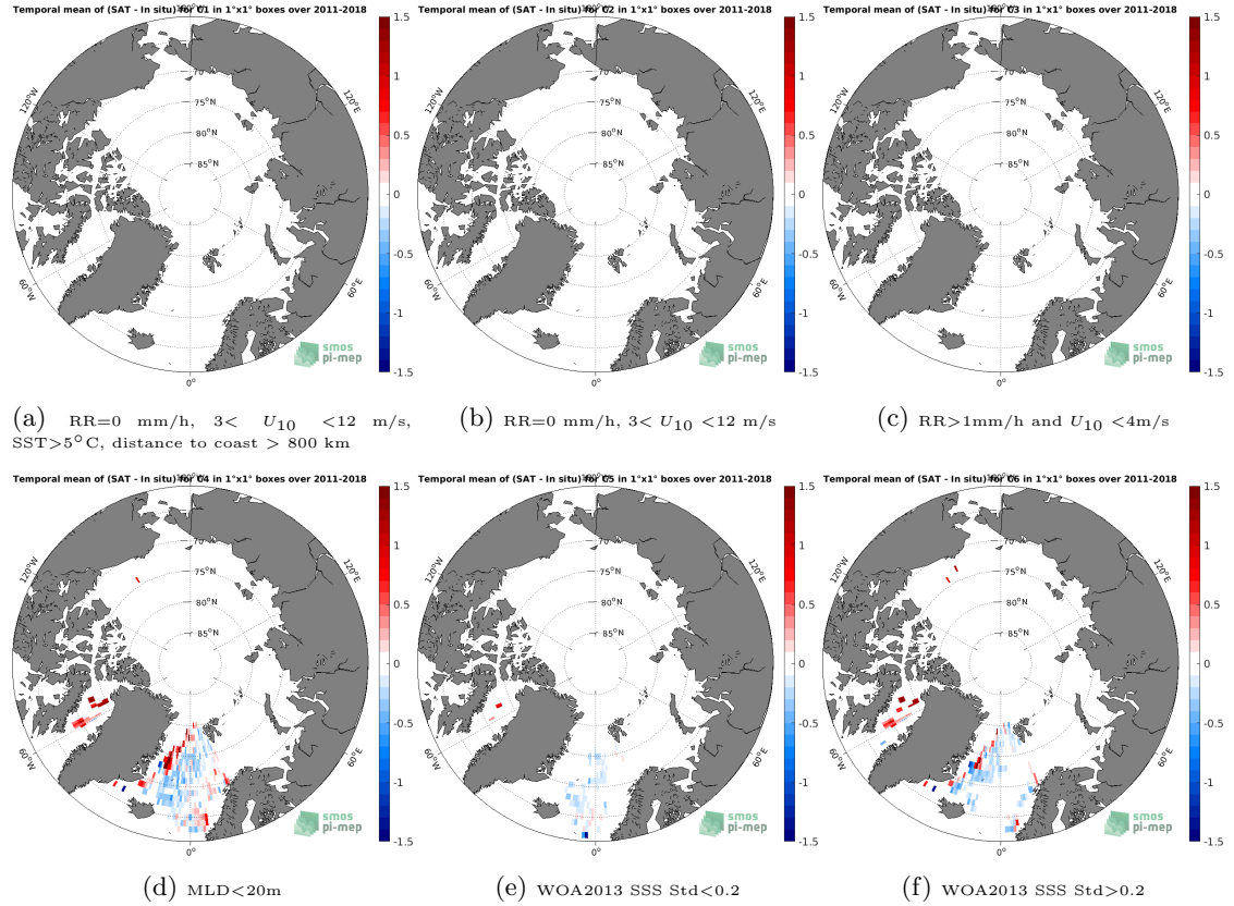
Figure 12: Temporal mean gridded over spatial boxes of size 1^{\circ} \times 1^{\circ} of \Delta\text{SSS} (SMOS SSS L3 Arctic OA v2 - 9 Days (BEC) - Argo) for 6 different subdatasets corresponding to: \text{RR}=0 mm/h, 3 < U_{10} < 12 m/s, \text{SST} > 5^{\circ}\text{C} , distance to coast > 800 km (a), \text{RR}=0 mm/h, 3 < U_{10} < 12 m/s (b), \text{RR} > 1\text{mm/h} and U_{10} < 4\text{m/s} (c), \text{MLD} < 20\text{m} (d), \text{WOA2013 SSS Std} < 0.2 (e), \text{WOA2013 SSS Std} > 0.2 (f).
