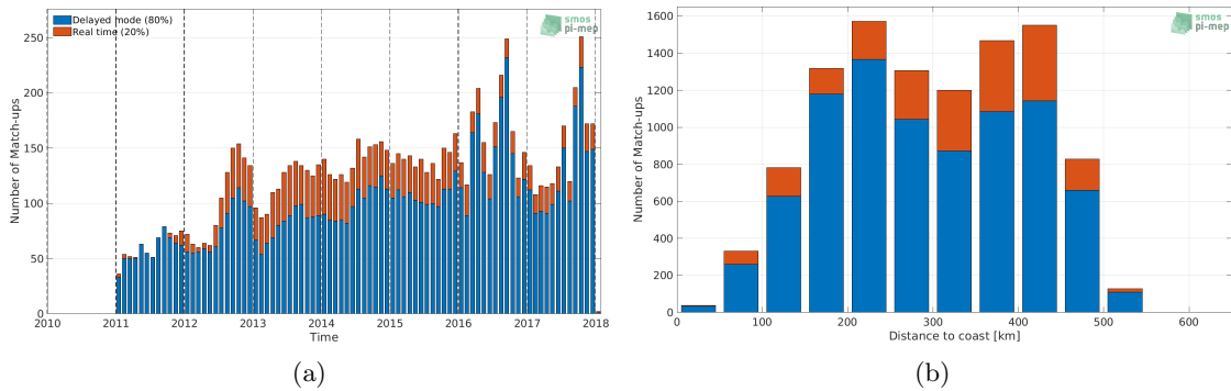
Figure 1: Number of match-ups between Argo and SMOS SSS L3 Arctic OA v2 - 9 Days (BEC) SSS as a function of time (a) and as function of the distance to coast (b) over the Arctic Ocean Pi-MEP region and for the full satellite product period.
