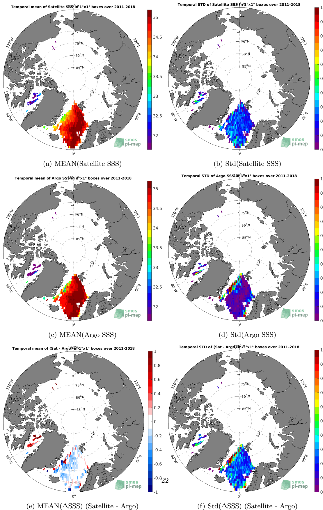
Figure 6: Temporal mean (left) and Std (right) of SSS from SMOS SSS L3 Arctic OA v2 - 9 Days (BEC) (top), Argo (middle), and of \Delta SSS (Satellite - Argo). Only match-up pairs are used to generate these maps.
