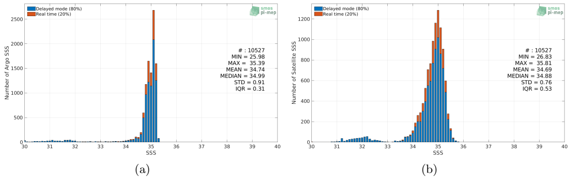
Figure 2: Histograms of SSS from Argo (a) and SMOS SSS L3 Arctic OA v2 - 9 Days (BEC) (b) considering all match-up pairs per bins of 0.1 over the Arctic Ocean Pi-MEP region and for the full satellite product period.
