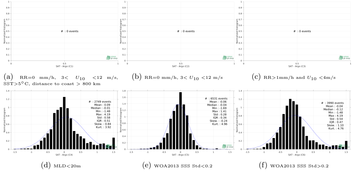
Figure 13: Normalized histogram of \Delta\text{SSS} (SMOS SSS L3 Arctic OA v2 - 9 Days (BEC) - Argo) for 6 different subdatasets corresponding to: RR=0 mm/h, 3 < U_{10} < 12 m/s, SST > 5^\circ\text{C} , distance to coast > 800 km (a), RR=0 mm/h, 3 < U_{10} < 12 m/s (b), RR > 1\text{mm/h} and U_{10} < 4\text{m/s} (c), MLD < 20\text{m} (d), WOA2013 SSS Std < 0.2 (e), WOA2013 SSS Std > 0.2 (f).
