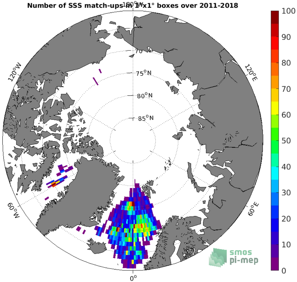
Figure 4: Number of SSS match-ups between Argo SSS and the SMOS SSS L3 Arctic OA v2 - 9 Days (BEC) SSS product for the Arctic Ocean Pi-MEP region over 1°x1° boxes and for the full satellite product period.
