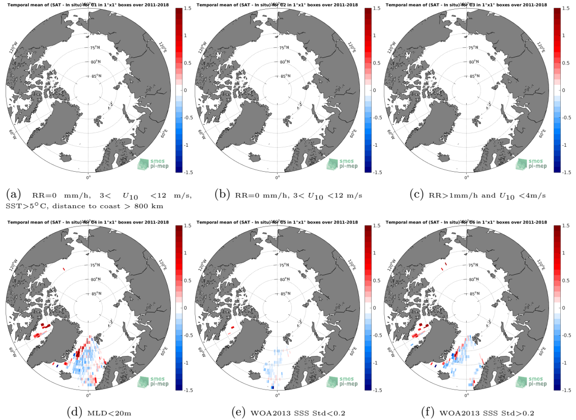
Figure 12: Temporal mean gridded over spatial boxes of size 1^{\circ}\times 1^{\circ} of \Delta\text{SSS} (SMOS L3 Arctic OA v2 - 9 Days (BEC) - Argo) for 6 different subdatasets corresponding to: RR=0 mm/h, 3 < U_{10} < 12 m/s, SST >5^{\circ}\text{C} , distance to coast > 800 km (a), RR=0 mm/h, 3 < U_{10} < 12 m/s (b), RR >1 mm/h and U_{10} < 4 m/s (c),MLD <20 m (d),WOA2013 SSS Std <0.2 (e),WOA2013 SSS Std >0.2 (f).
