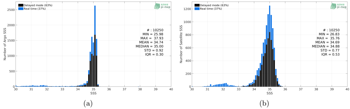
Figure 2: Histograms of SSS from Argo (a) and SMOS L3 Arctic OA v2 - 9 Days (BEC) (b) considering all match-up pairs per bins of 0.1 over the Arctic Ocean Pi-MEP region and for the full satellite product period.
