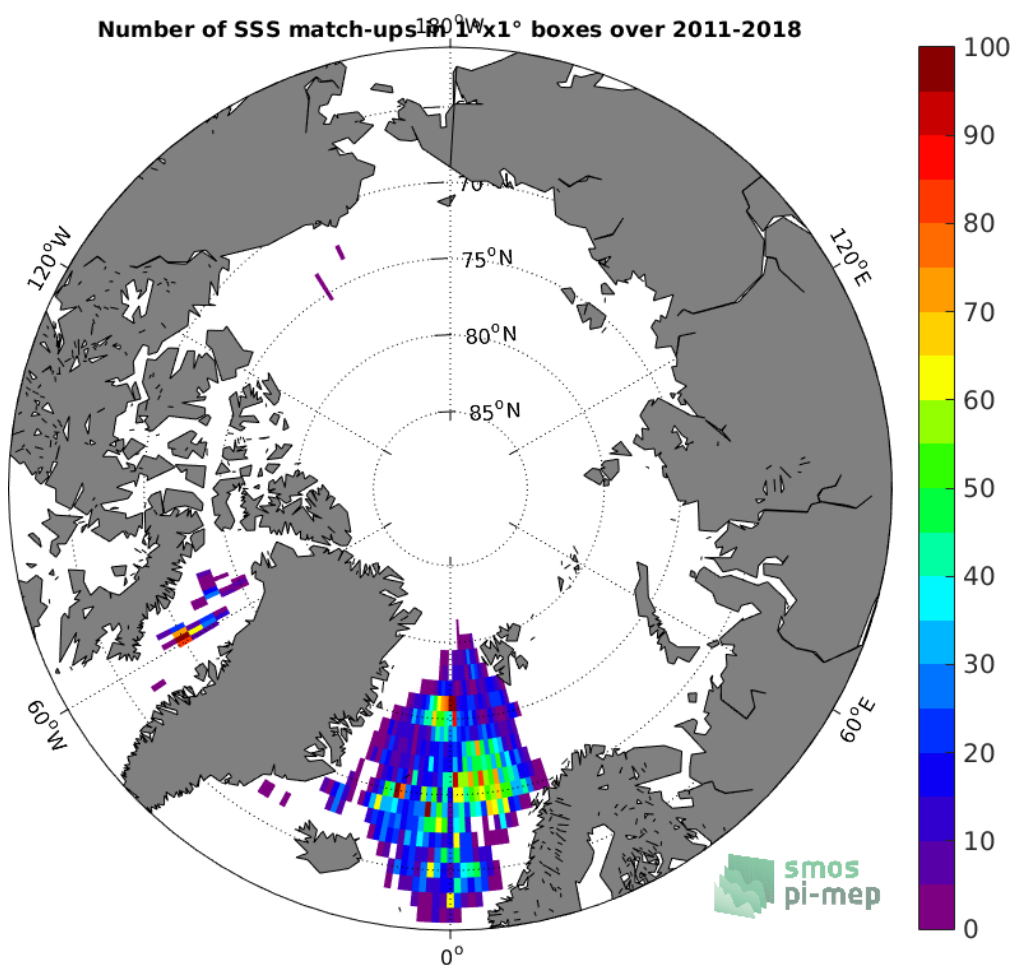
Figure 4: Number of SSS match-ups between Argo SSS and the SMOS L3 Arctic OA v2 - 9 Days (BEC) SSS product for the Arctic Ocean Pi-MEP region over 1^\circ \times 1^\circ boxes and for the full satellite product period.
