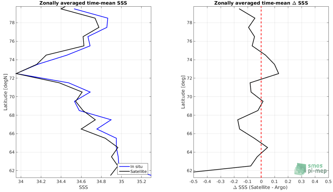
Figure 8: Left panel: Zonal mean SSS from SMOS L3 Arctic OA v2 - 9 Days (BEC) satellite product (black) and from Argo (blue). Right panel: Zonal mean of \Delta SSS (Satellite - Argo) for all the collected Pi-MEP match-up pairs estimated over the full satellite product period.
