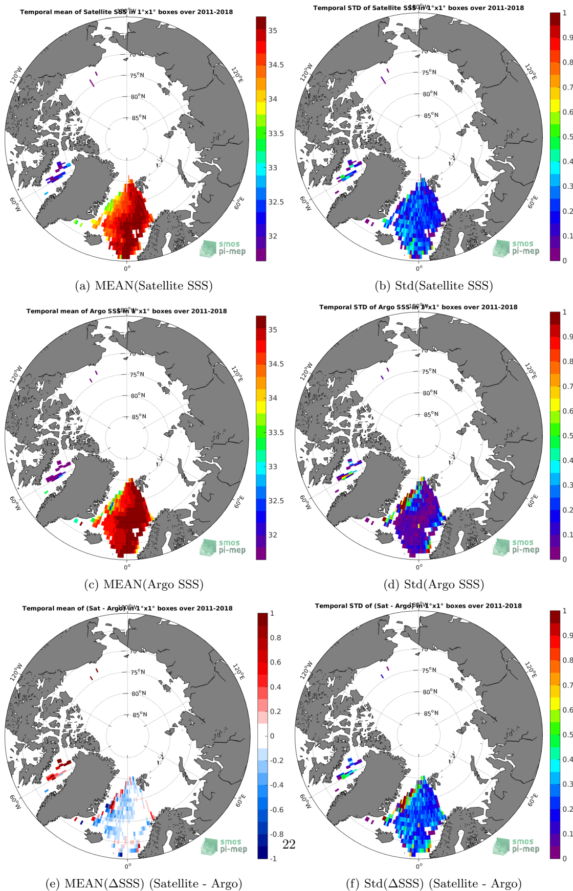
Figure 6: Temporal mean (left) and Std (right) of SSS from SMOS L3 Arctic OA v2 - 9 Days (BEC) (top), Argo (middle), and of ΔSSS (Satellite - Argo). Only match-up pairs are used to generate these maps.
