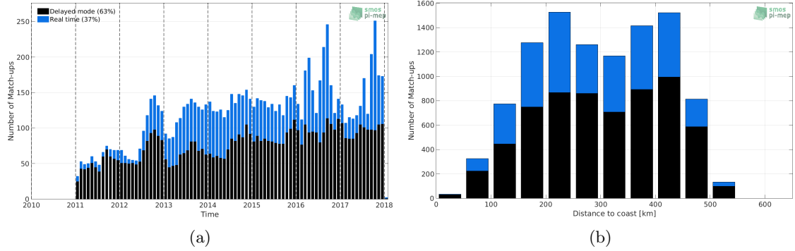
Figure 1: Number of match-ups between Argo and SMOS L3 Arctic OA v2 - 9 Days (BEC) SSS as a function of time (a) and as function of the distance to coast (b) over the Arctic Ocean Pi-MEP region and for the full satellite product period.
