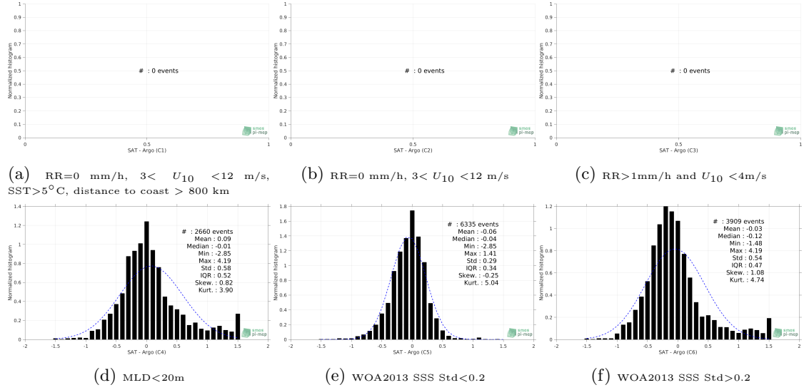
Figure 13: Normalized histogram of \Delta\text{SSS} (SMOS L3 Arctic OA v2 - 9 Days (BEC) - Argo) for 6 different subdatasets corresponding to: RR=0 mm/h, 3 < U_{10} < 12 m/s, SST > 5^\circ\text{C} , distance to coast > 800 km (a), RR=0 mm/h, 3 < U_{10} < 12 m/s (b), RR > 1\text{mm/h} and U_{10} < 4\text{m/s} (c), MLD < 20\text{m} (d), WOA2013 SSS Std < 0.2 (e), WOA2013 SSS Std > 0.2 (f).
