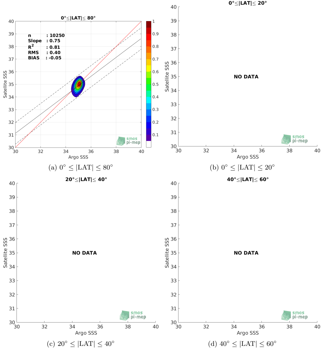
Figure 9: Contour maps of the concentration of SMOS L3 Arctic OA v2 - 9 Days (BEC) SSS (y-axis) versus Argo SSS (x-axis) at match-up pairs for different latitude bands. For each plot, the red line shows x=y . The black thin and dashed lines indicate a linear fit through the data cloud and the \pm 95\% confidence levels, respectively. The number match-up pairs n , the slope and R^2 coefficient of the linear fit, the root mean square (RMS) and the mean bias between satellite and in situ data are indicated for each latitude band in each plots.
