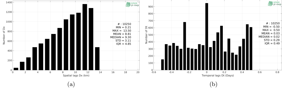
Figure 5: Histograms of the spatial (a) and temporal (b) lags between the time of the Argo measurements and the date of the corresponding SMOS L3 Arctic OA v2 - 9 Days (BEC) SSS product.
