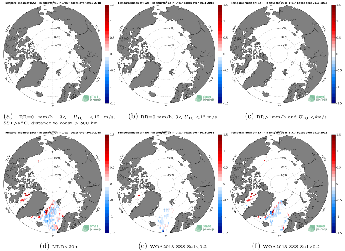
Figure 12: Temporal mean gridded over spatial boxes of size 1^\circ \times 1^\circ of \Delta SSS (SMOS-L3-BEC-ARCTIC-OA-V2-9DAYS-0.25DEG - Argo) for 6 different subdatasets corresponding to: RR=0 mm/h, 3 < U_{10} < 12 m/s, SST > 5^\circ C , distance to coast > 800 km (a), RR=0 mm/h, 3 < U_{10} < 12 m/s (b), RR > 1 mm/h and U_{10} < 4 m/s (c), MLD < 20 m (d), WOA2013 SSS Std < 0.2 (e), WOA2013 SSS Std > 0.2 (f).
