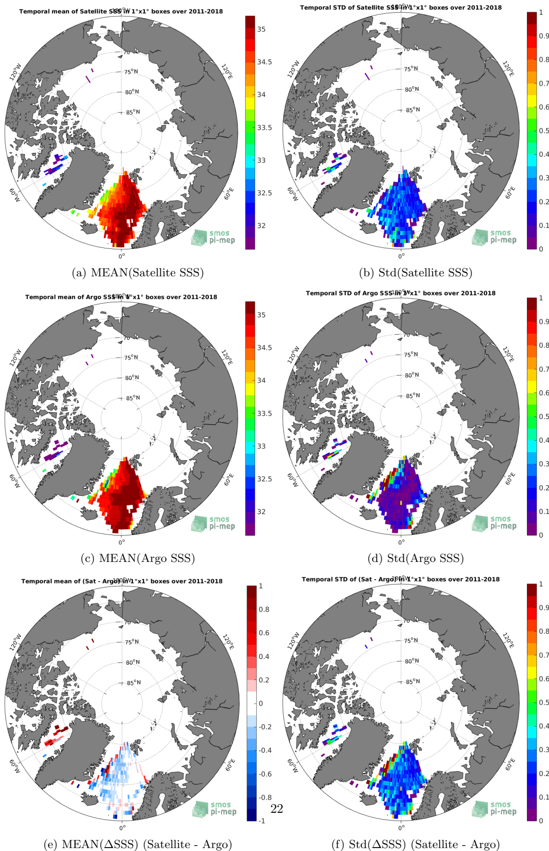
Figure 6: Temporal mean (left) and Std (right) of SSS from SMOS-L3-BEC-ARCTIC-OA-V2-9DAYS-0.25DEG (top), Argo (middle), and of \Delta SSS (Satellite - Argo). Only match-up pairs are used to generate these maps.
