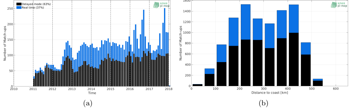
Figure 1: Number of match-ups between Argo and SMOS-L3-BEC-ARCTIC-OA-V2-9DAYS-0.25DEG SSS as a function of time (a) and as function of the distance to coast (b) over the Arctic Ocean Pi-MEP region and for the full satellite product period.
