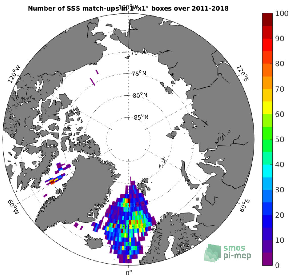
Figure 4: Number of SSS match-ups between Argo SSS and the SMOS-L3-BEC-ARCTIC-OA-V2-9DAYS-0.25DEG SSS product for the Arctic Ocean Pi-MEP region over 1^\circ \times 1^\circ boxes and for the full satellite product period.
