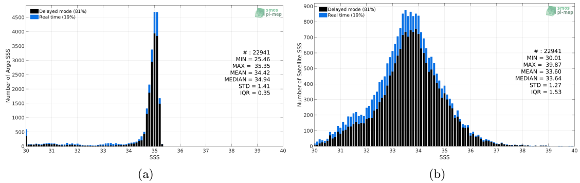
Figure 2: Histograms of SSS from Argo (a) and SMOS SSS L2-AVERAGED v700 (ESA) (b) considering all match-up pairs per bins of 0.1 over the Arctic Ocean Pi-MEP region and for the full satellite product period.
