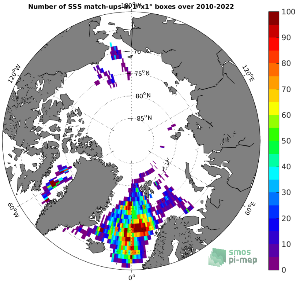
Figure 4: Number of SSS match-ups between Argo SSS and the SMOS SSS L2-AVERAGED v700 (ESA) SSS product for the Arctic Ocean Pi-MEP region over 1^\circ \times 1^\circ boxes and for the full satellite product period.
