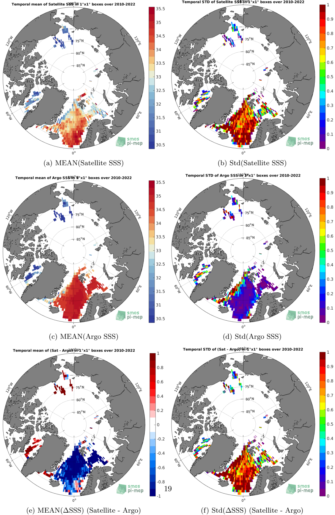
Figure 6: Temporal mean (left) and Std (right) of SSS from SMOS SSS L2-AVERAGED v700 (ESA) (top), Argo (middle), and of \Delta SSS (Satellite - Argo). Only match-up pairs are used to generate these maps.
