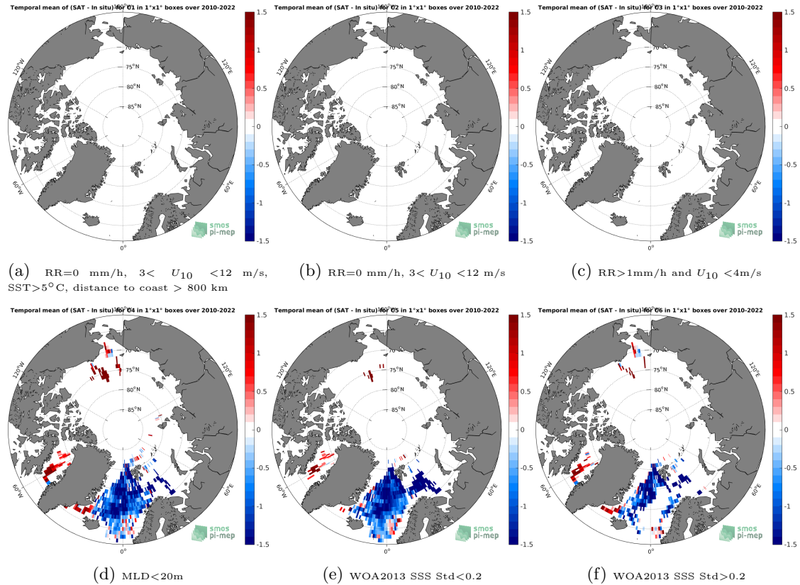
Figure 12: Temporal mean gridded over spatial boxes of size 1^{\circ}\times 1^{\circ} of \Delta\text{SSS} (SMOS SSS L2-AVERAGED v700 (ESA) - Argo) for 6 different subdatasets corresponding to:RR=0 mm/h, 3 < U_{10} < 12 m/s, SST >5^{\circ}\text{C} , distance to coast > 800 km (a), RR=0 mm/h, 3 < U_{10} < 12 m/s (b), RR >1 mm/h and U_{10} < 4 m/s (c),MLD <20 m (d),WOA2013 SSS Std <0.2 (e),WOA2013 SSS Std >0.2 (f).
