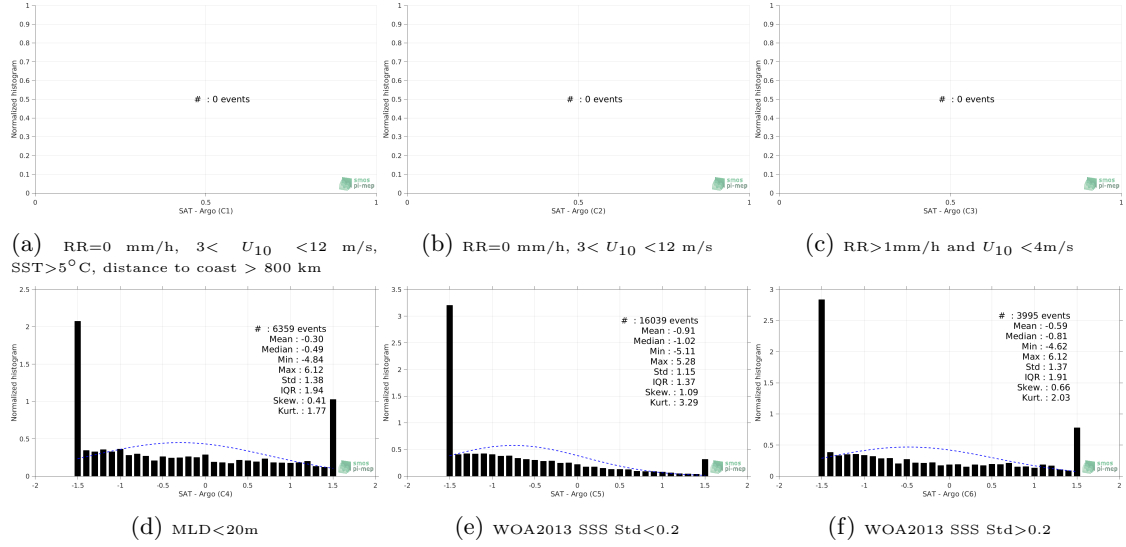
Figure 13: Normalized histogram of \Delta SSS (SMOS SSS L2-AVERAGED v700 (ESA) - Argo) for 6 different subdatasets corresponding to: RR=0 mm/h, 3 < U_{10} < 12 m/s, SST > 5°C, distance to coast > 800 km (a), RR=0 mm/h, 3 < U_{10} < 12 m/s (b), RR > 1mm/h and U_{10} < 4 m/s (c), MLD < 20m (d), WOA2013 SSS Std < 0.2 (e), WOA2013 SSS Std > 0.2 (f).
