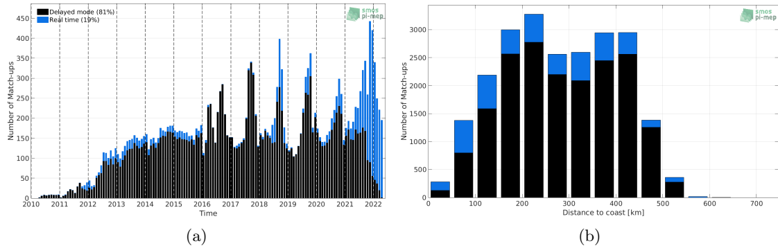
Figure 1: Number of match-ups between Argo and SMOS SSS L2-AVERAGED v700 (ESA) SSS as a function of time (a) and as function of the distance to coast (b) over the Arctic Ocean Pi-MEP region and for the full satellite product period.
