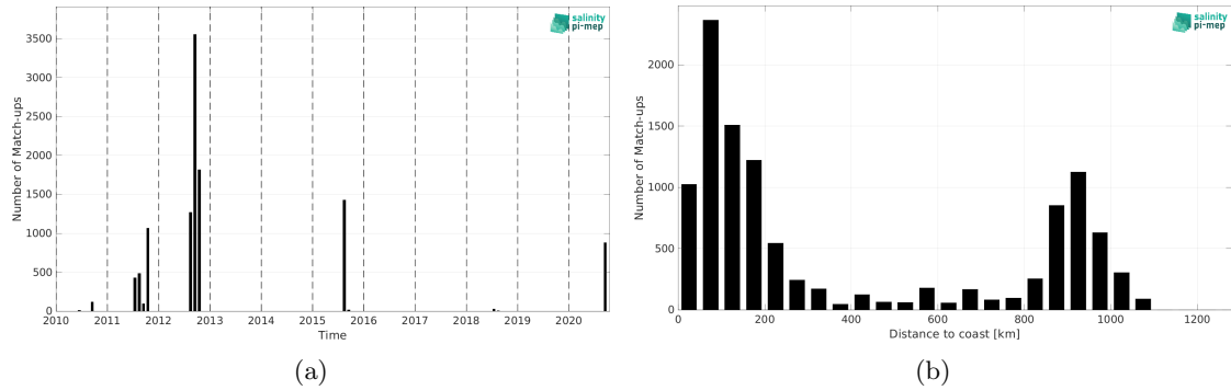
Figure 1: Number of match-ups between TSG (SAMOS) and SMOS SSS L2 v700 (ESA) SSS as a function of time (a) and as function of the distance to coast (b) over the Arctic Ocean Pi-MEP region and for the full satellite product period.
