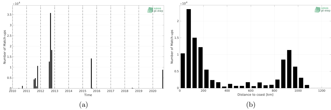
Figure 1: Number of match-ups between TSG (SAMOS) and SMOS SSS L2 v700 (ESA) SSS as a function of time (a) and as function of the distance to coast (b) over the Arctic Ocean Pi-MEP region and for the full satellite product period.
