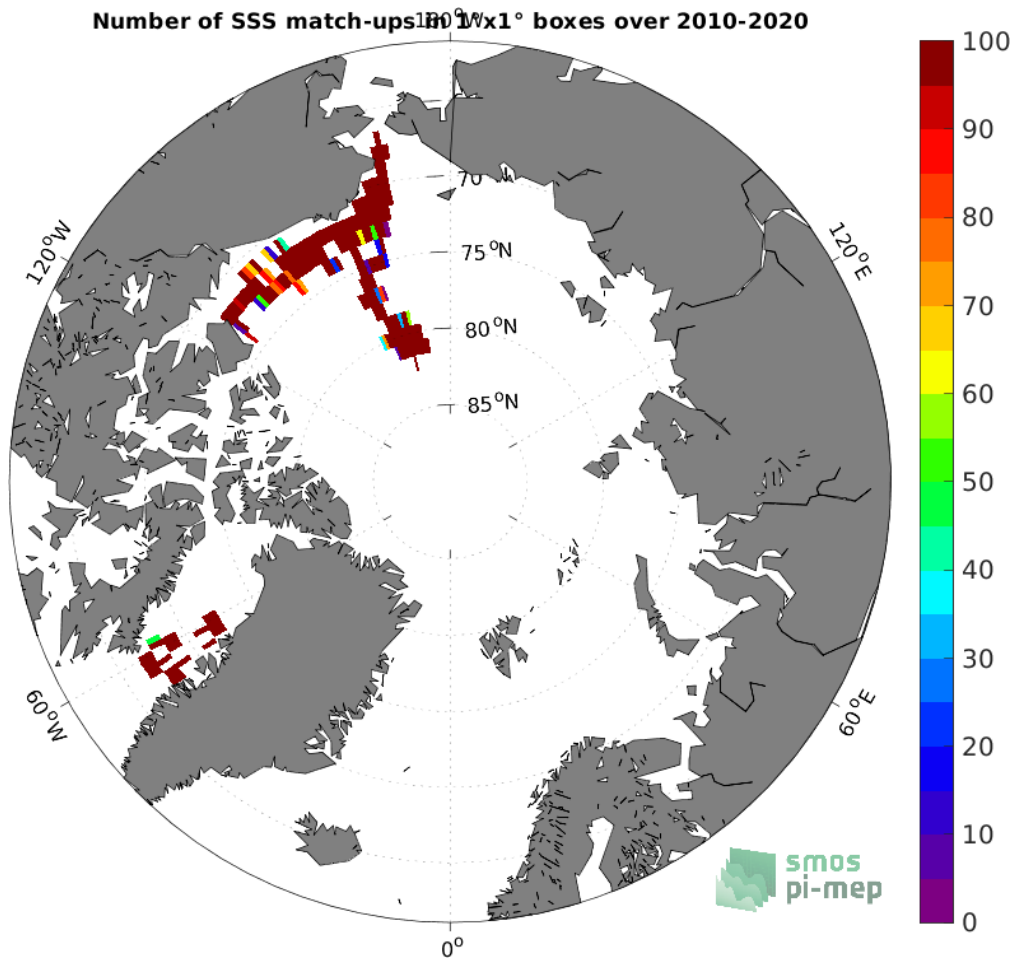
Figure 4: Number of SSS match-ups between TSG (SAMOS) SSS and the SMOS SSS L2 v700 (ESA) SSS product for the Arctic Ocean Pi-MEP region over 1^{\circ} \times 1^{\circ} boxes and for the full satellite product period.
