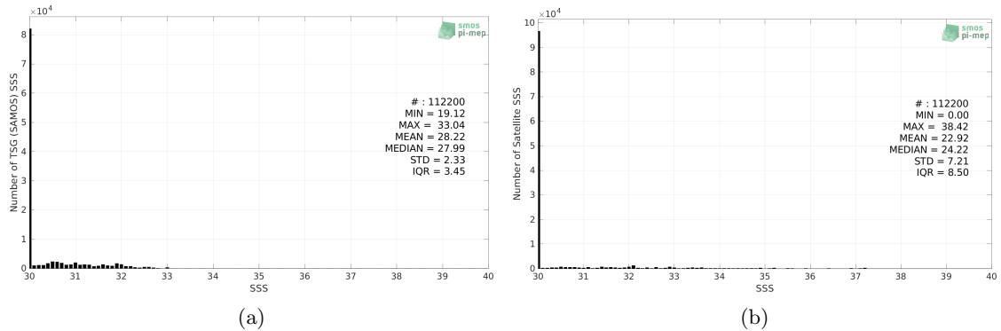
Figure 2: Histograms of SSS from TSG (SAMOS) (a) and SMOS SSS L2 v700 (ESA) (b) considering all match-up pairs per bins of 0.1 over the Arctic Ocean Pi-MEP region and for the full satellite product period.
