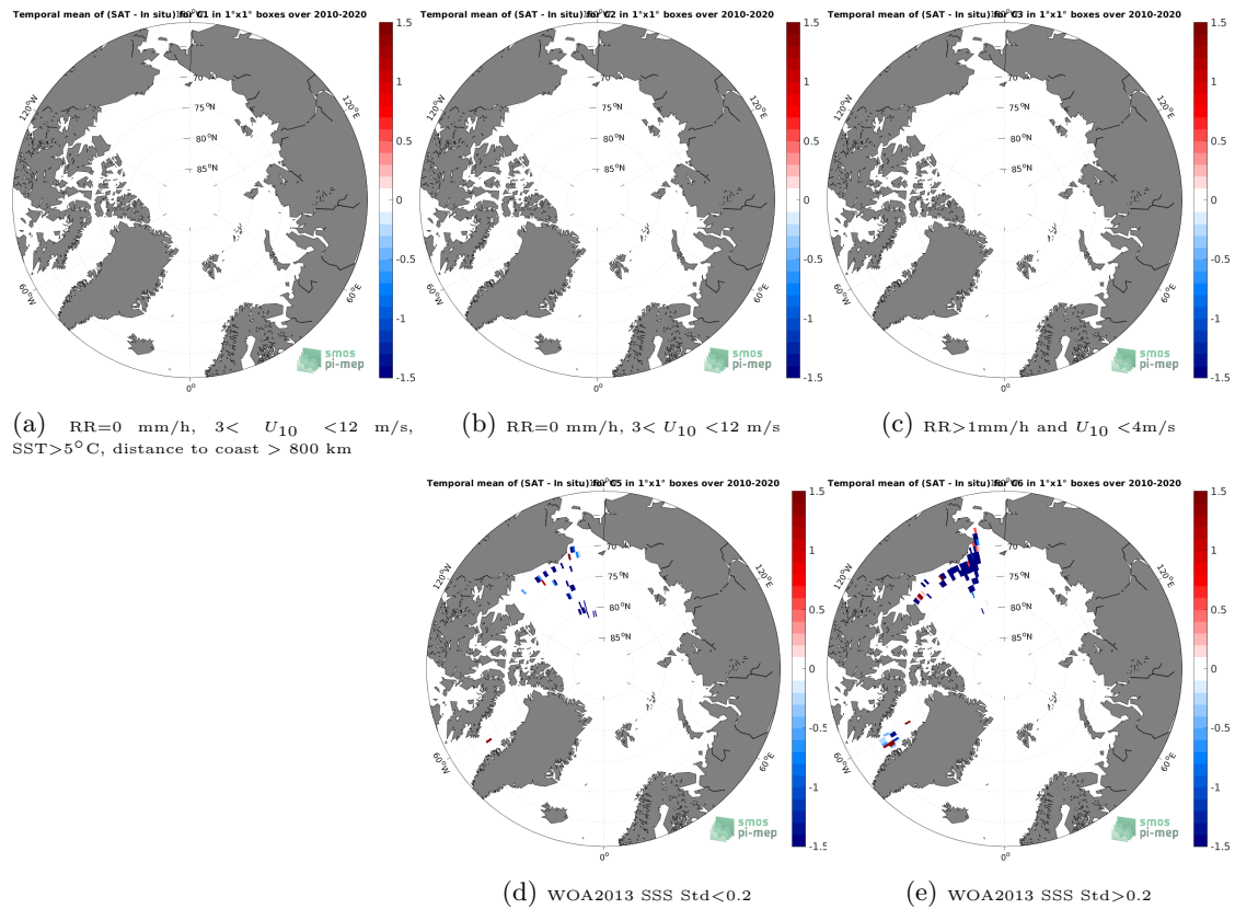
Figure 12: Temporal mean gridded over spatial boxes of size 1^{\circ}\times 1^{\circ} of \Delta\text{SSS} (SMOS SSS L2 v700 (ESA) - TSG (SAMOS)) for 5 different subdatasets corresponding to:RR=0 mm/h, 3 < U_{10} < 12 m/s, SST > 5^{\circ}\text{C} , distance to coast > 800 km (a), RR=0 mm/h, 3 < U_{10} < 12 m/s (b), RR > 1 mm/h and U_{10} < 4 m/s (c), WOA2013 SSS Std < 0.2 (d), WOA2013 SSS Std > 0.2 (e).
