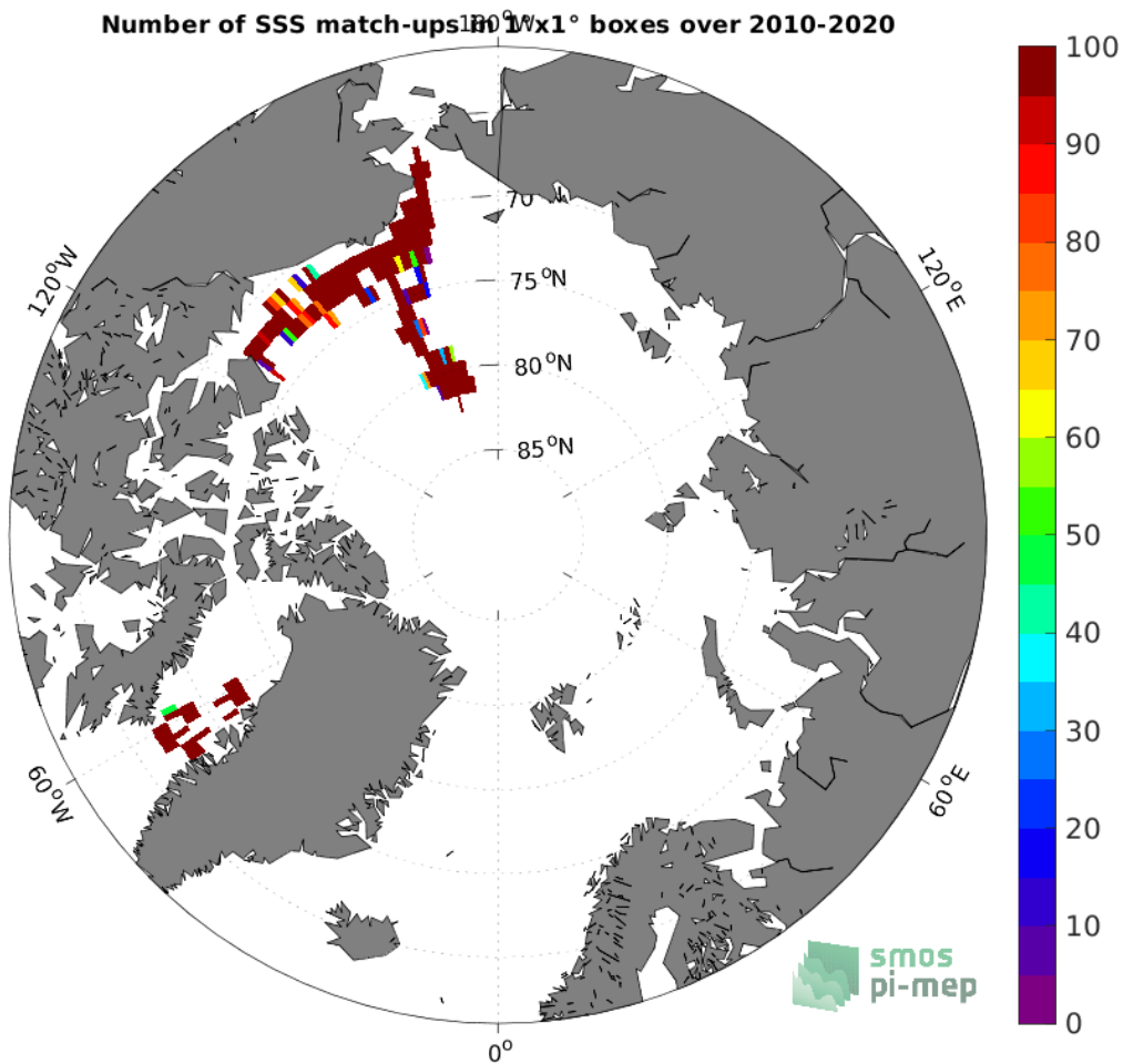
Figure 4: Number of SSS match-ups between TSG (SAMOS) SSS and the SMOS SSS L2 v700 (ESA) SSS product for the Arctic Ocean Pi-MEP region over 1^\circ \times 1^\circ boxes and for the full satellite product period.
