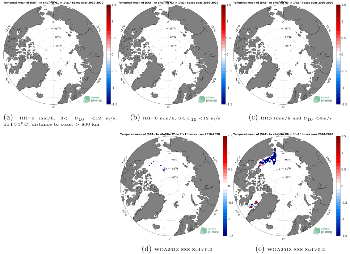
Figure 12: Temporal mean gridded over spatial boxes of size 1^{\circ} \times 1^{\circ} of \Delta\text{SSS} (SMOS SSS L2 v700 (ESA) - TSG (SAMOS)) for 5 different subdatasets corresponding to: \text{RR}=0 mm/h, 3 < U_{10} < 12 m/s, \text{SST} > 5^{\circ}\text{C} , distance to coast > 800 km (a), \text{RR}=0 mm/h, 3 < U_{10} < 12 m/s (b), \text{RR} > 1 mm/h and U_{10} < 4 m/s (c), WOA2013 SSS Std < 0.2 (d), WOA2013 SSS Std > 0.2 (e).
