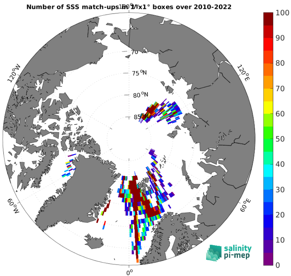
Figure 5: Number of SSS match-ups between TSG (Polarstern) SSS and the SMOS SSS L2 v700 (ESA) SSS product for the Arctic Ocean Pi-MEP region over 1^\circ \times 1^\circ boxes and for the full satellite product period.
