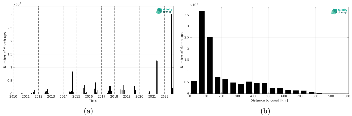
Figure 2: Number of match-ups between TSG (Polarstern) and SMOS SSS L2 v700 (ESA) SSS as a function of time (a) and as function of the distance to coast (b) over the Arctic Ocean Pi-MEP region and for the full satellite product period.
