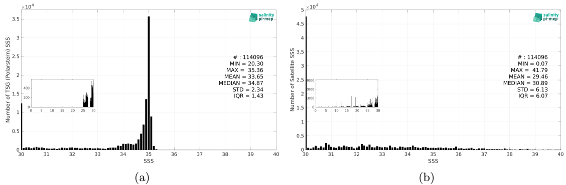
Figure 3: Histograms of SSS from TSG (Polarstern) (a) and SMOS SSS L2 v700 (ESA) (b) considering all match-up pairs per bins of 0.1 over the Arctic Ocean Pi-MEP region and for the full satellite product period.
