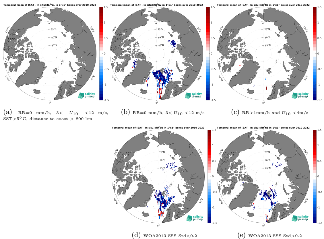
Figure 14: Temporal mean gridded over spatial boxes of size 1^\circ \times 1^\circ of \Delta SSS (SMOS SSS L2 v700 (ESA) - TSG (Polarstern)) for 5 different subdatasets corresponding to:RR=0 mm/h, 3 < U_{10} < 12 m/s, SST > 5^\circ\text{C} , distance to coast > 800 km (a), RR=0 mm/h, 3 < U_{10} < 12 m/s (b), RR > 1 mm/h and U_{10} < 4 m/s (c), WOA2013 SSS Std < 0.2 (d), WOA2013 SSS Std > 0.2 (e).
