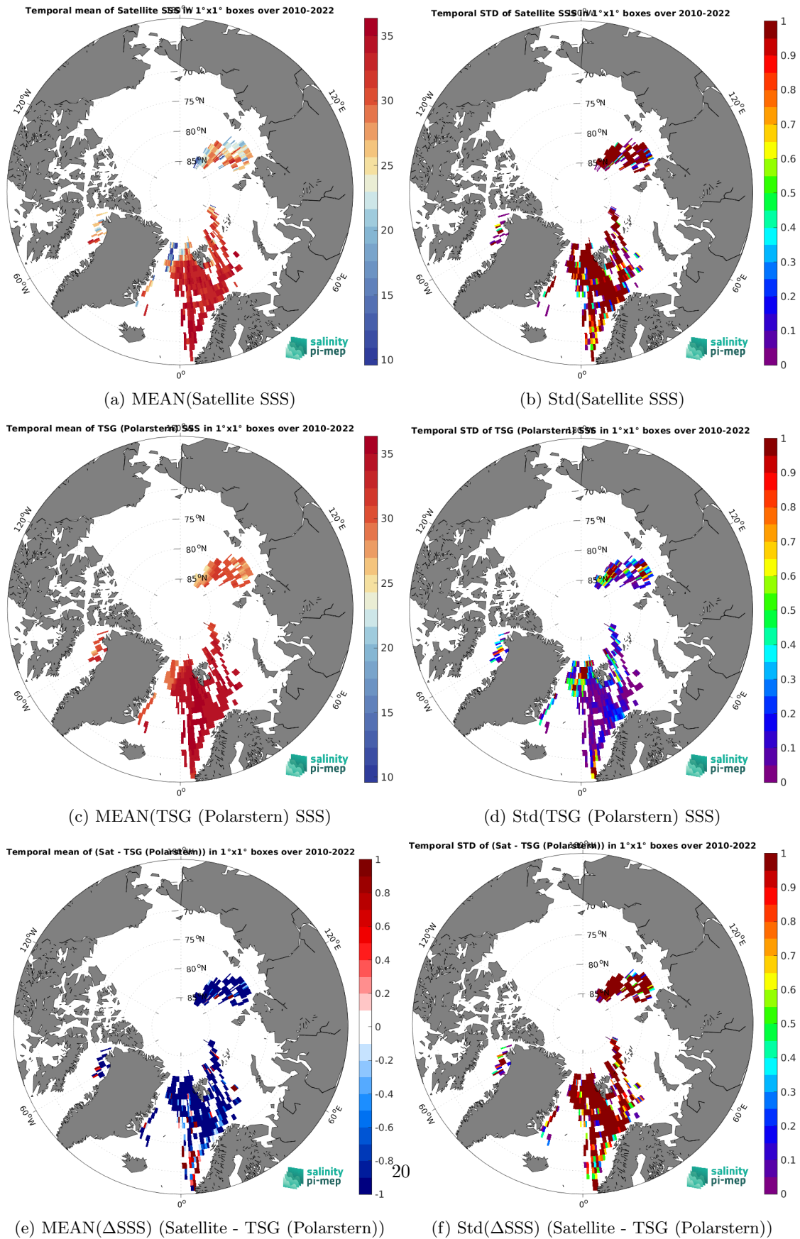
Figure 7: Temporal mean (left) and Std (right) of SSS from SMOS SSS L2 v700 (ESA) (top), TSG (Polarstern) (middle), and of \Delta SSS (Satellite - TSG (Polarstern)). Only match-up pairs are used to generate these maps.
