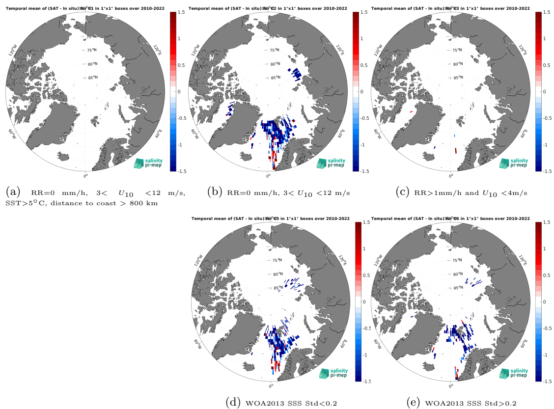
Figure 14: Temporal mean gridded over spatial boxes of size 1^\circ \times 1^\circ of \Delta\text{SSS} (SMOS SSS L2 v700 (ESA) - TSG (Polarstern)) for 5 different subdatasets corresponding to:RR=0 mm/h, 3 < U_{10} < 12 m/s, SST > 5°C, distance to coast > 800 km (a), RR=0 mm/h, 3 < U_{10} < 12 m/s (b), RR > 1mm/h and U_{10} < 4 m/s (c), WOA2013 SSS Std < 0.2 (d), WOA2013 SSS Std > 0.2 (e).
