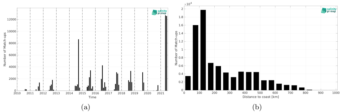
Figure 1: Number of match-ups between TSG (Polarstern) and SMOS SSS L2 v700 (ESA) SSS as a function of time (a) and as function of the distance to coast (b) over the Arctic Ocean Pi-MEP region and for the full satellite product period.
